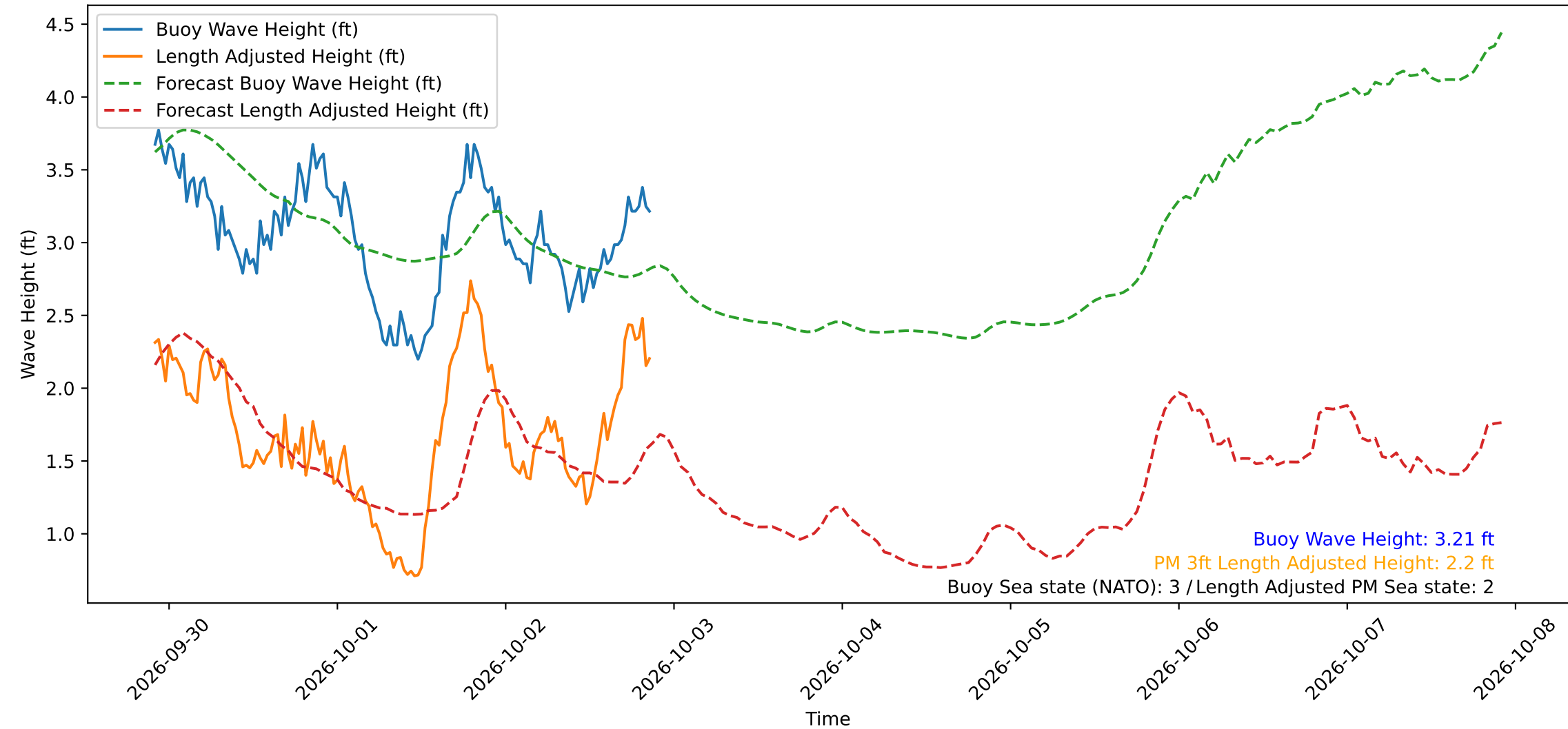
Wave Heights over Time for Green Beach at 2026-10-02 21:31:12
