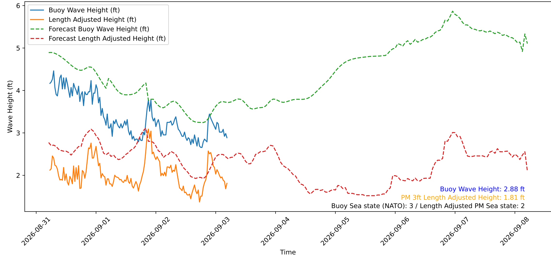
Wave Heights over Time for Green Beach at 2026-09-03 05:11:13
