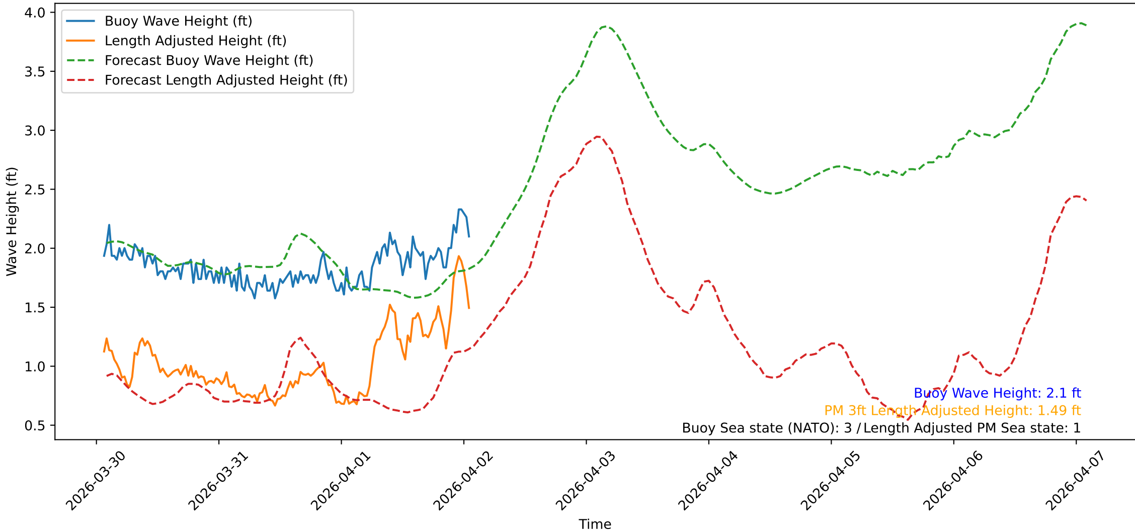
Wave Heights over Time for Oceanside Harbor at 2026-04-02 01:40:31
