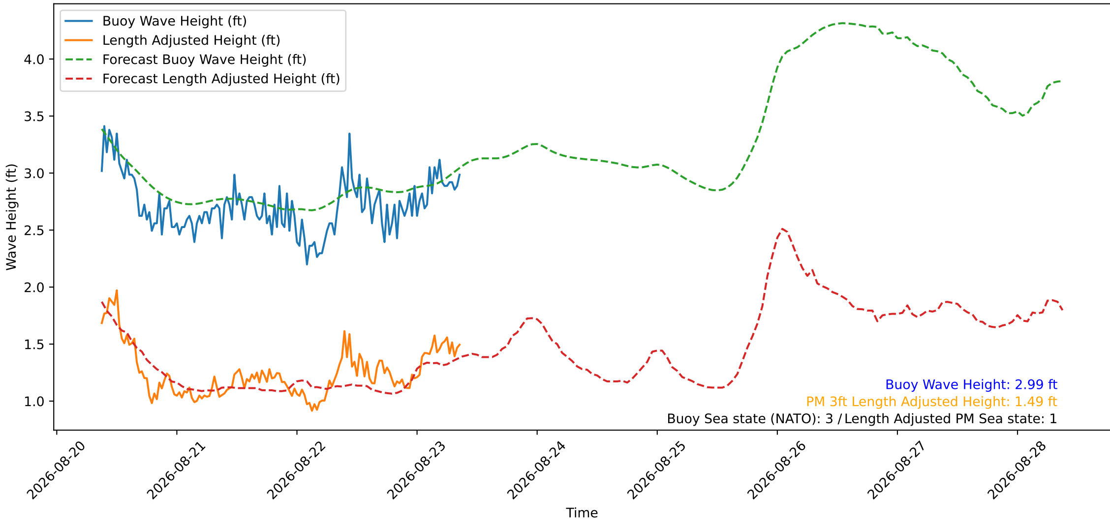
Wave Heights over Time for Oceanside Harbor at 2026-08-23 09:00:29
