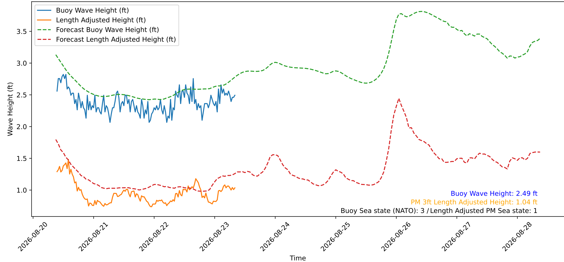
Wave Heights over Time for Red Beach at 2026-08-23 09:00:49
