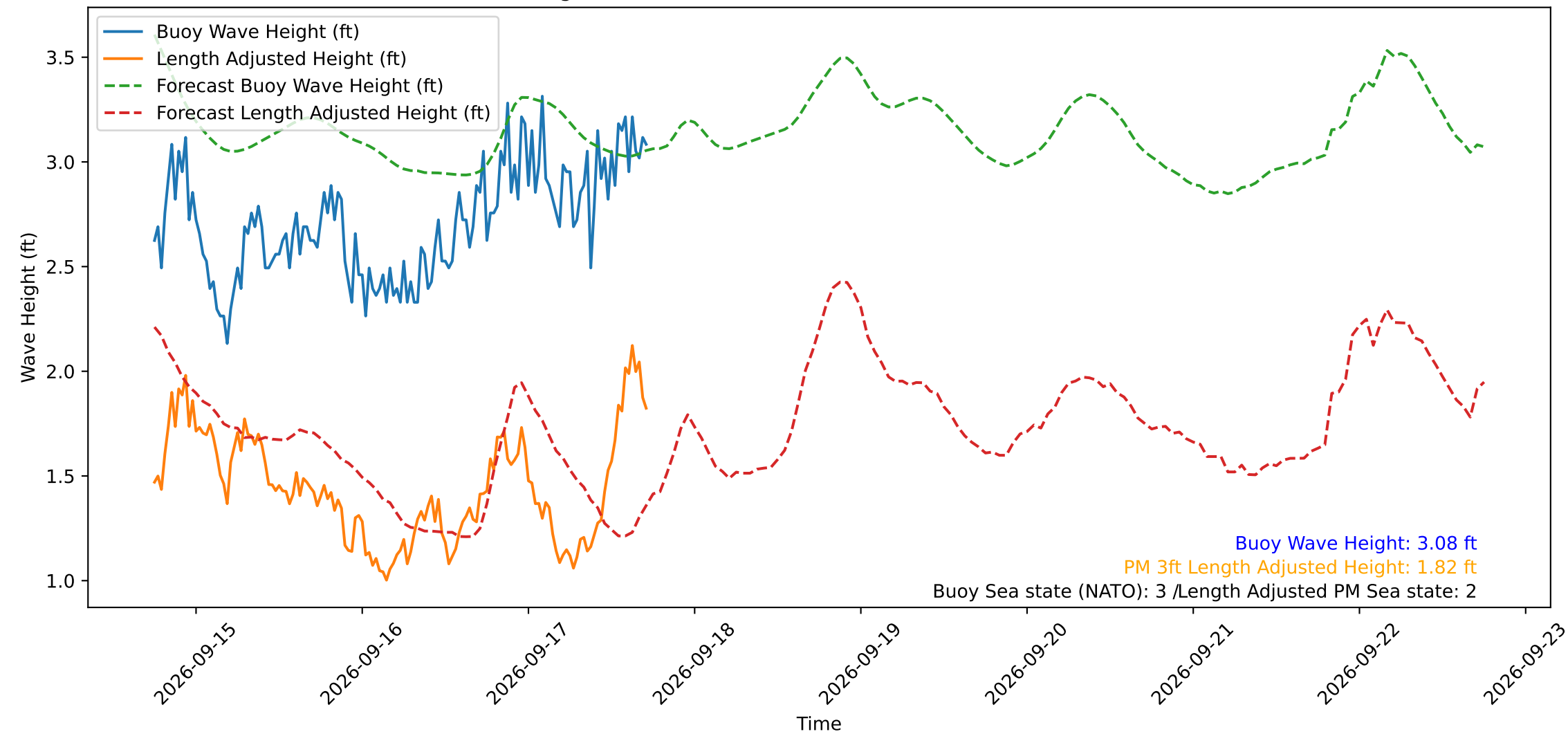
Wave Heights over Time for Green Beach at 2026-09-17 17:41:11
