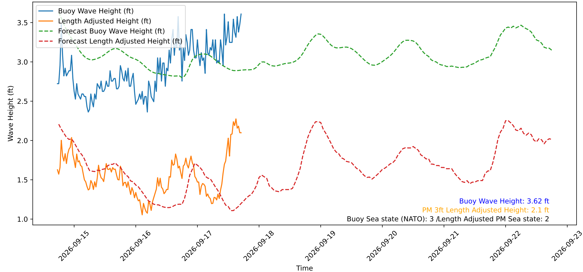
Wave Heights over Time for Oceanside Harbor at 2026-09-17 17:40:29
