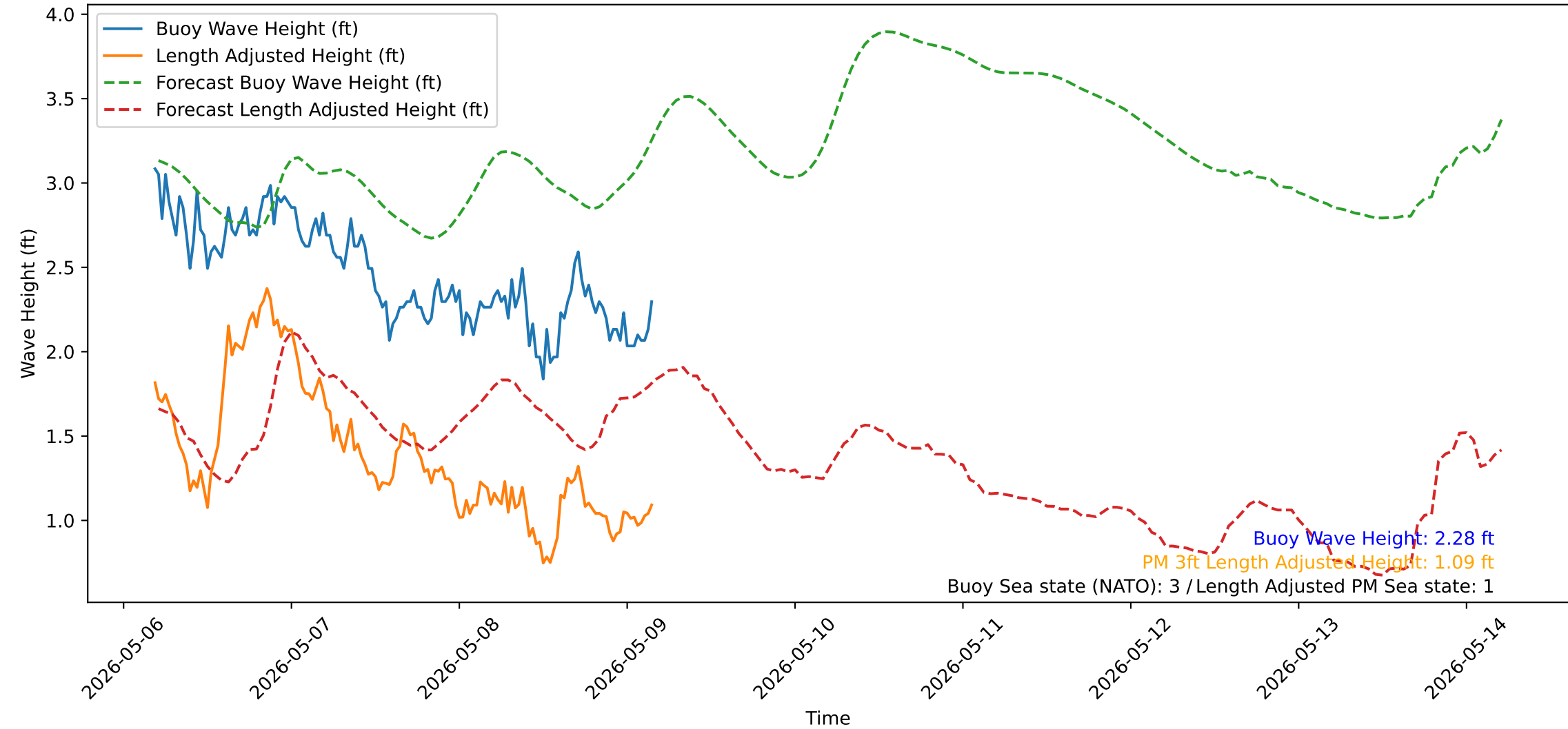
Wave Heights over Time for Green Beach at 2026-05-09 04:31:15
