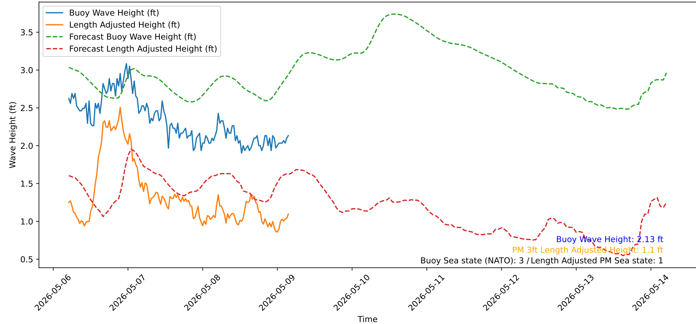
Wave Heights over Time for Red Beach at 2026-05-09 04:30:51
