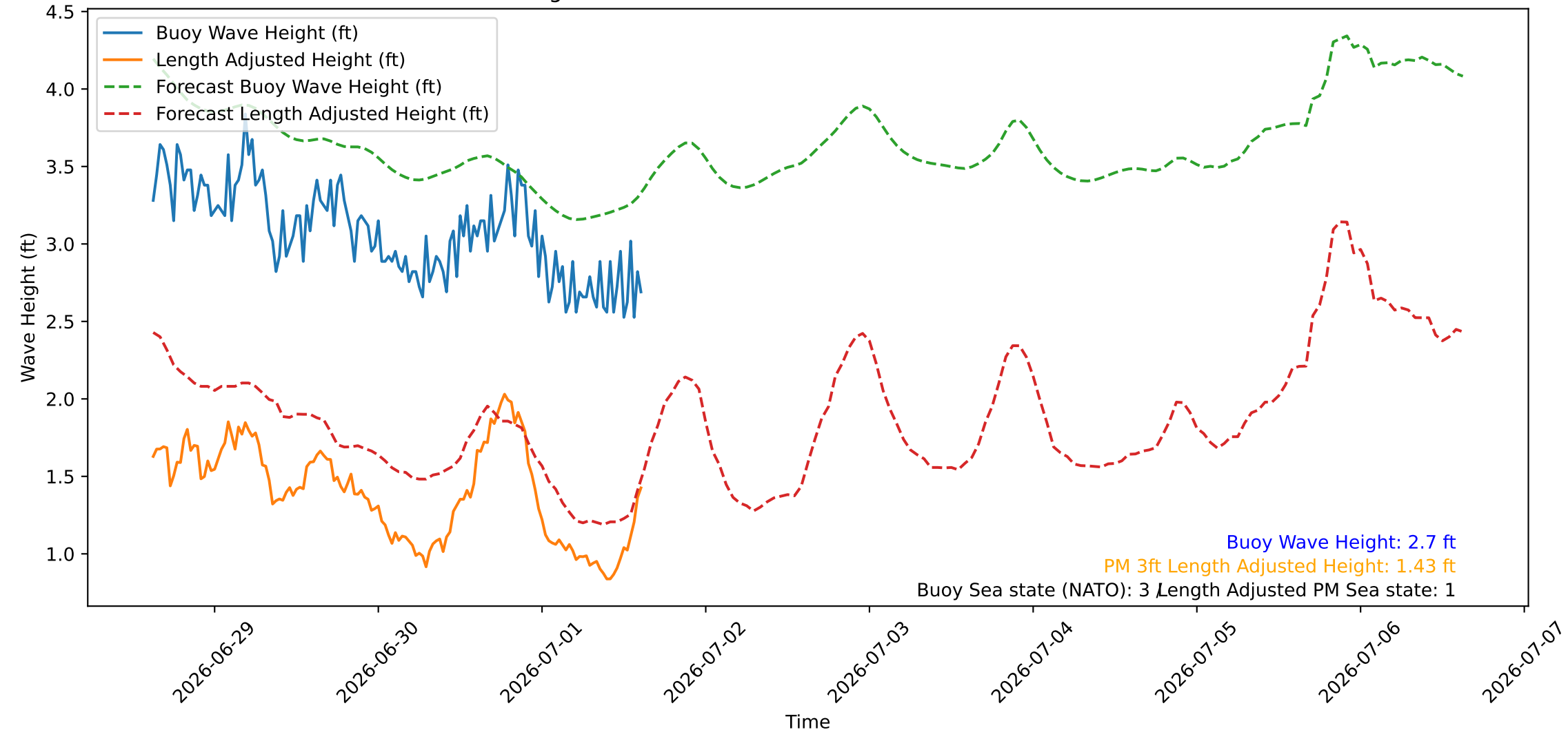
Wave Heights over Time for Green Beach at 2026-07-01 15:11:08
