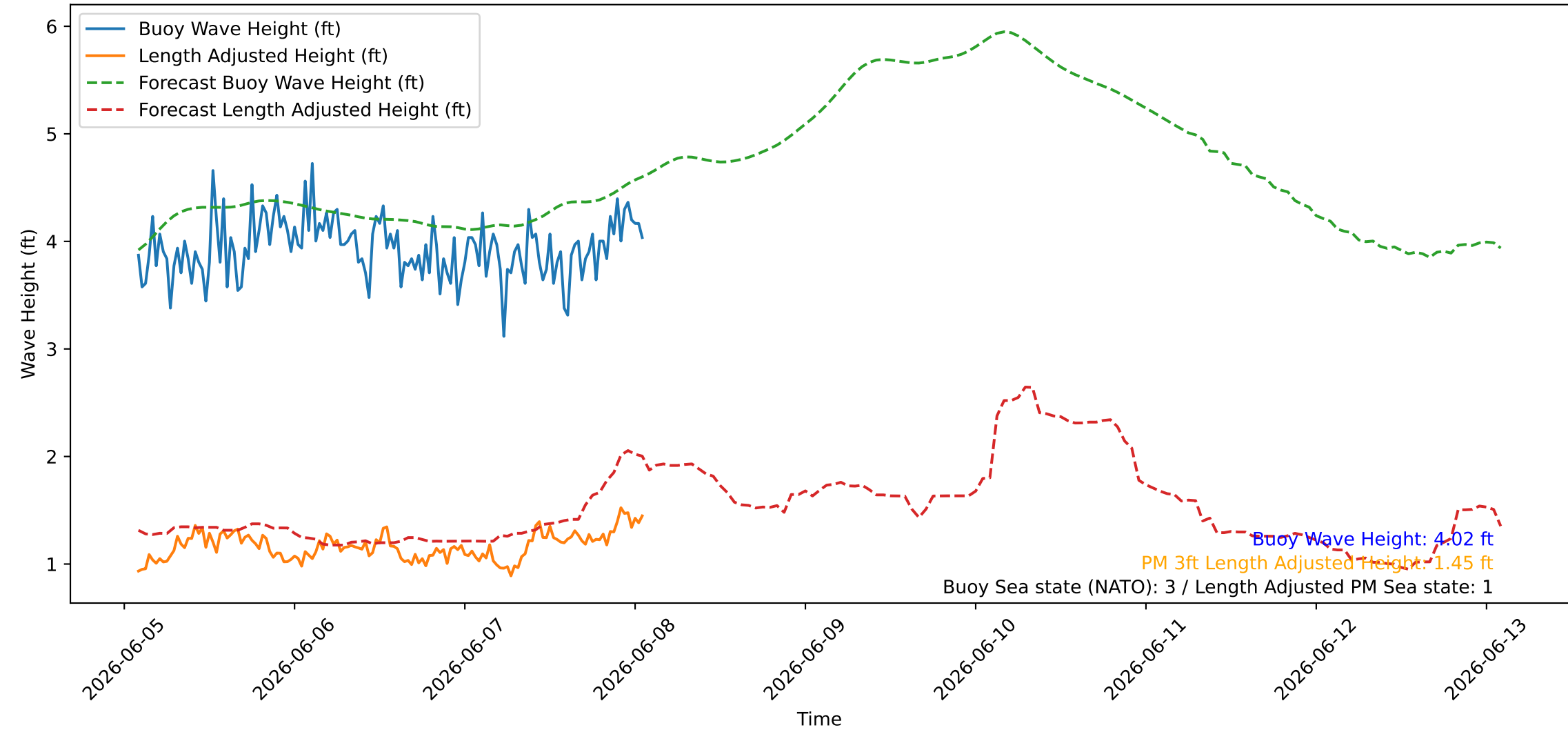
Wave Heights over Time for Green Beach at 2026-06-08 01:51:09
