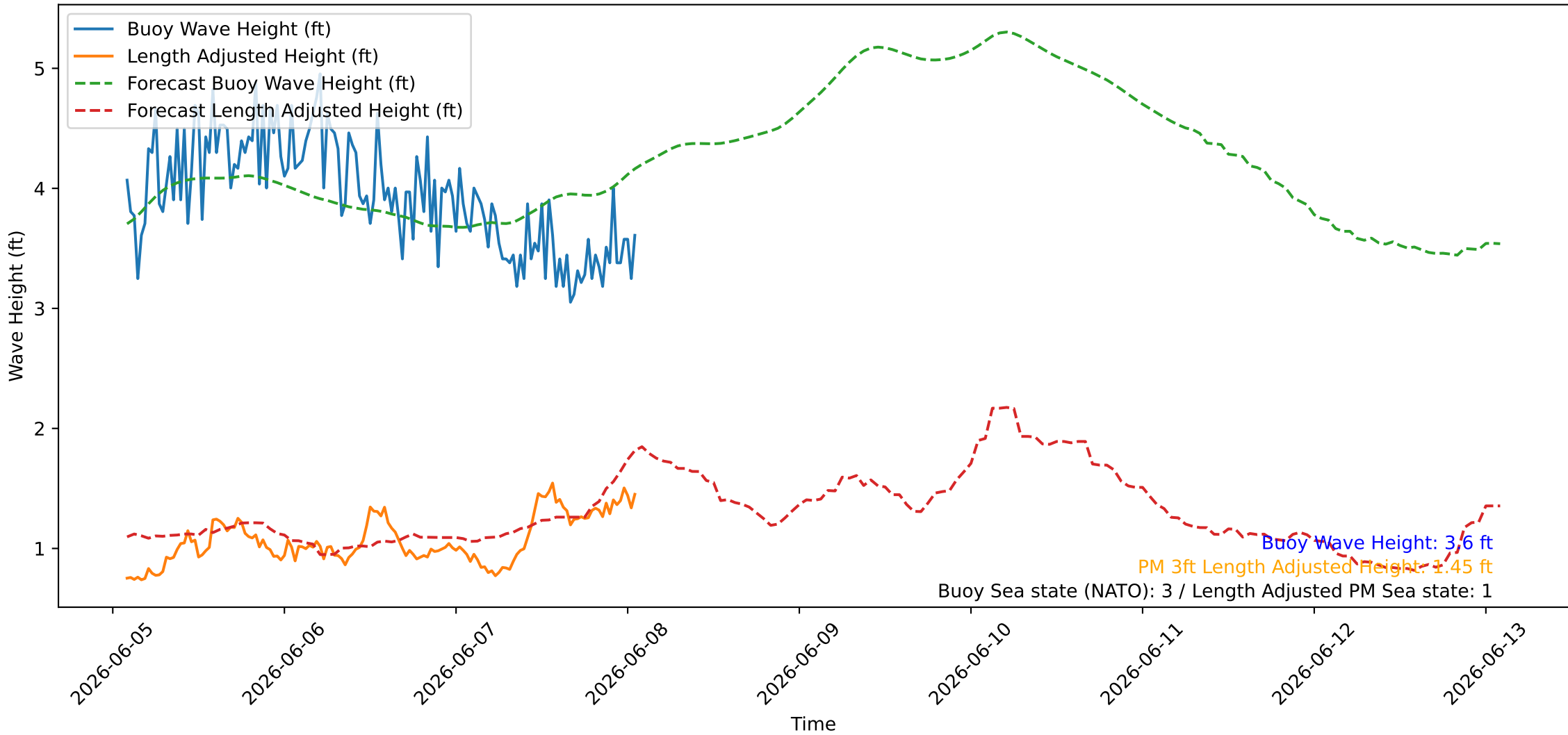
Wave Heights over Time for Red Beach at 2026-06-08 01:50:47
