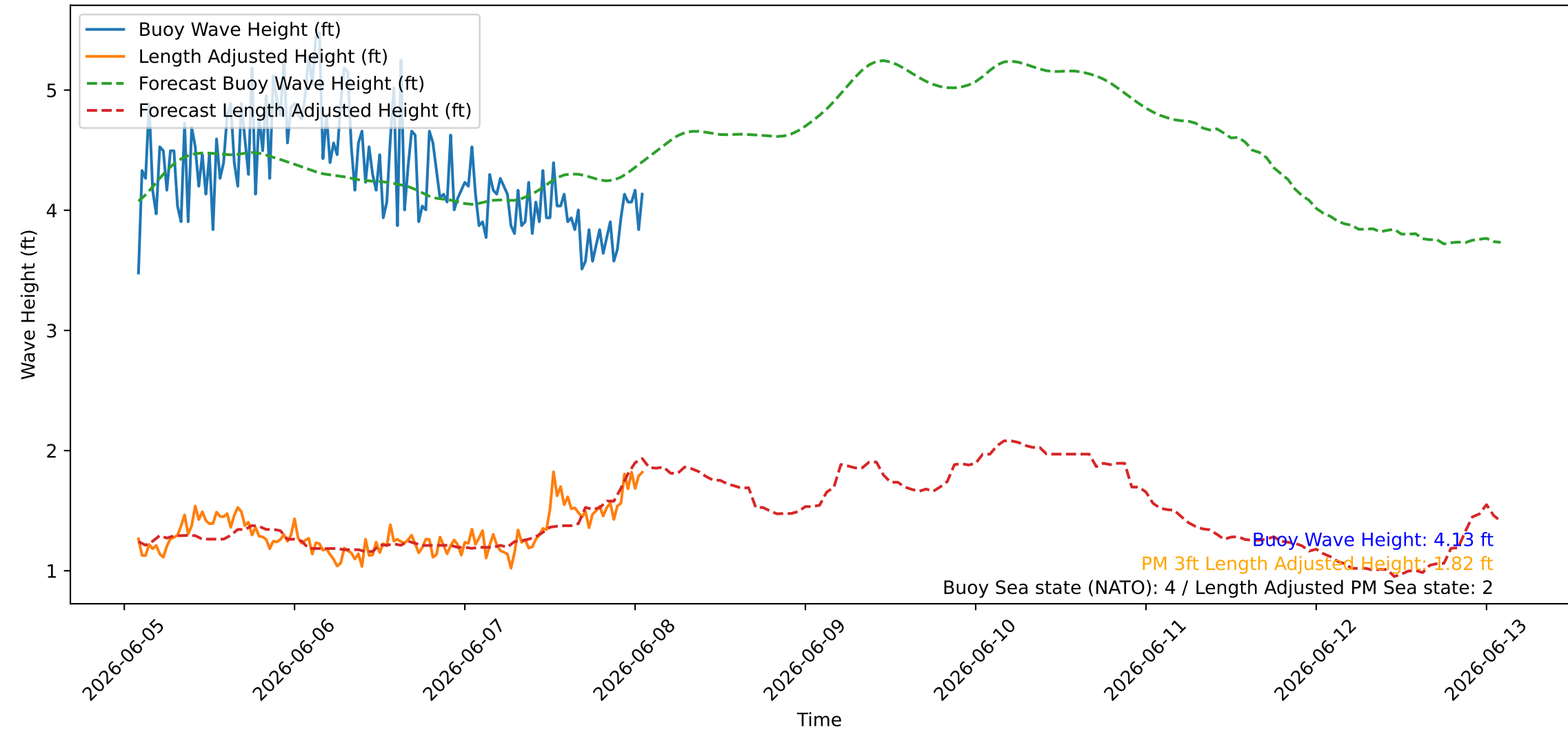
Wave Heights over Time for Oceanside Harbor at 2026-06-08 01:50:26
