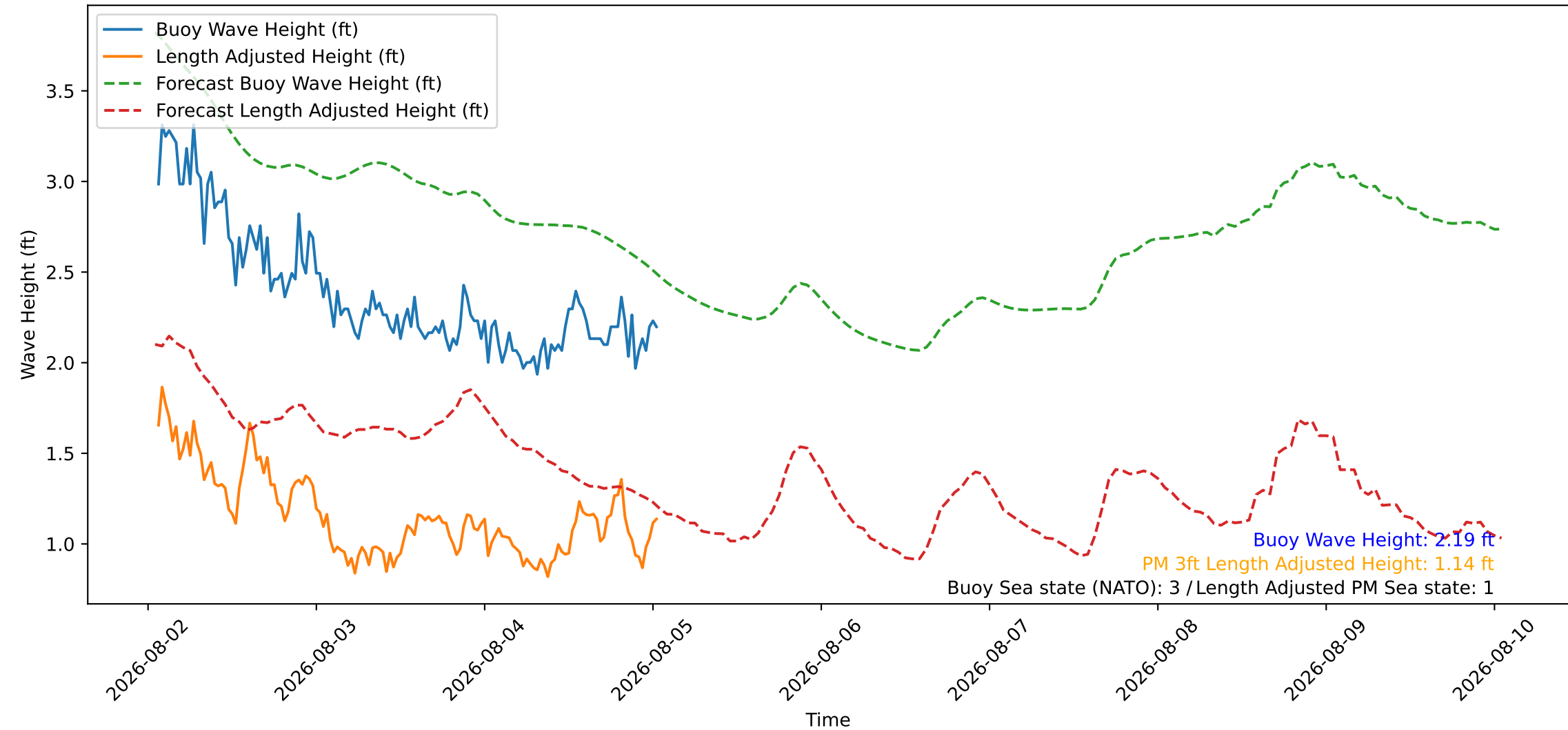
Wave Heights over Time for Green Beach at 2026-08-05 01:21:11
