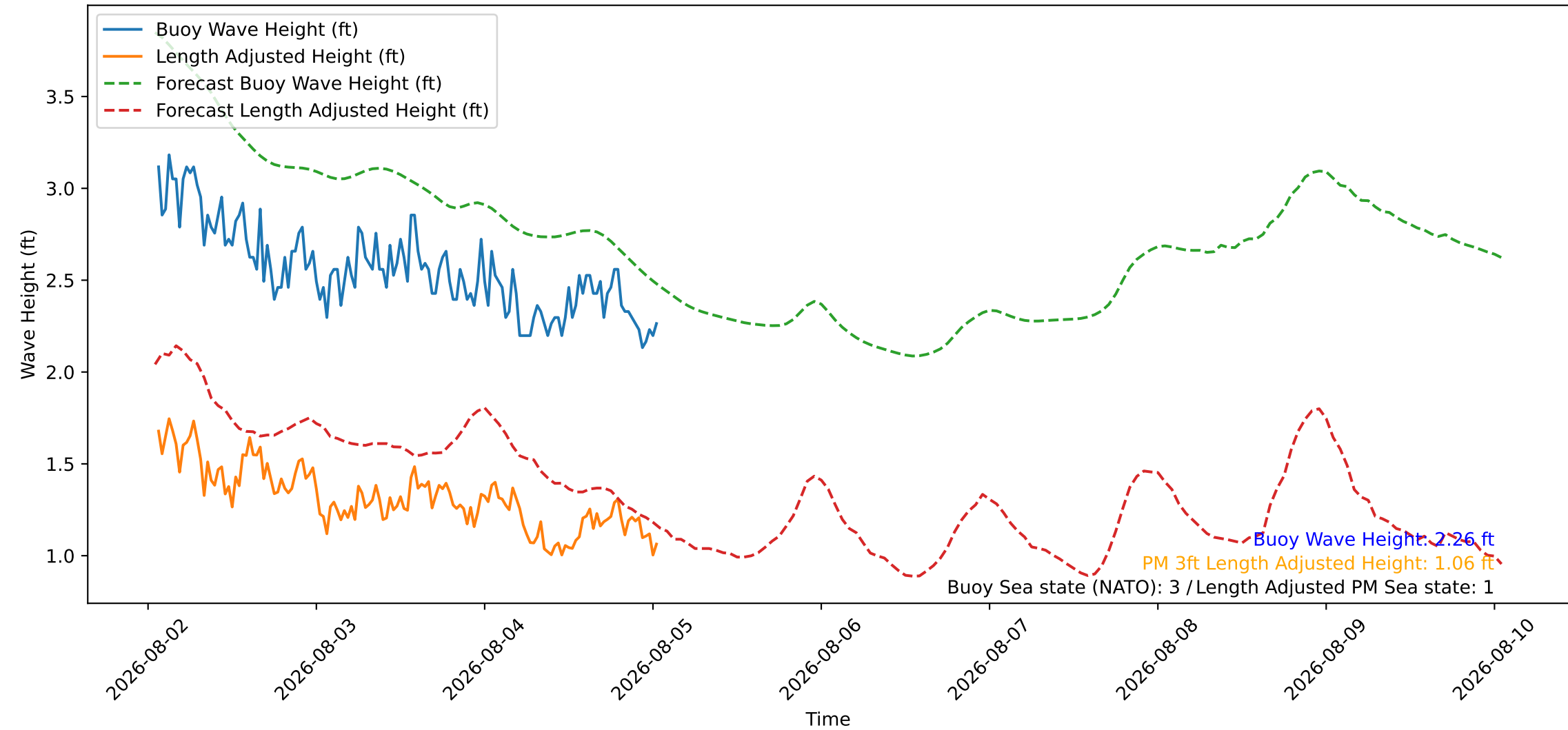
Wave Heights over Time for Oceanside Harbor at 2026-08-05 01:20:27
