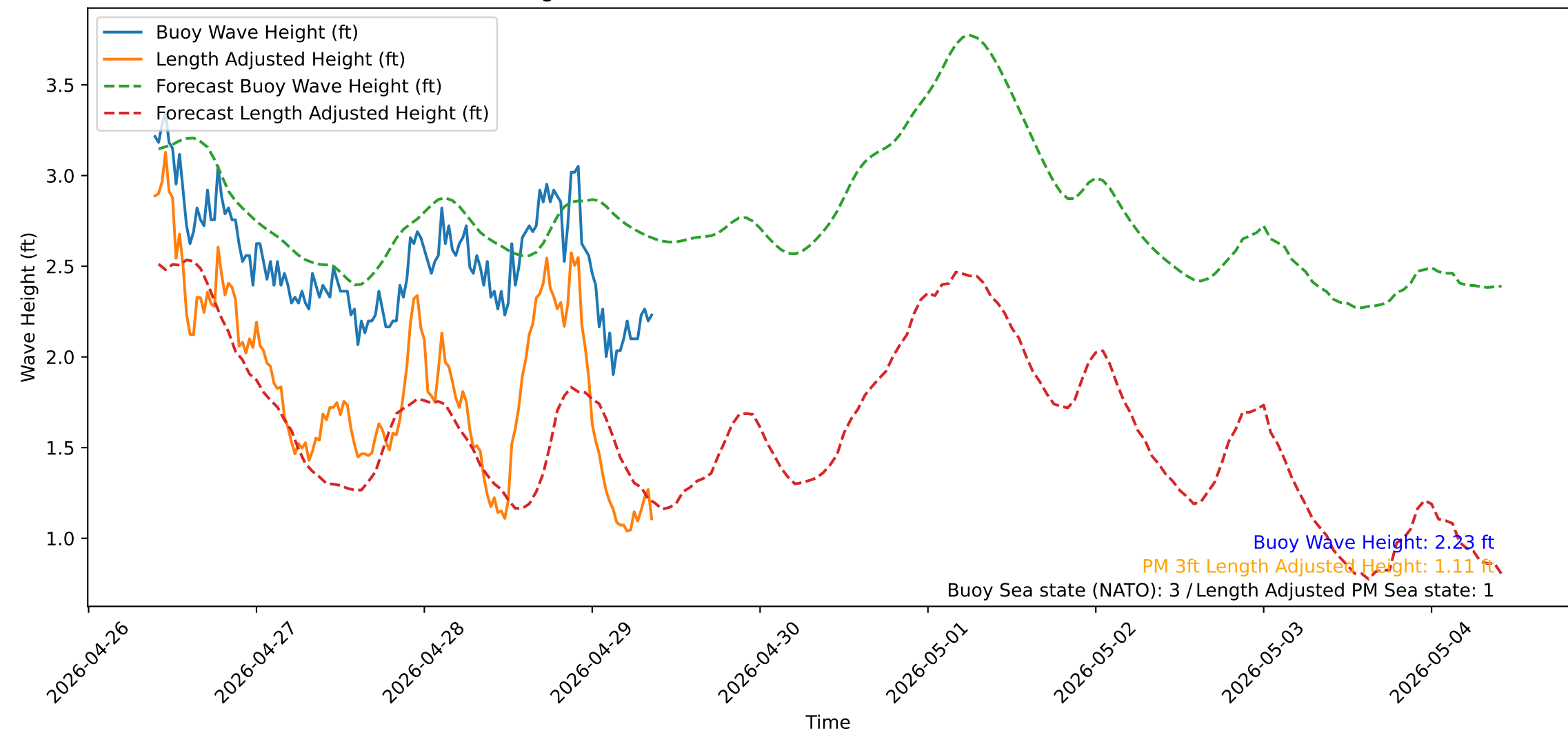
Wave Heights over Time for Oceanside Harbor at 2026-04-29 09:30:32
