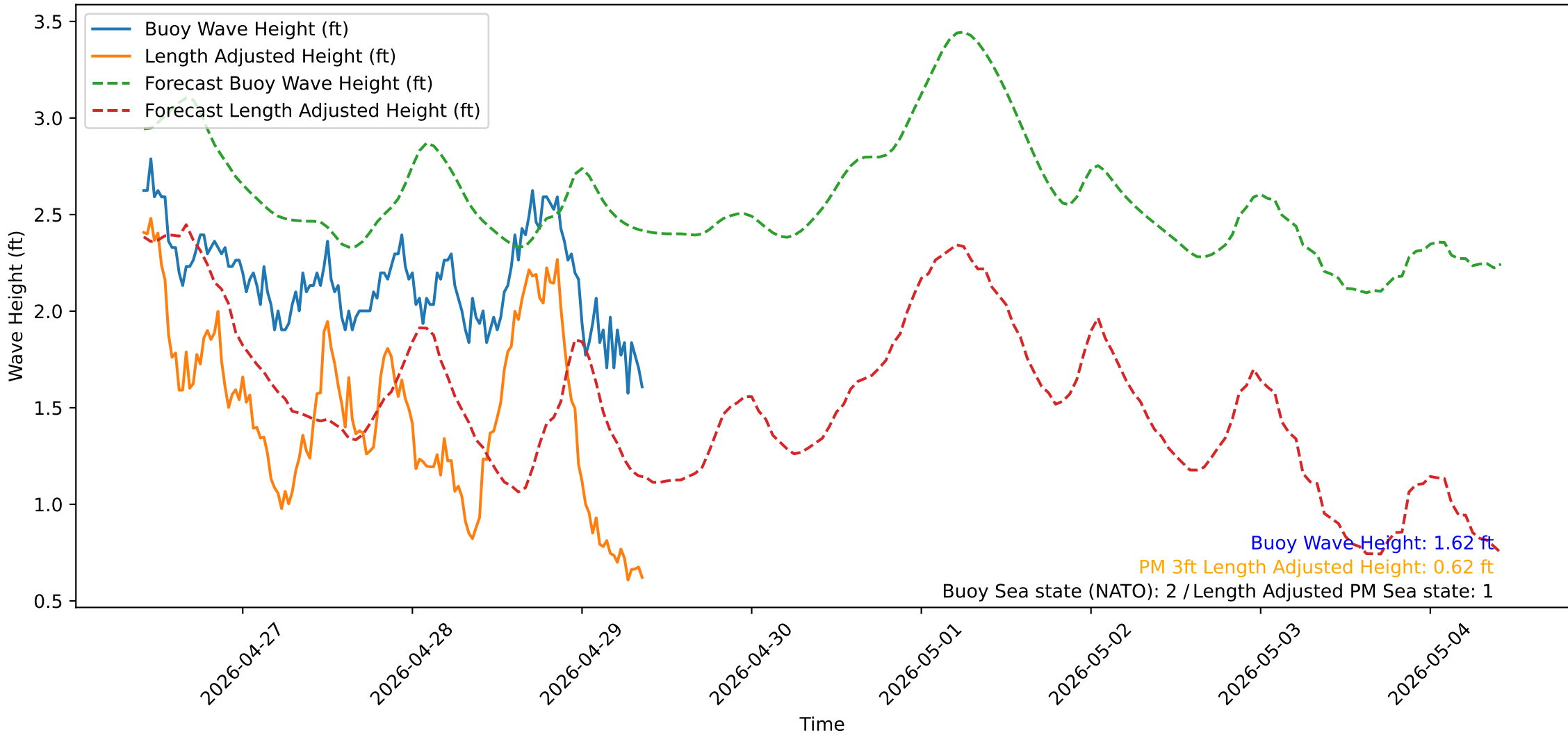
Wave Heights over Time for Red Beach at 2026-04-29 09:30:51
