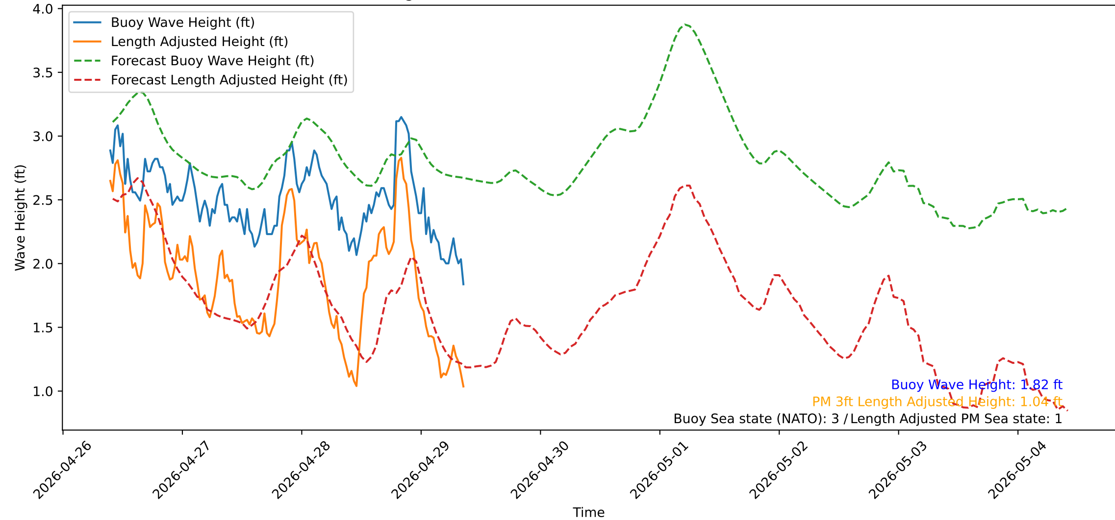
Wave Heights over Time for Green Beach at 2026-04-29 09:31:14
