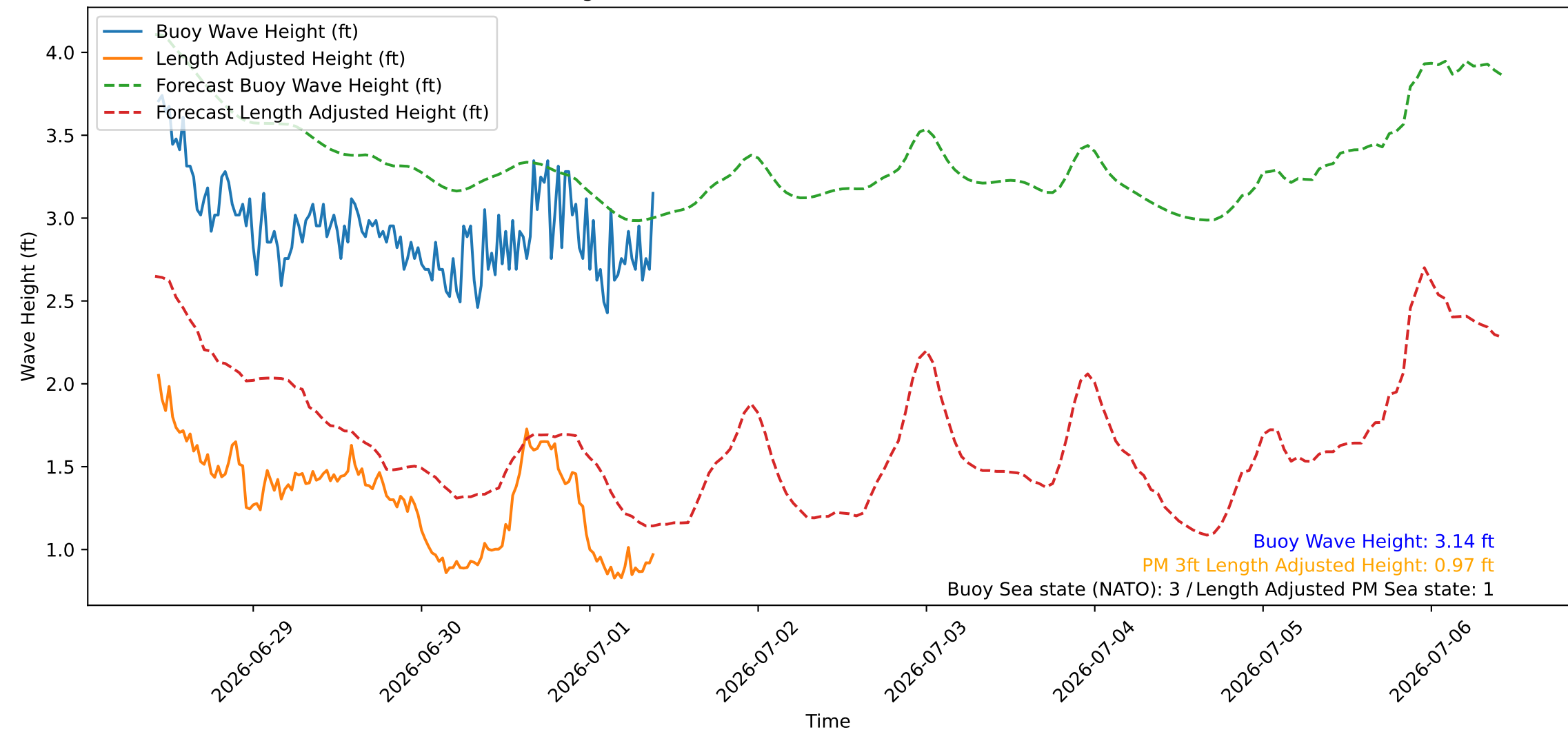
Wave Heights over Time for Red Beach at 2026-07-01 10:10:46
