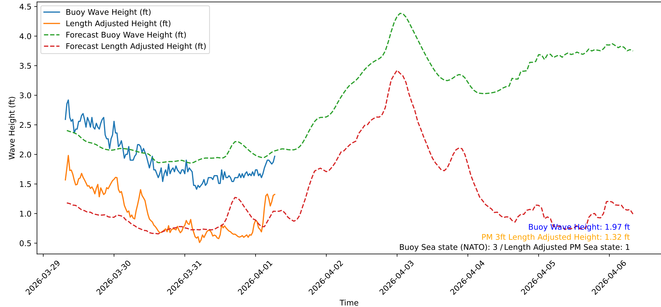
Wave Heights over Time for Green Beach at 2026-04-01 07:31:10
