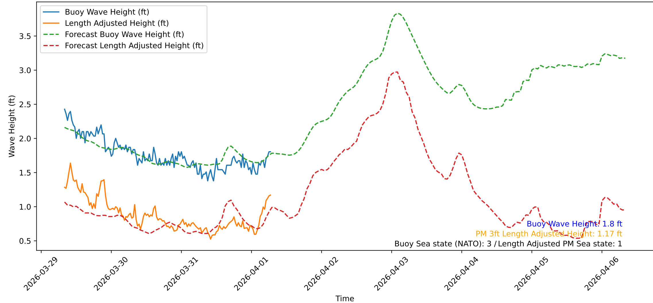
Wave Heights over Time for Red Beach at 2026-04-01 07:30:48
