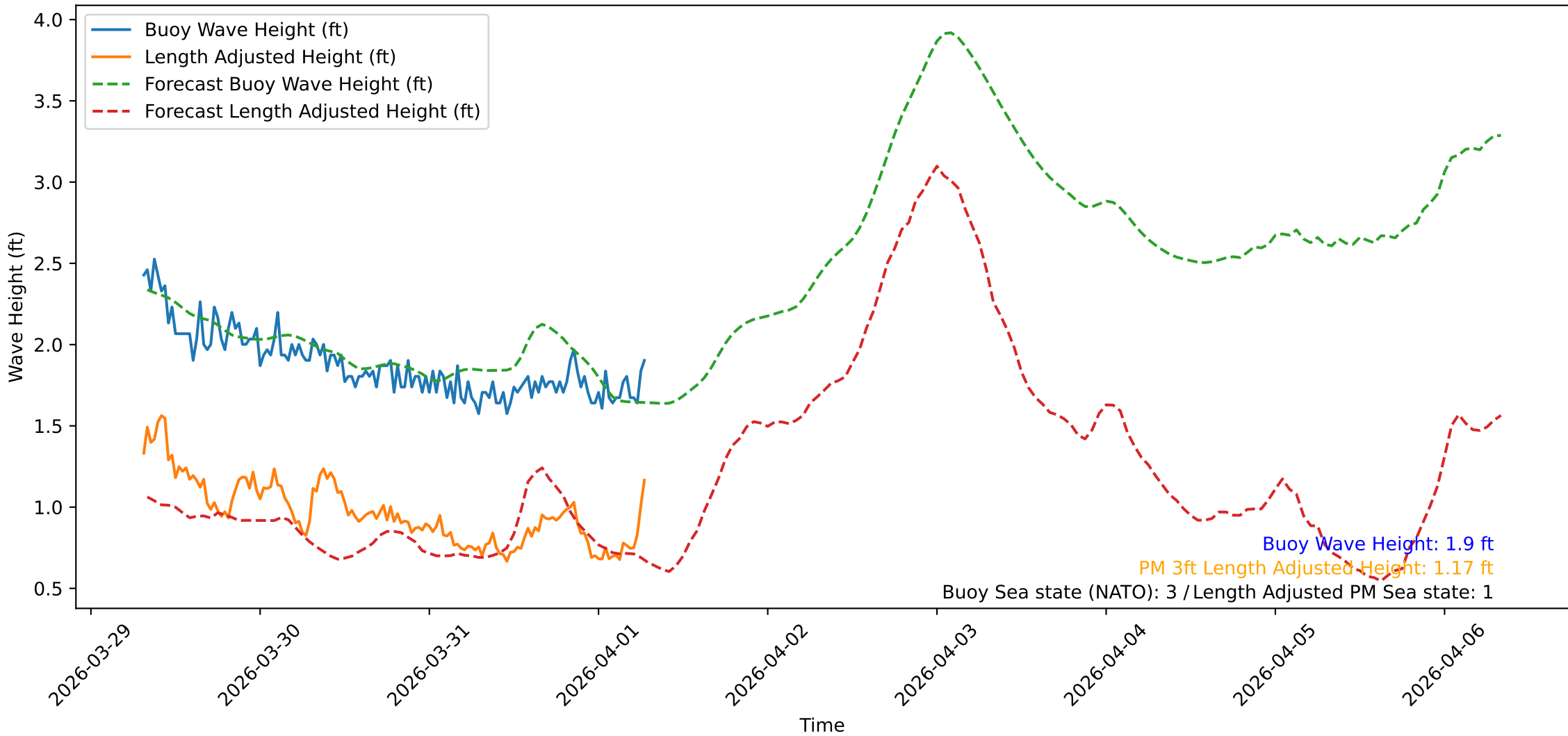
Wave Heights over Time for Oceanside Harbor at 2026-04-01 07:30:31
