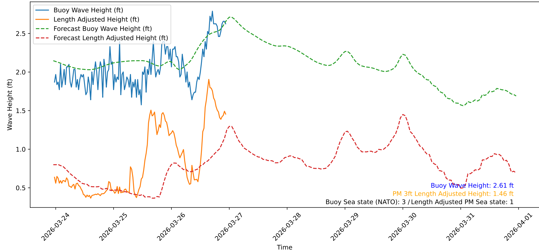
Wave Heights over Time for Red Beach at 2026-03-26 23:20:46
