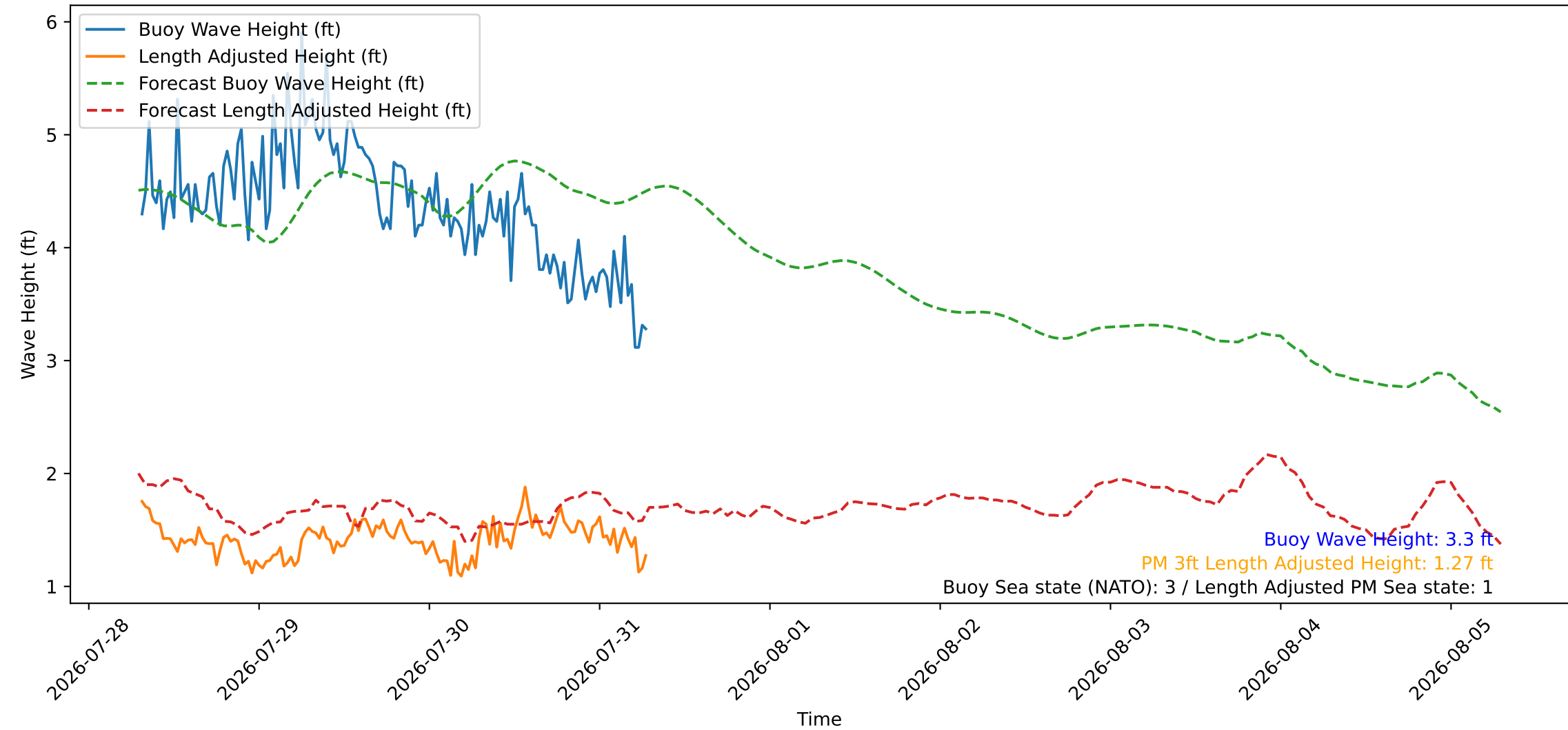
Wave Heights over Time for Oceanside Harbor at 2026-07-31 07:20:26
