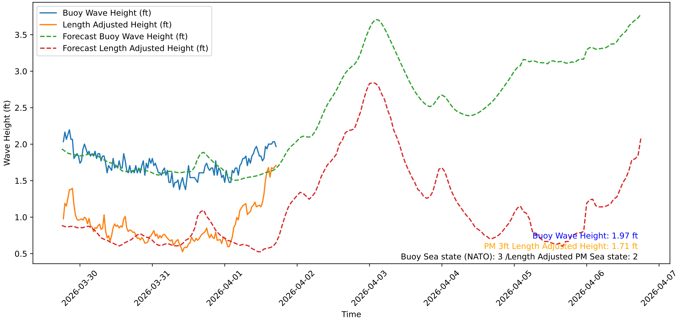
Wave Heights over Time for Red Beach at 2026-04-01 18:00:47
