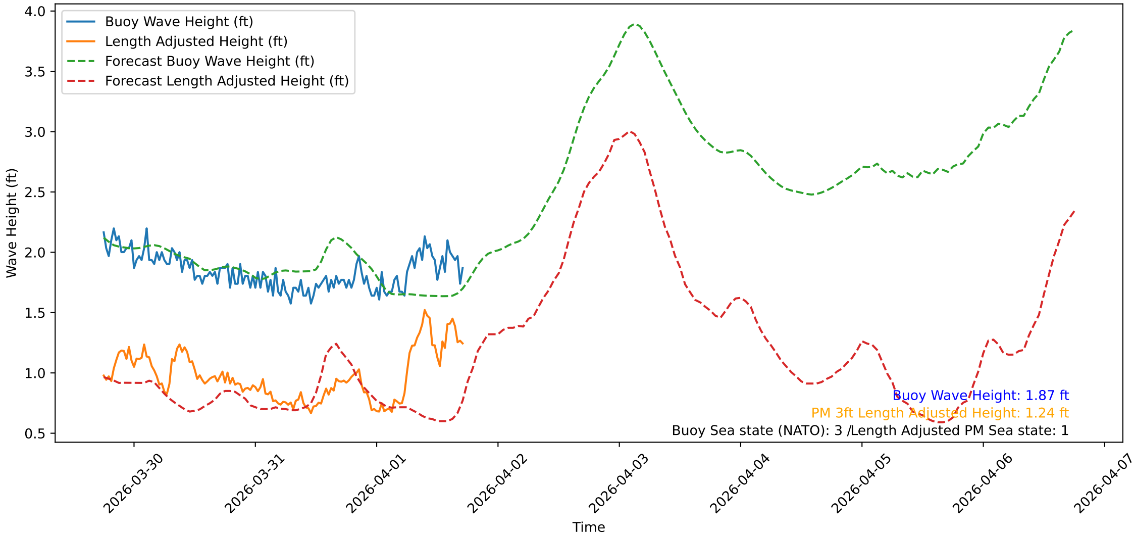
Wave Heights over Time for Oceanside Harbor at 2026-04-01 18:00:32
