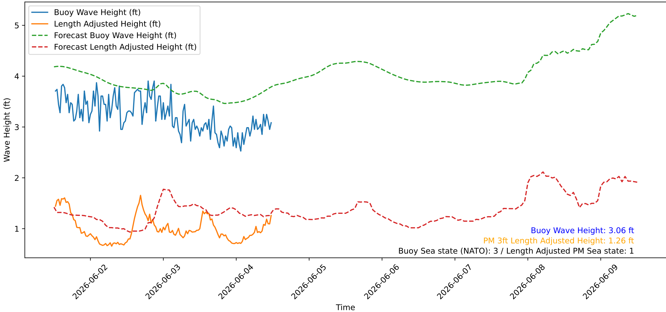
Wave Heights over Time for Red Beach at 2026-06-04 12:20:48
