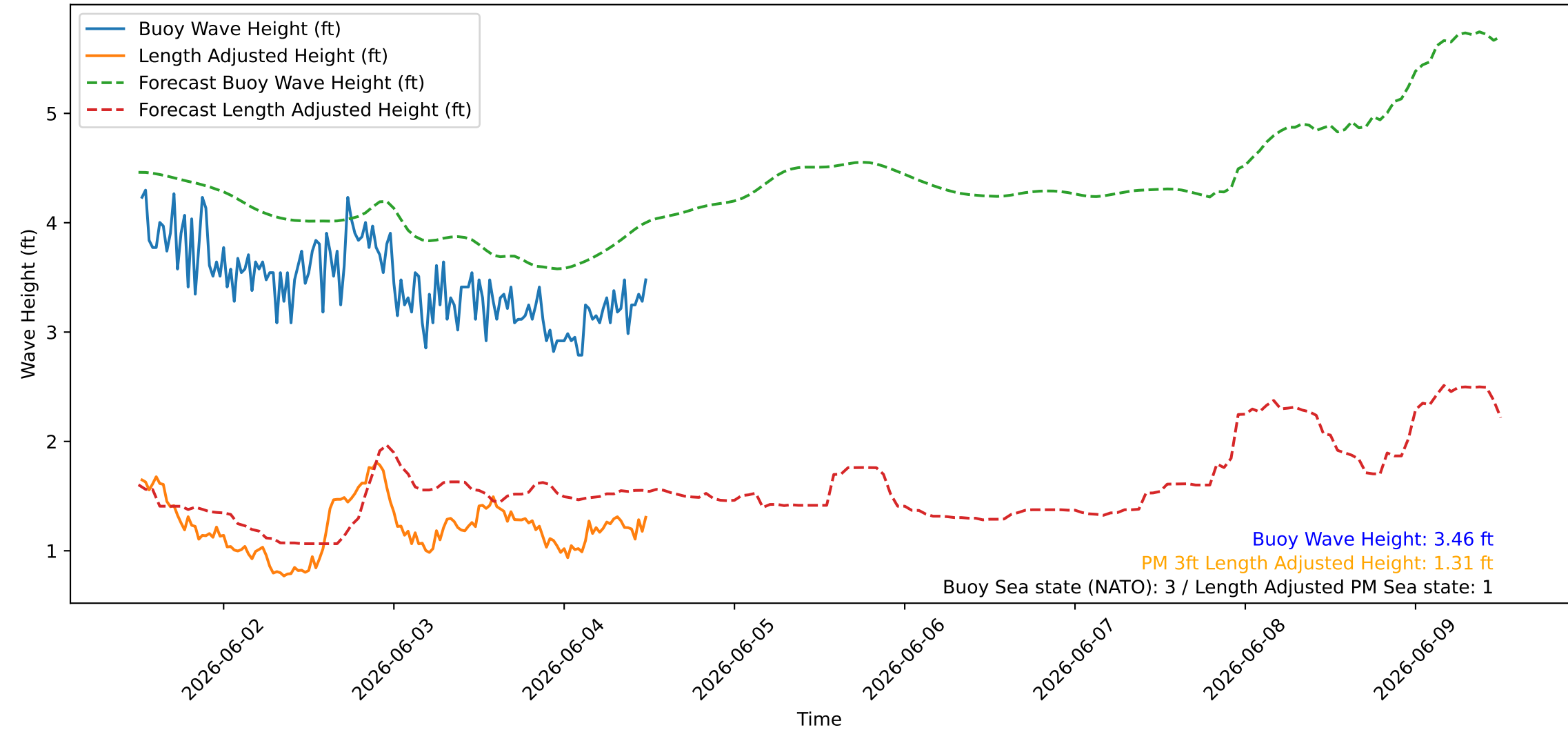
Wave Heights over Time for Green Beach at 2026-06-04 12:21:10
