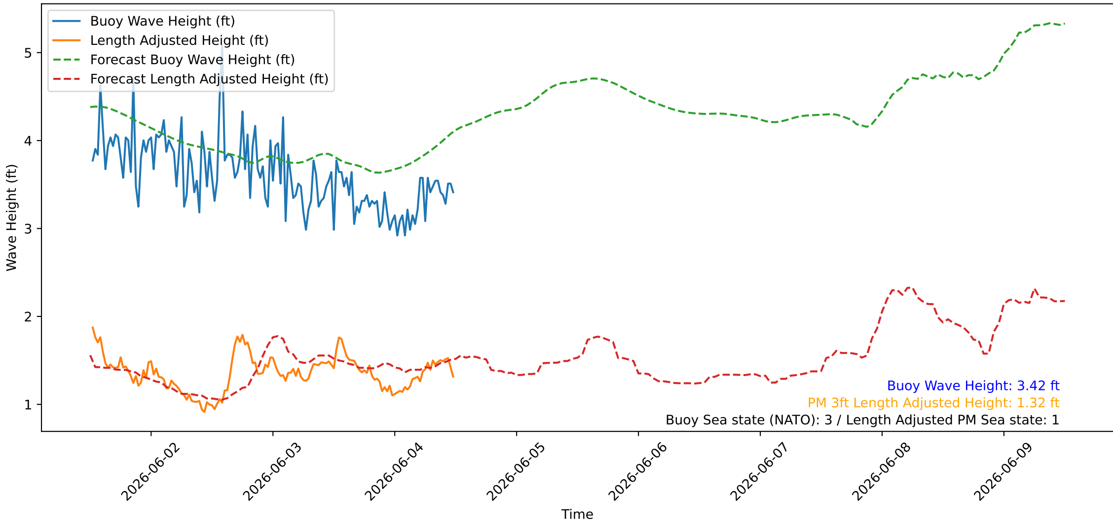
Wave Heights over Time for Oceanside Harbor at 2026-06-04 12:20:27
