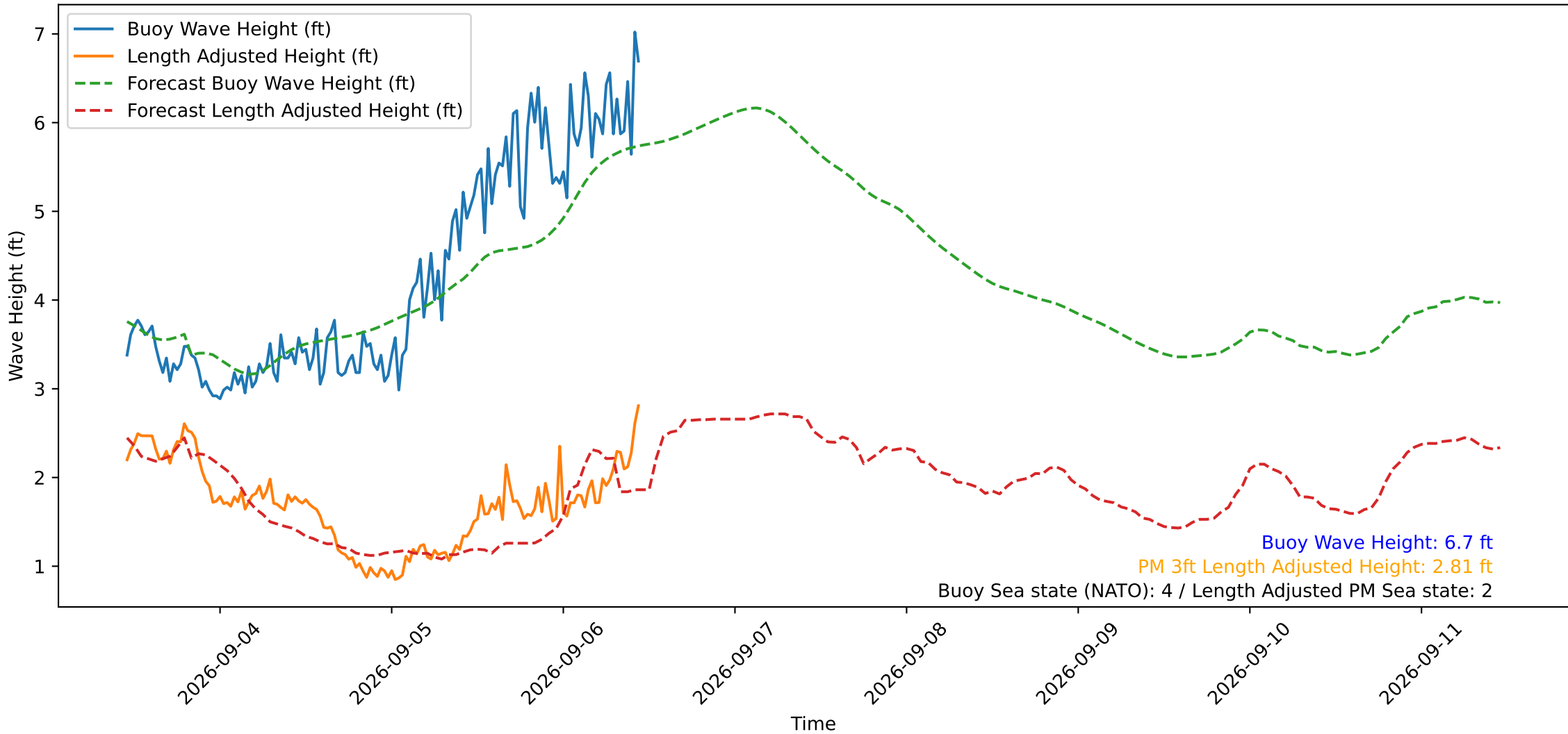
Wave Heights over Time for Oceanside Harbor at 2026-09-06 11:00:30
