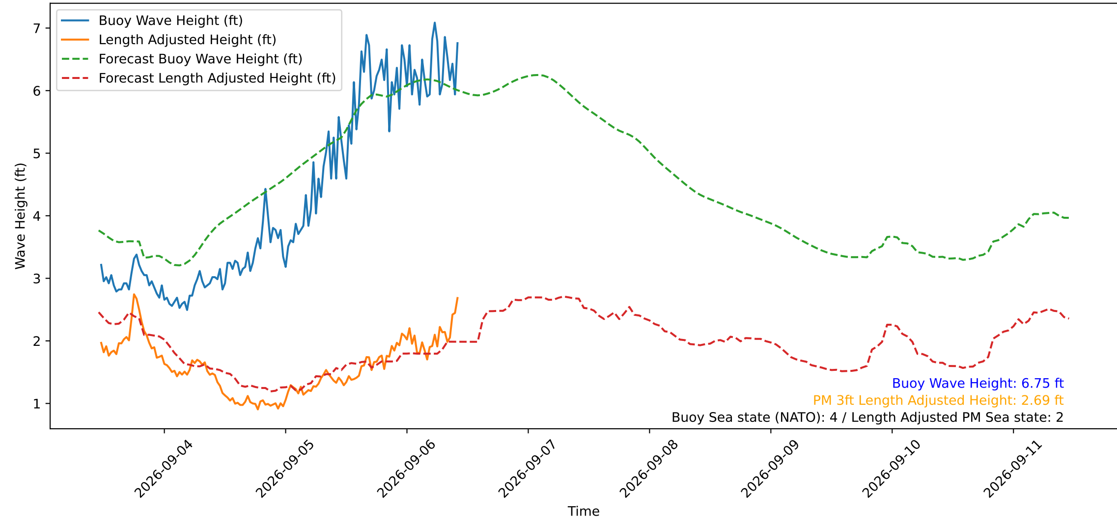
Wave Heights over Time for Green Beach at 2026-09-06 11:01:12
