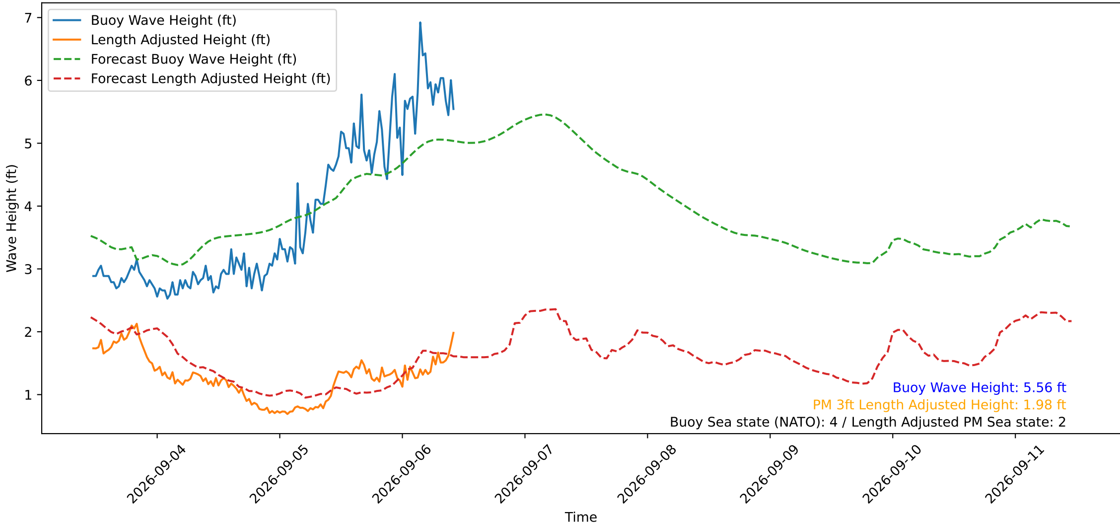
Wave Heights over Time for Red Beach at 2026-09-06 11:00:50
