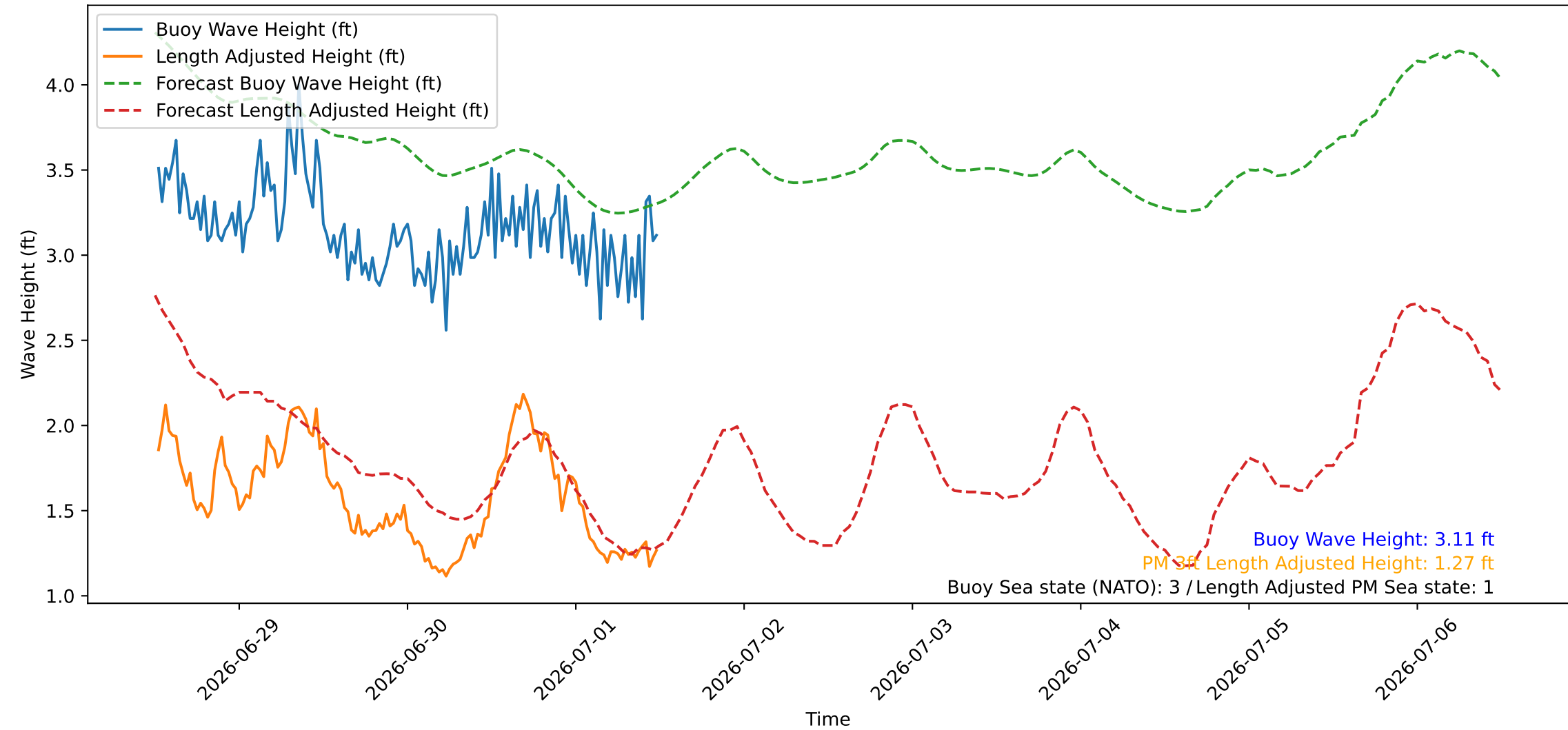
Wave Heights over Time for Oceanside Harbor at 2026-07-01 12:20:26
