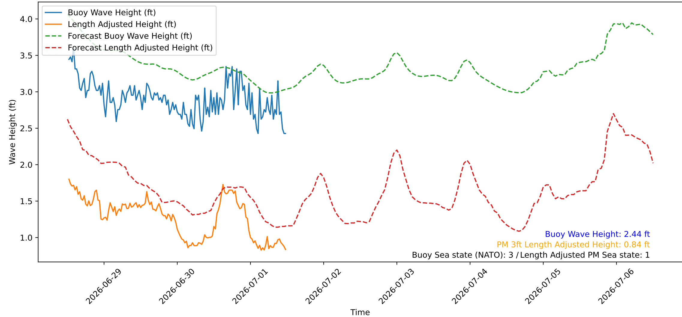
Wave Heights over Time for Red Beach at 2026-07-01 12:20:47
