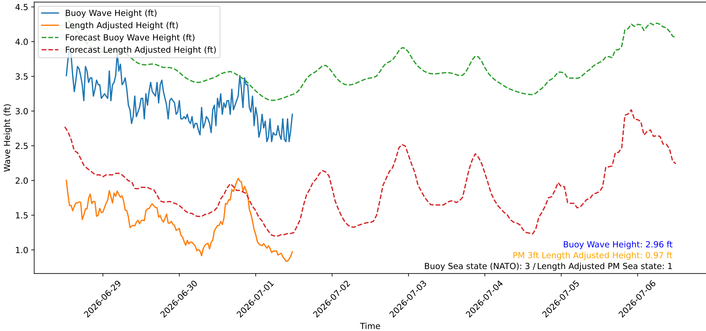
Wave Heights over Time for Green Beach at 2026-07-01 12:21:09
