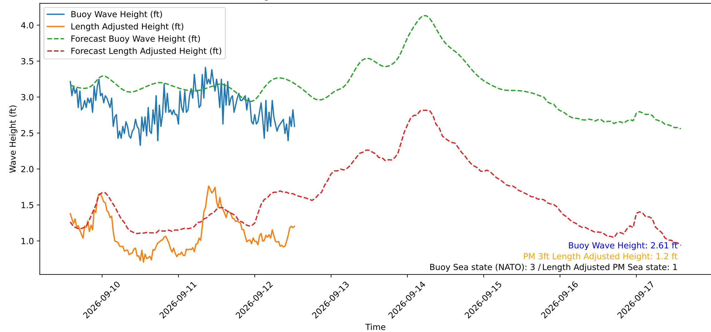
Wave Heights over Time for Red Beach at 2026-09-12 13:30:49
