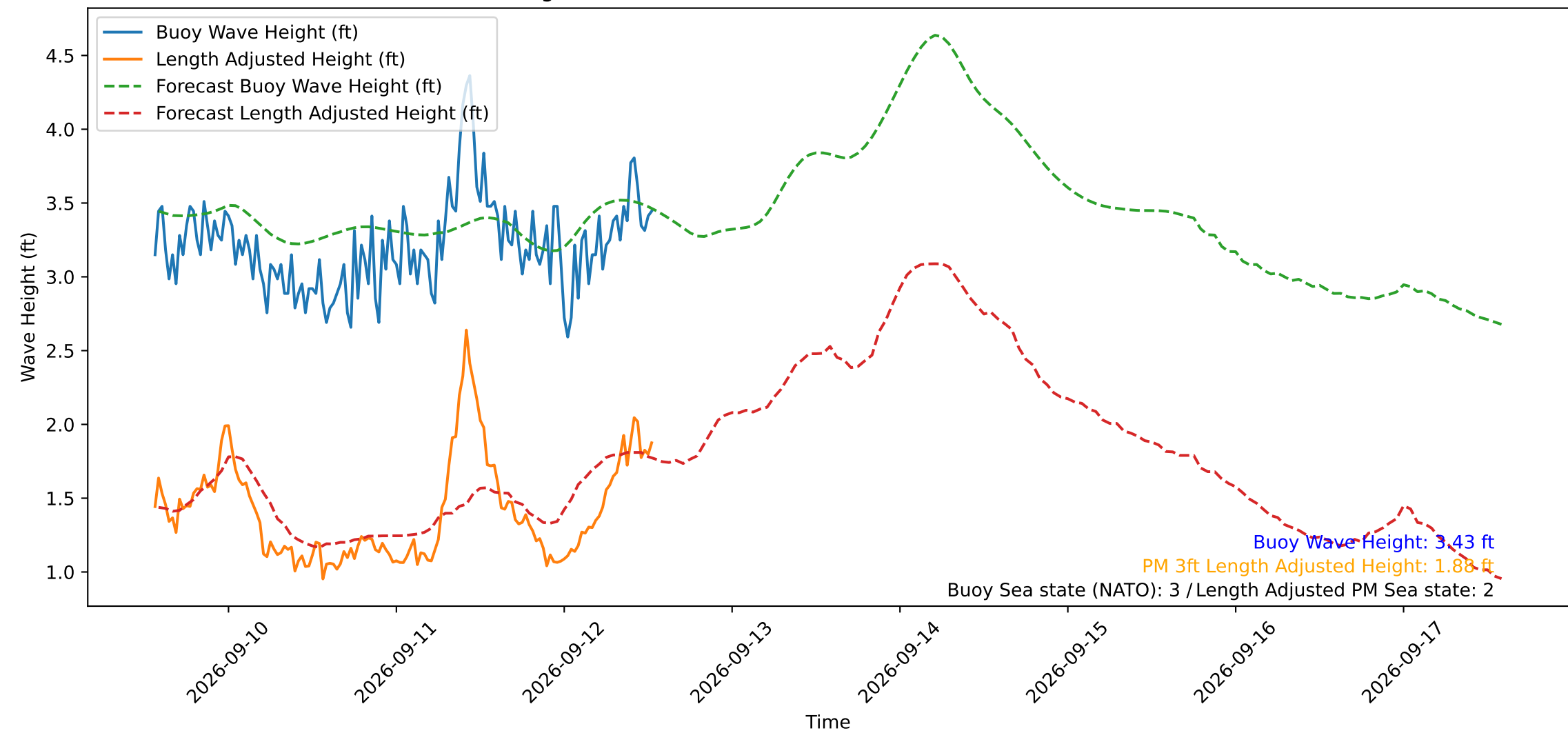
Wave Heights over Time for Oceanside Harbor at 2026-09-12 13:30:29
