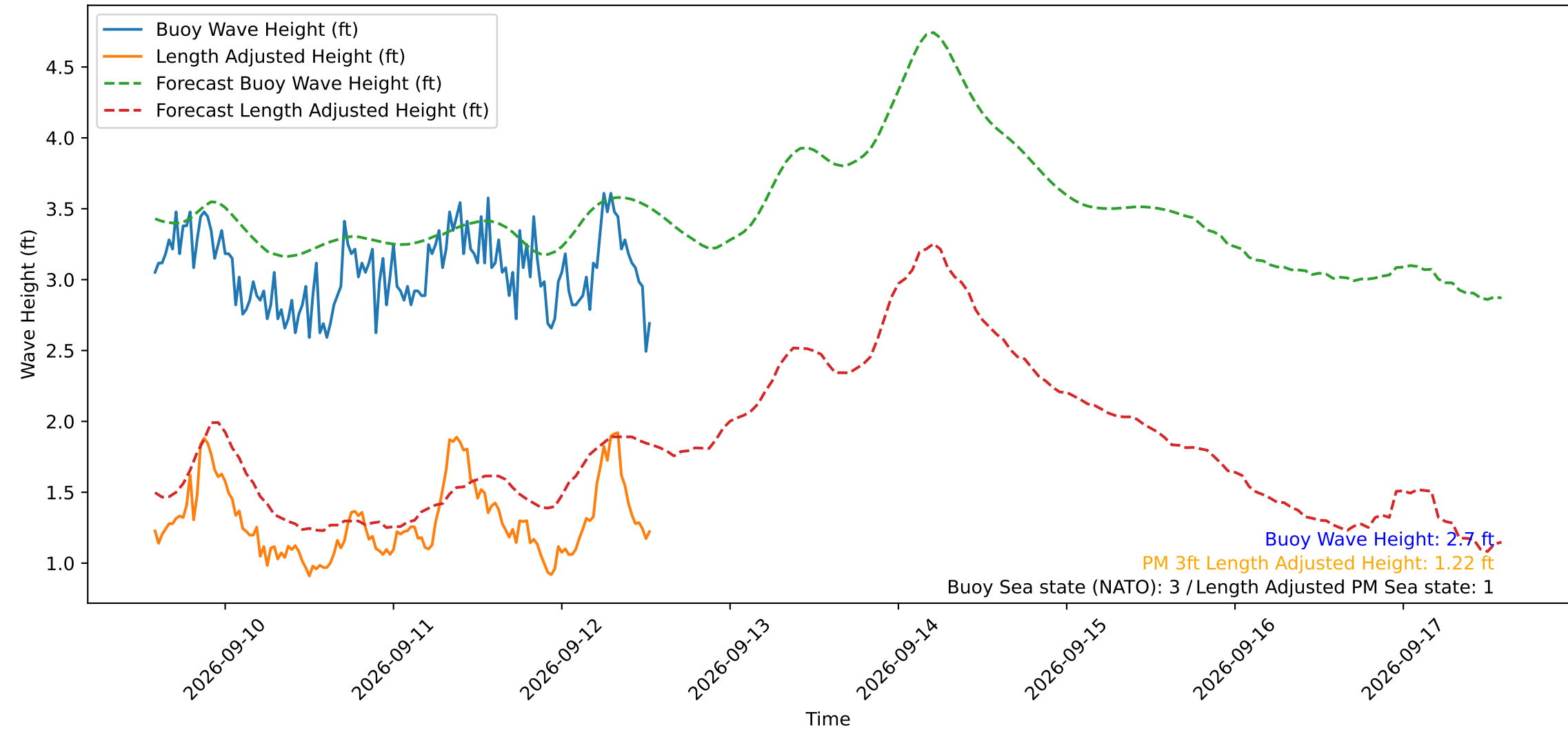
Wave Heights over Time for Green Beach at 2026-09-12 13:31:12
