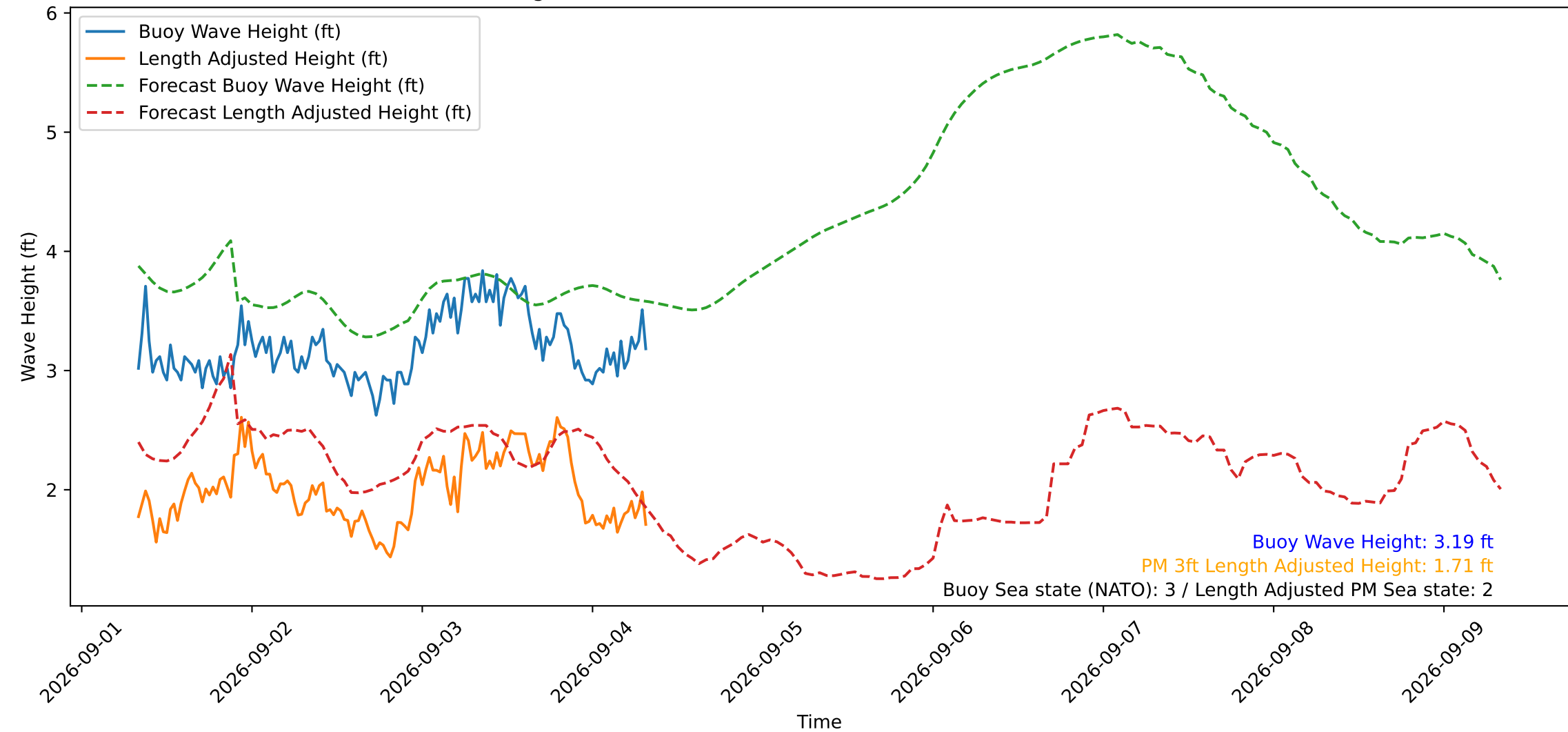
Wave Heights over Time for Oceanside Harbor at 2026-09-04 08:10:30
