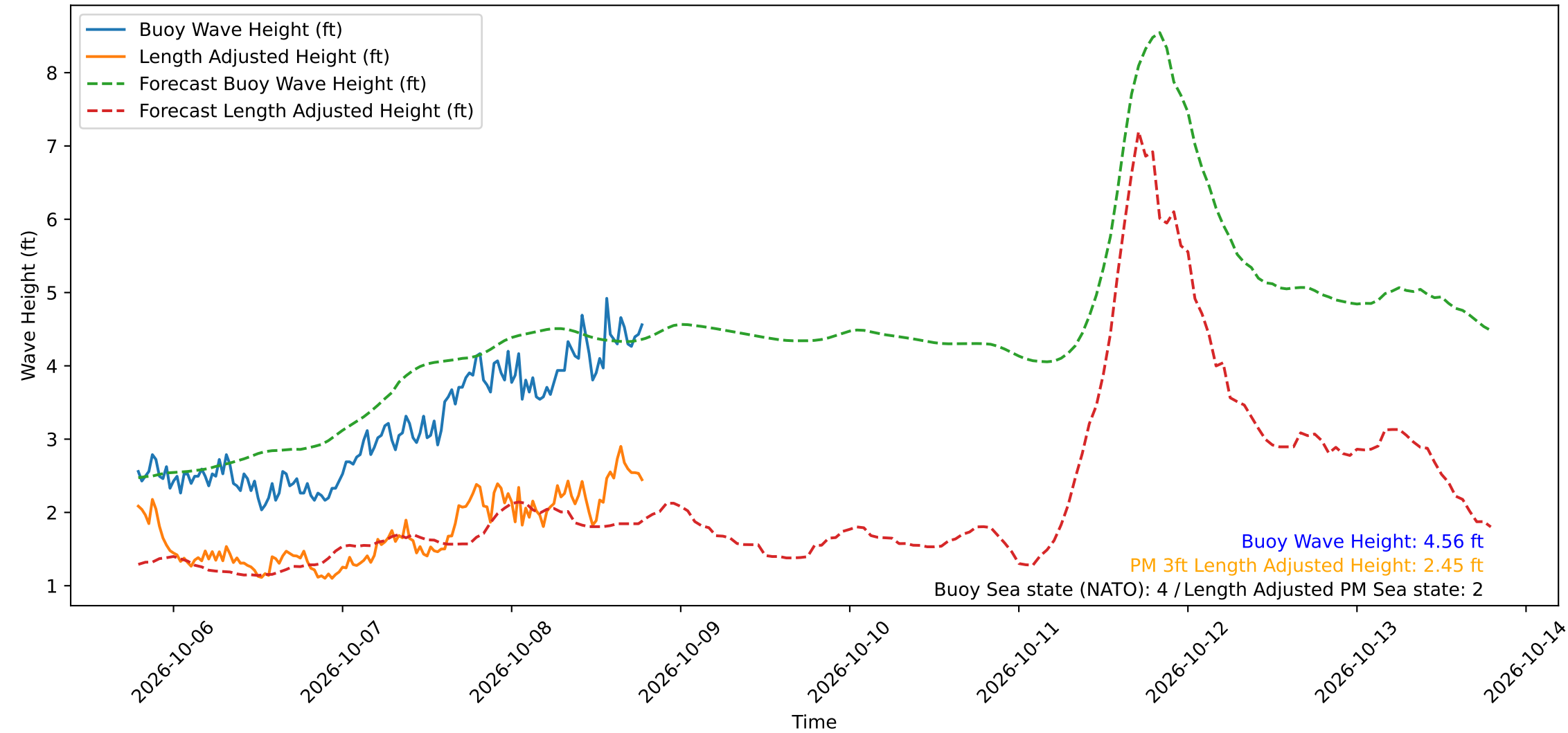
Wave Heights over Time for Oceanside Harbor at 2026-10-08 19:10:30
