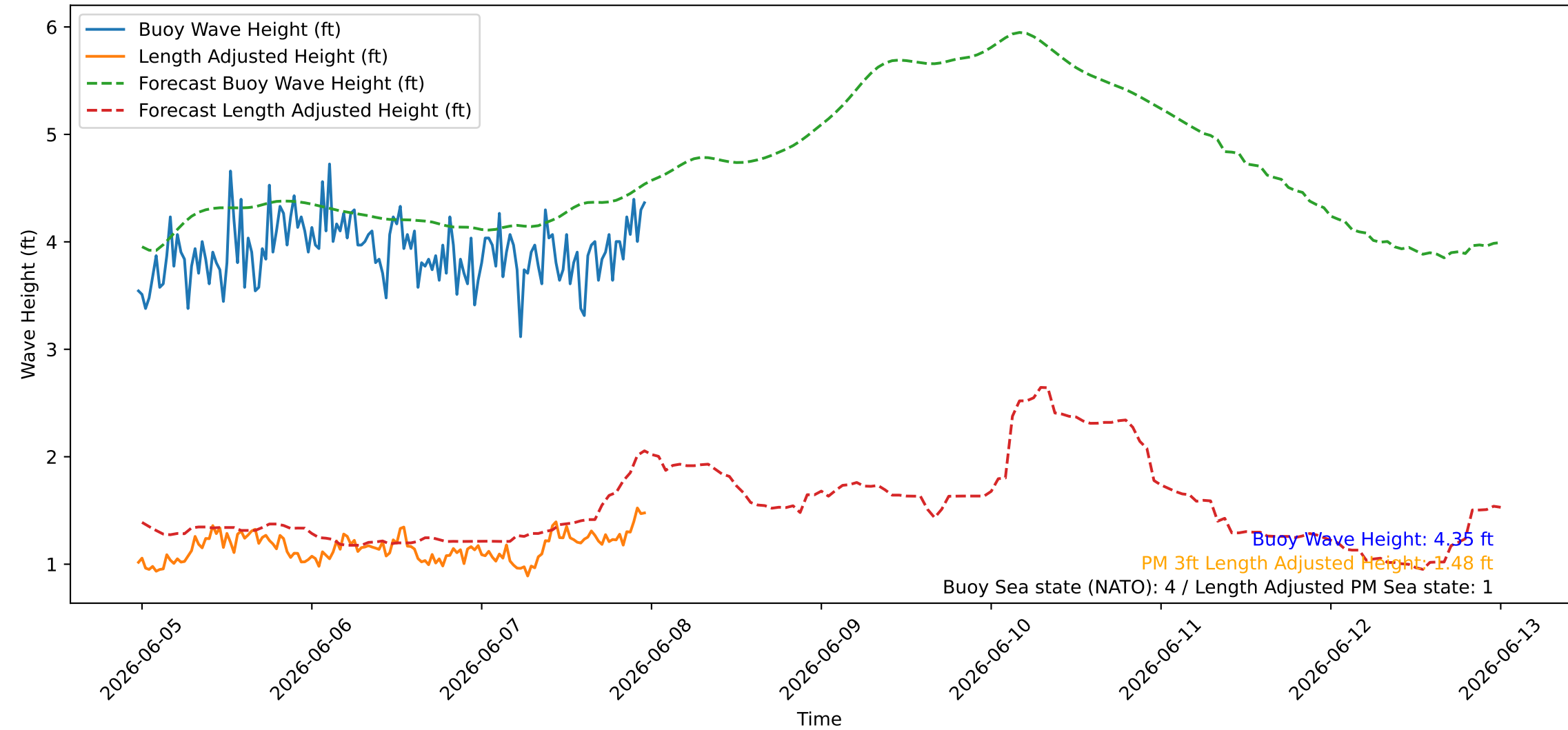
Wave Heights over Time for Green Beach at 2026-06-07 23:41:08
