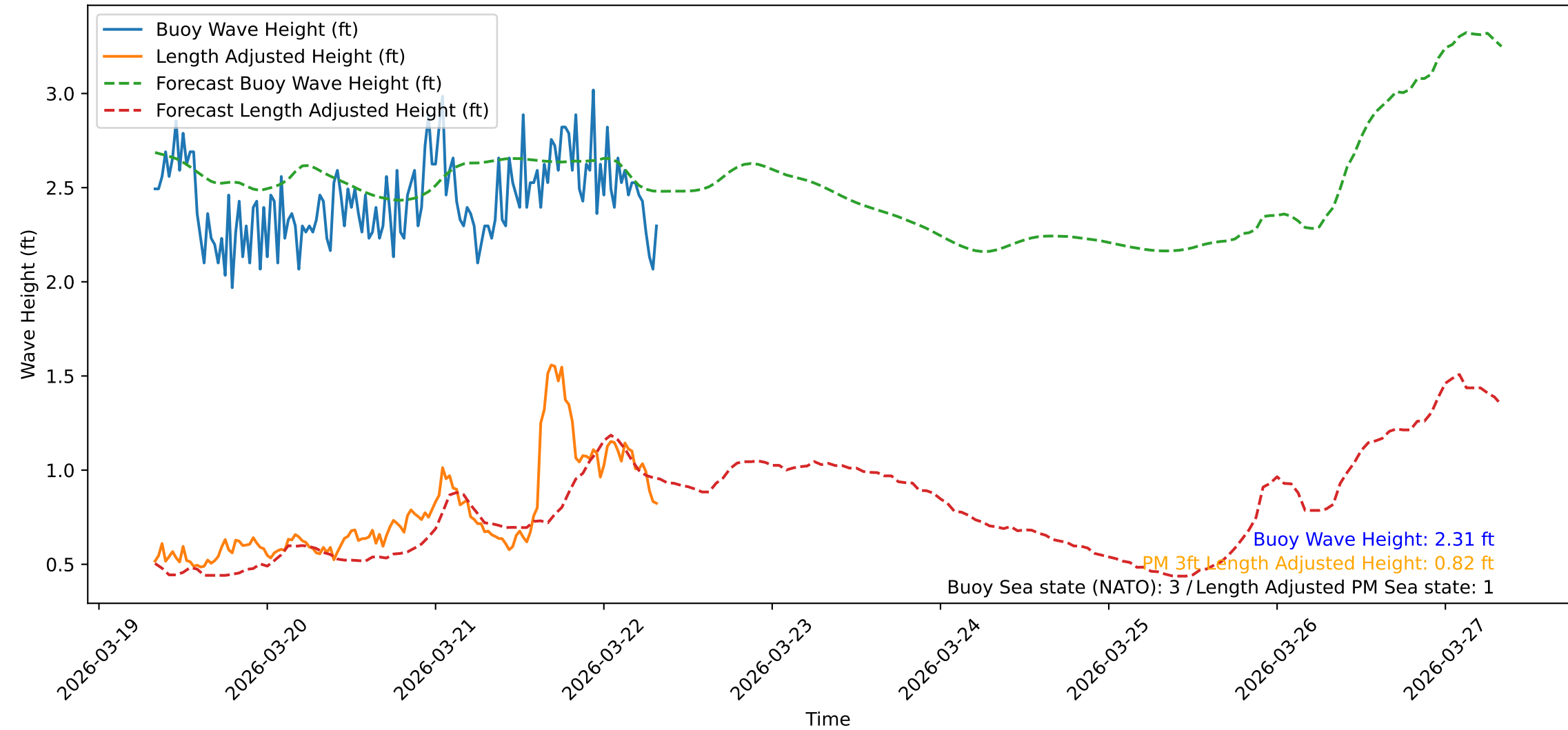
Wave Heights over Time for Oceanside Harbor at 2026-03-22 08:10:32
