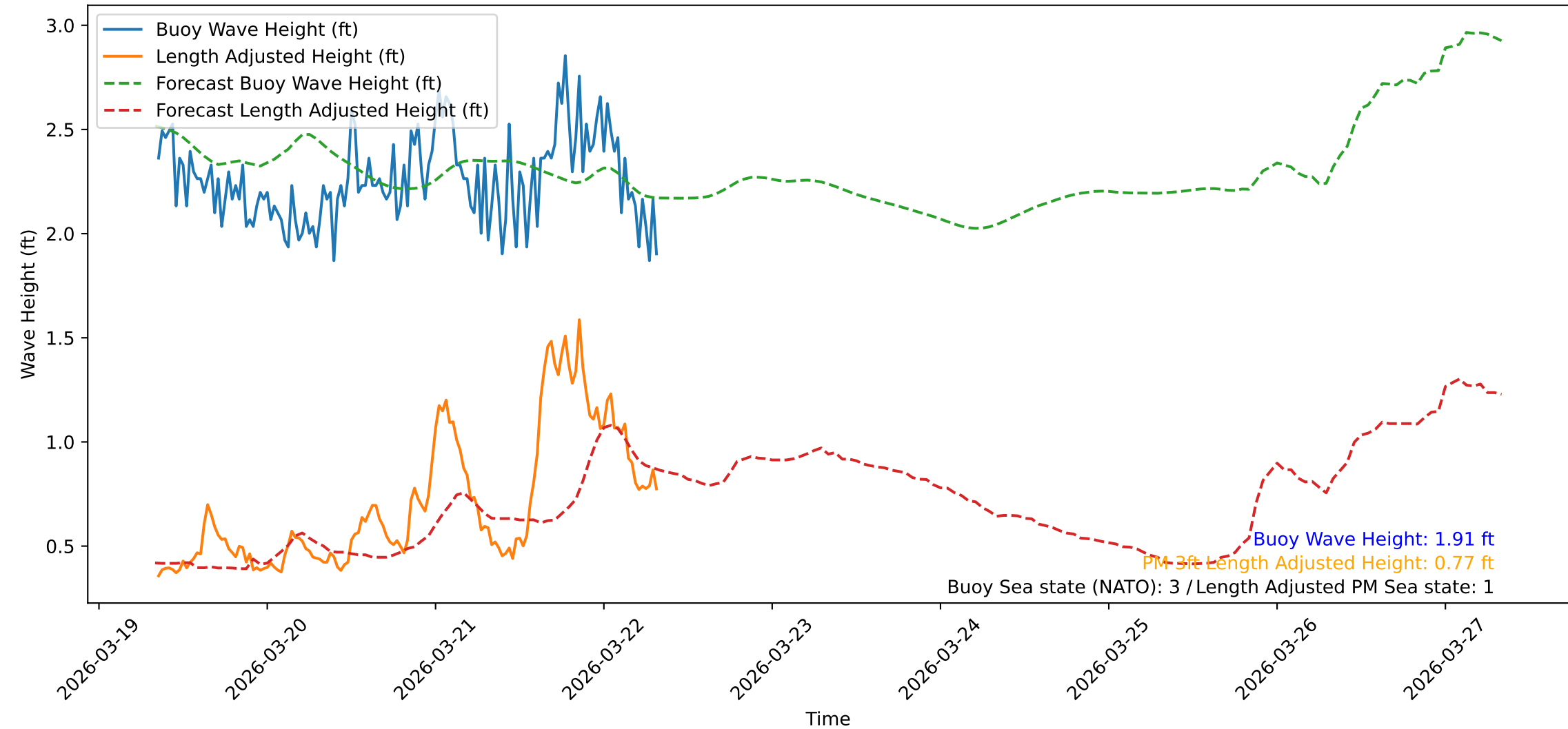
Wave Heights over Time for Red Beach at 2026-03-22 08:10:48
