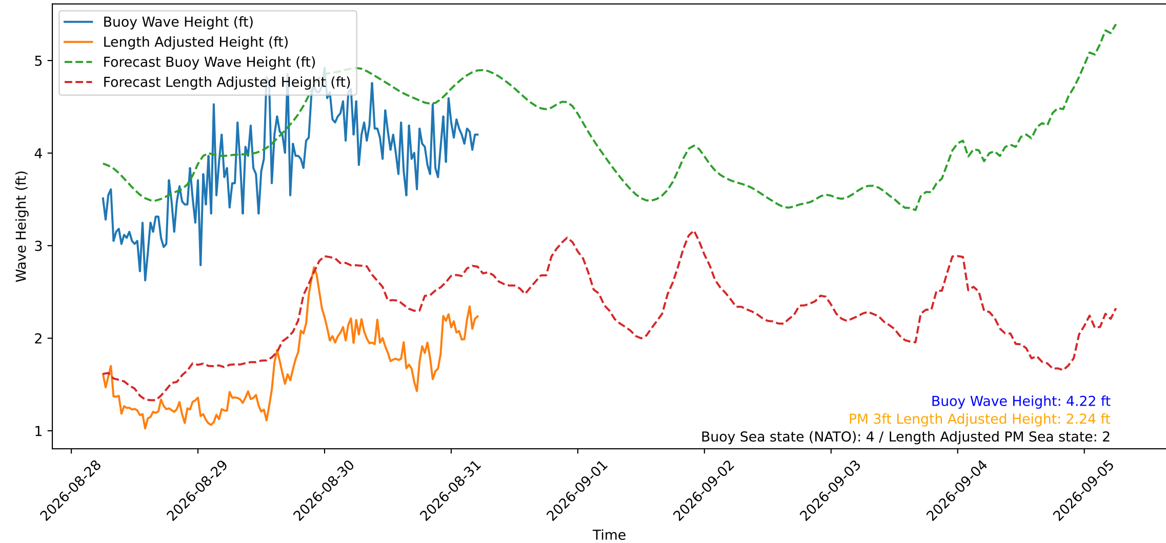
Wave Heights over Time for Green Beach at 2026-08-31 05:41:13
