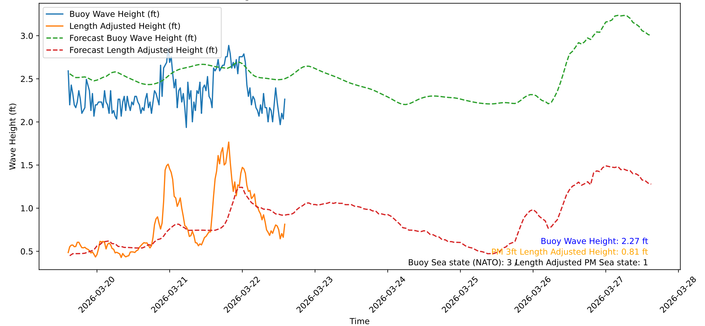
Wave Heights over Time for Green Beach at 2026-03-22 14:41:10
