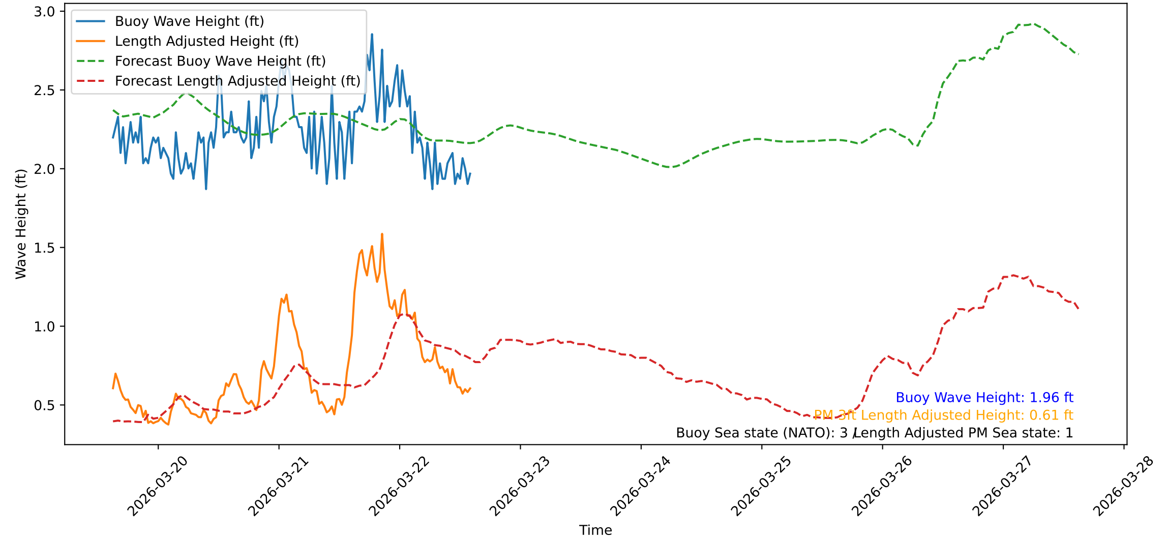
Wave Heights over Time for Red Beach at 2026-03-22 14:40:47
