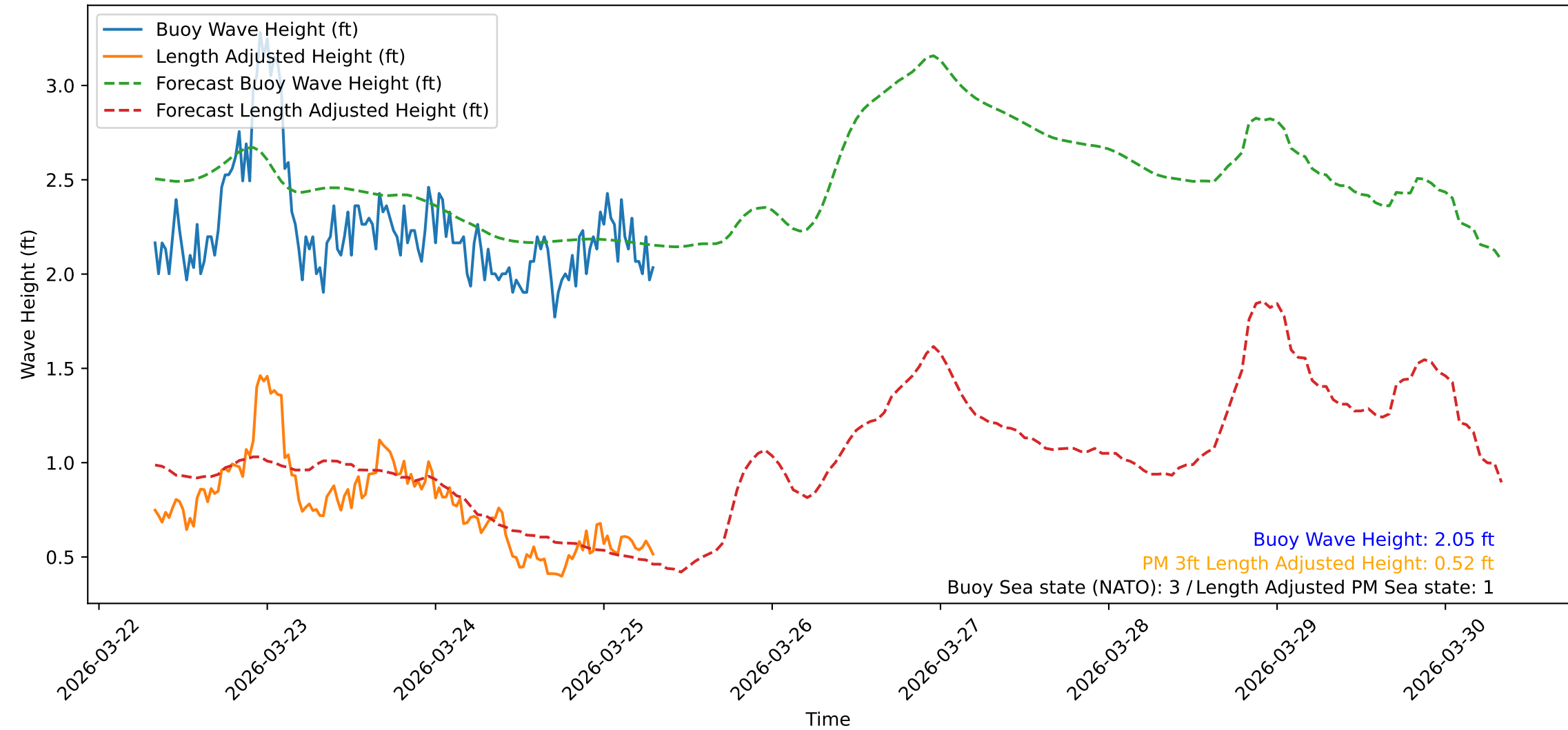
Wave Heights over Time for Green Beach at 2026-03-25 07:51:09
