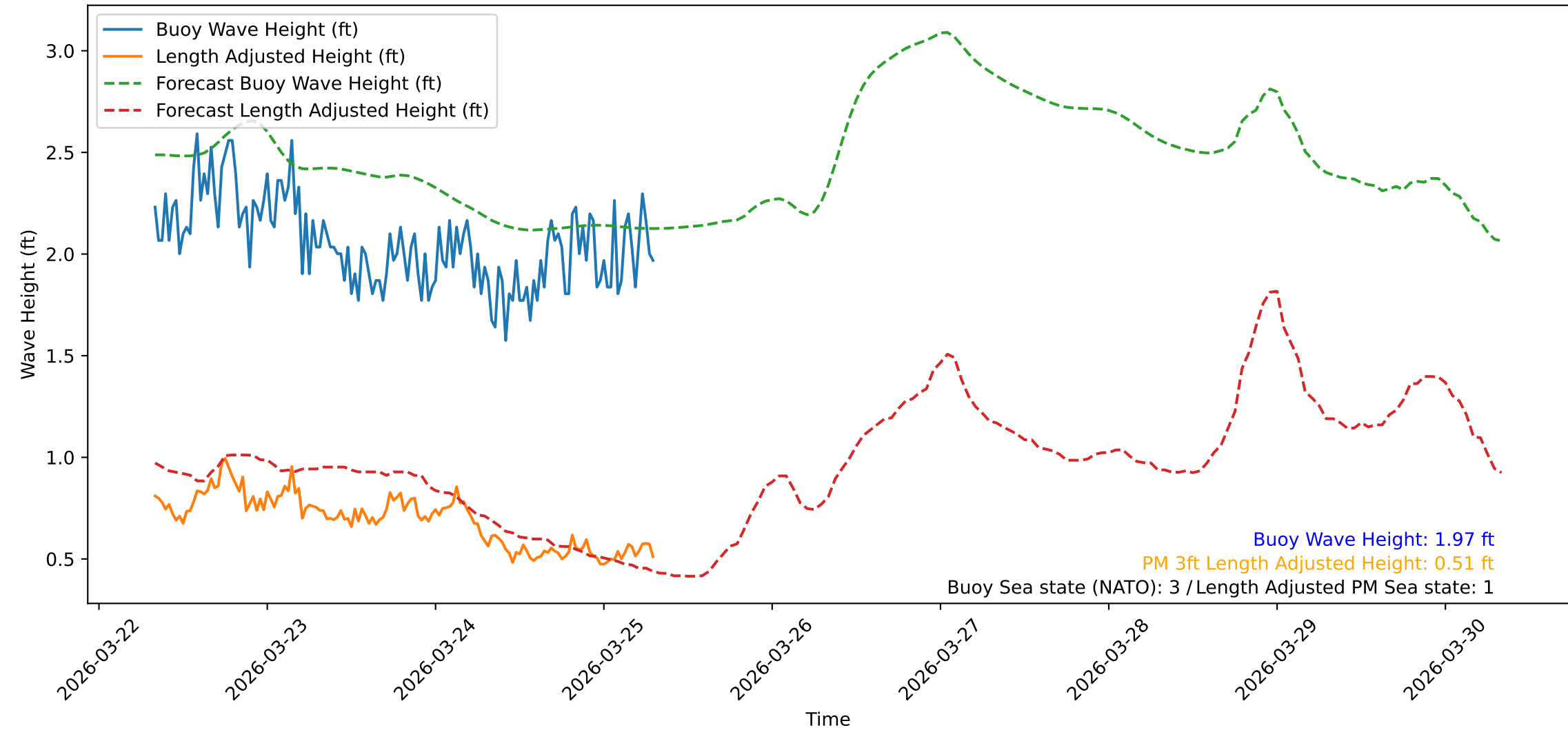
Wave Heights over Time for Oceanside Harbor at 2026-03-25 07:50:31
