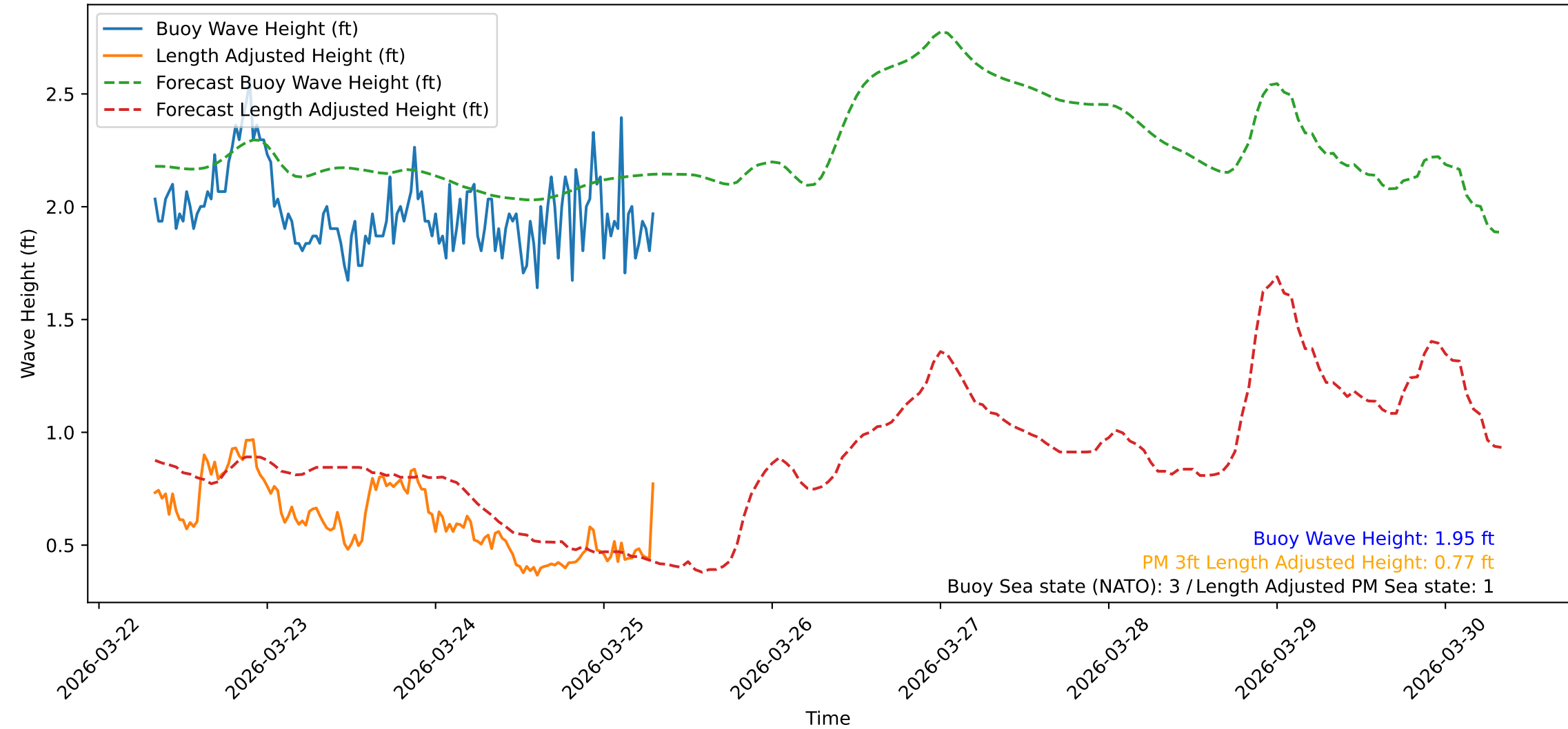
Wave Heights over Time for Red Beach at 2026-03-25 07:50:47
