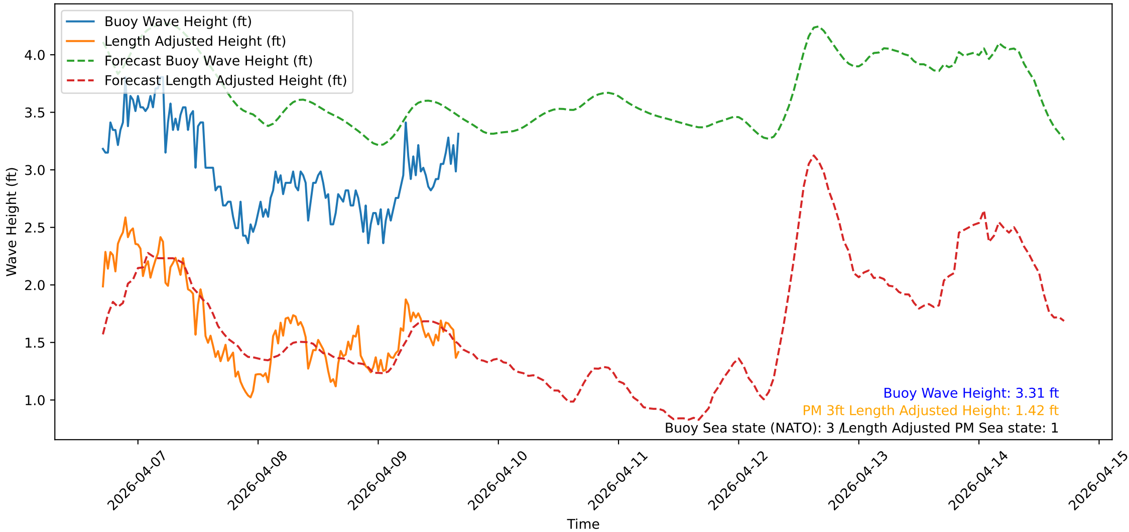
Wave Heights over Time for Green Beach at 2026-04-09 16:51:08
