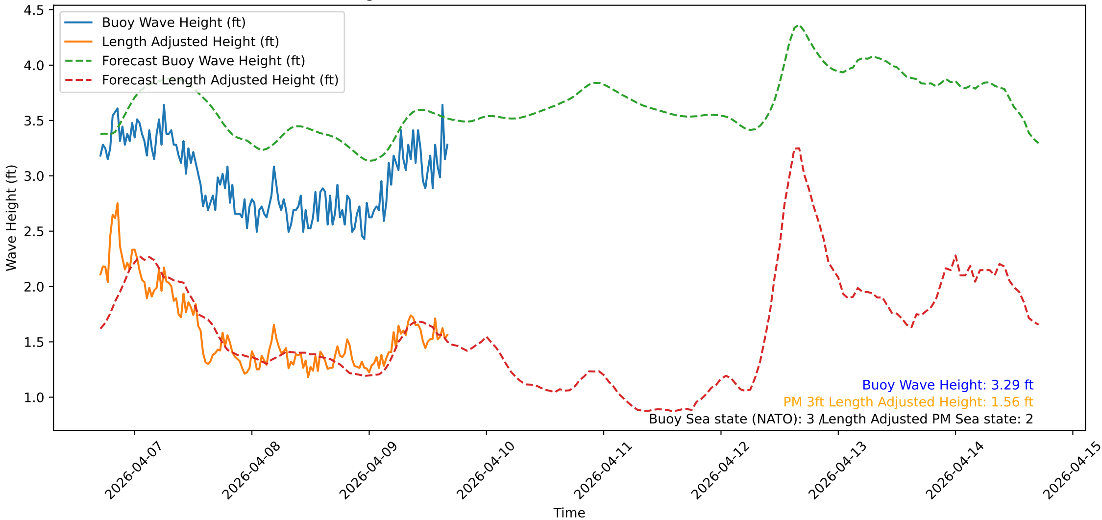
Wave Heights over Time for Oceanside Harbor at 2026-04-09 16:50:30
