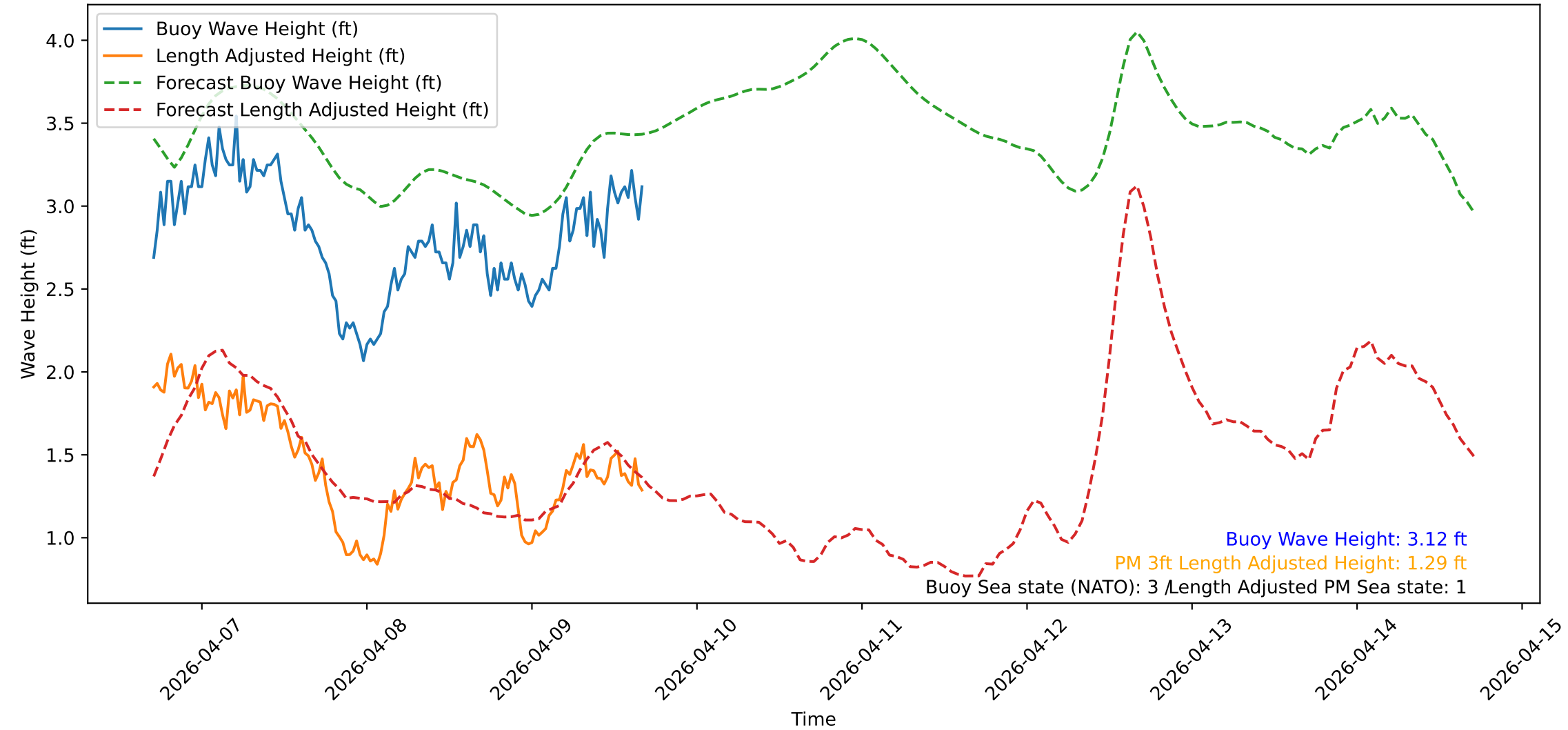
Wave Heights over Time for Red Beach at 2026-04-09 16:50:46
