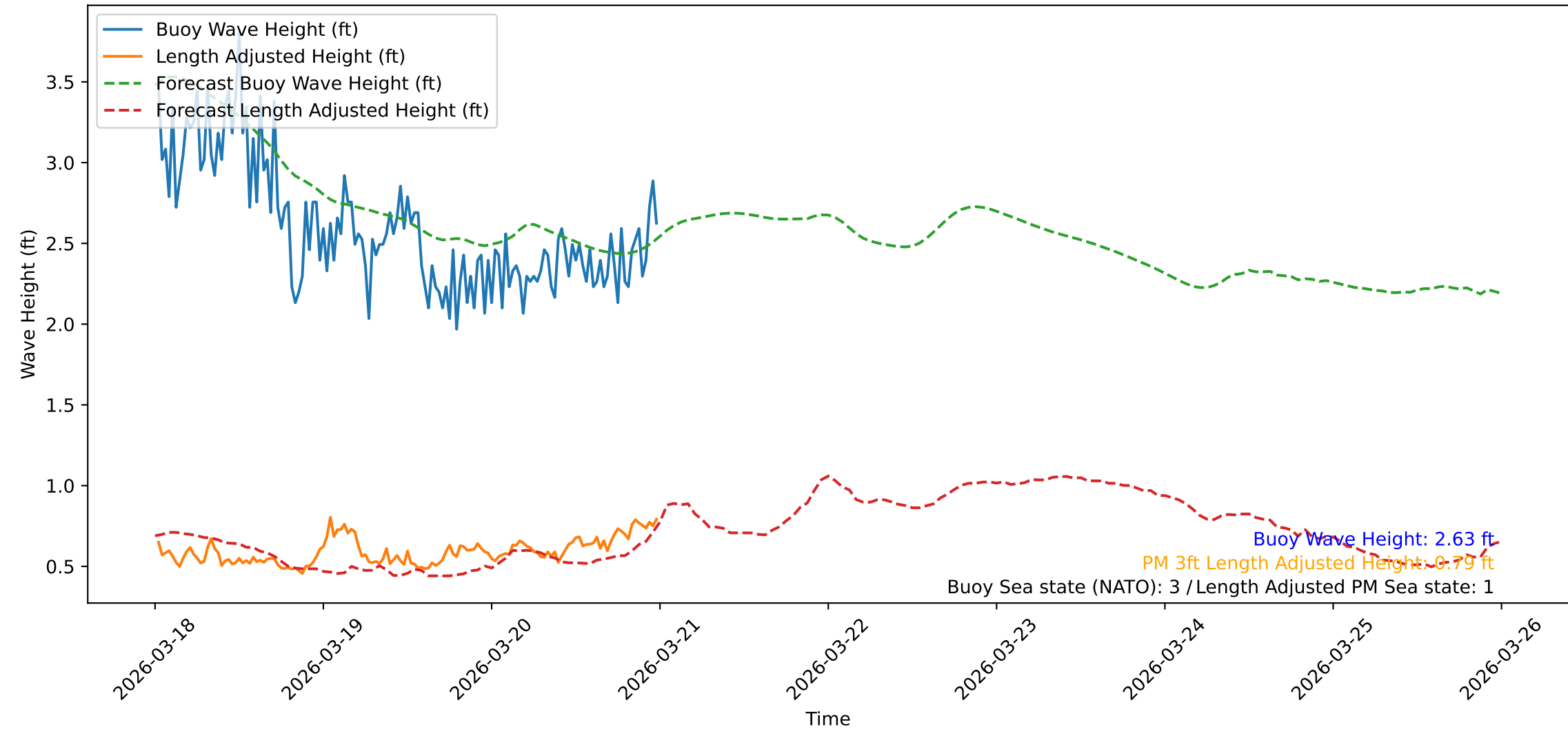
Wave Heights over Time for Oceanside Harbor at 2026-03-21 00:20:31
