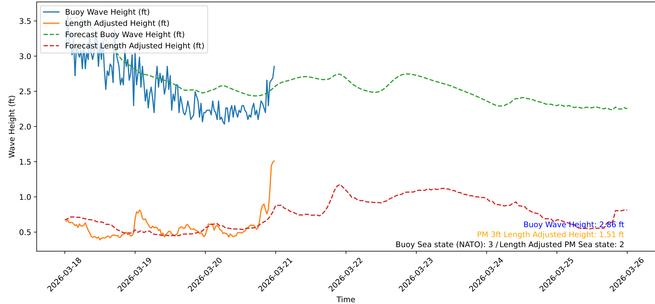
Wave Heights over Time for Green Beach at 2026-03-21 00:21:10
