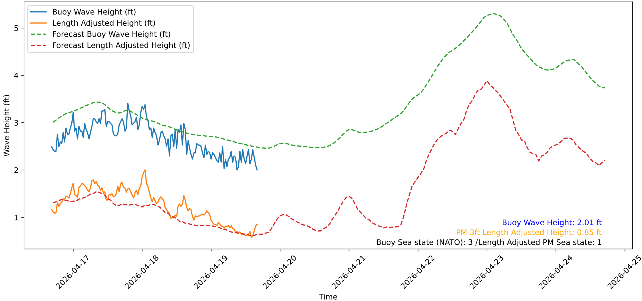
Wave Heights over Time for Oceanside Harbor at 2026-04-19 16:30:32
