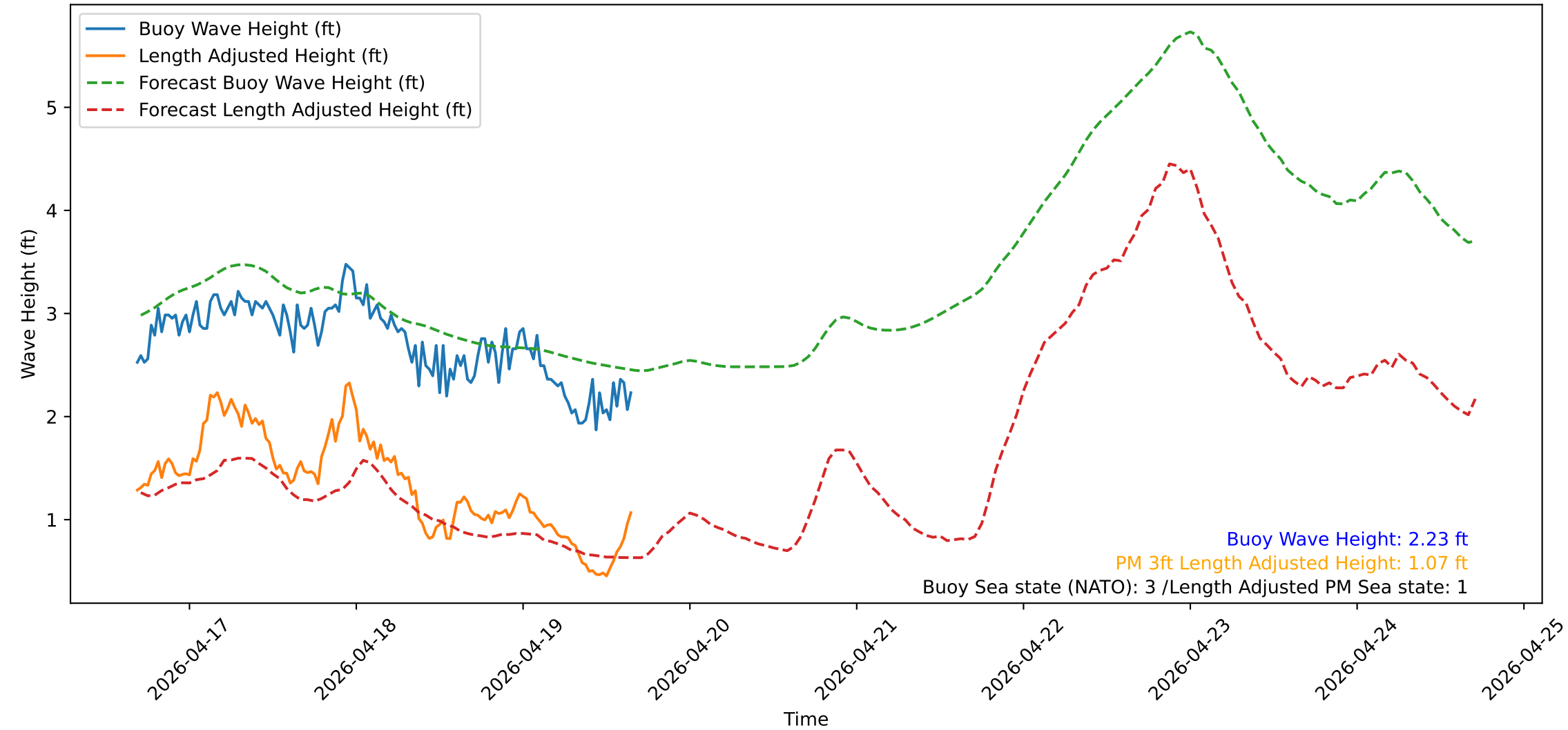
Wave Heights over Time for Green Beach at 2026-04-19 16:31:14
