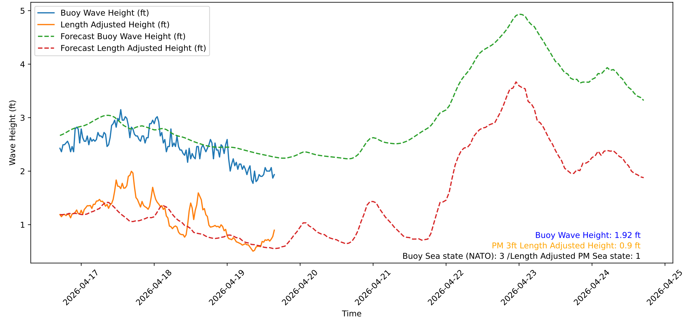
Wave Heights over Time for Red Beach at 2026-04-19 16:30:51
