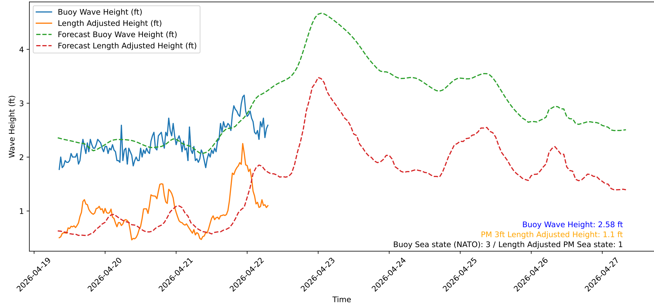
Wave Heights over Time for Red Beach at 2026-04-22 08:00:50
