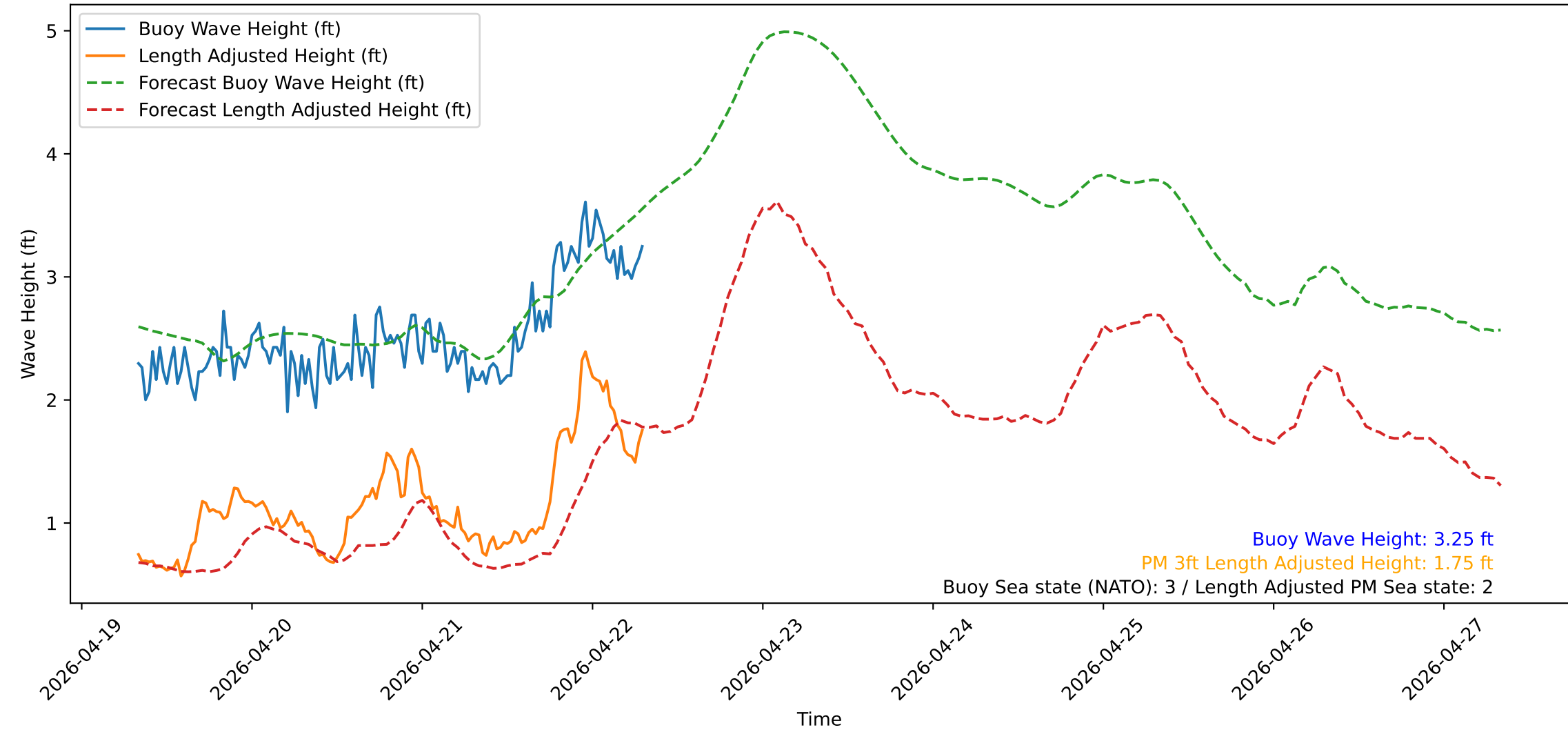
Wave Heights over Time for Oceanside Harbor at 2026-04-22 08:00:31
