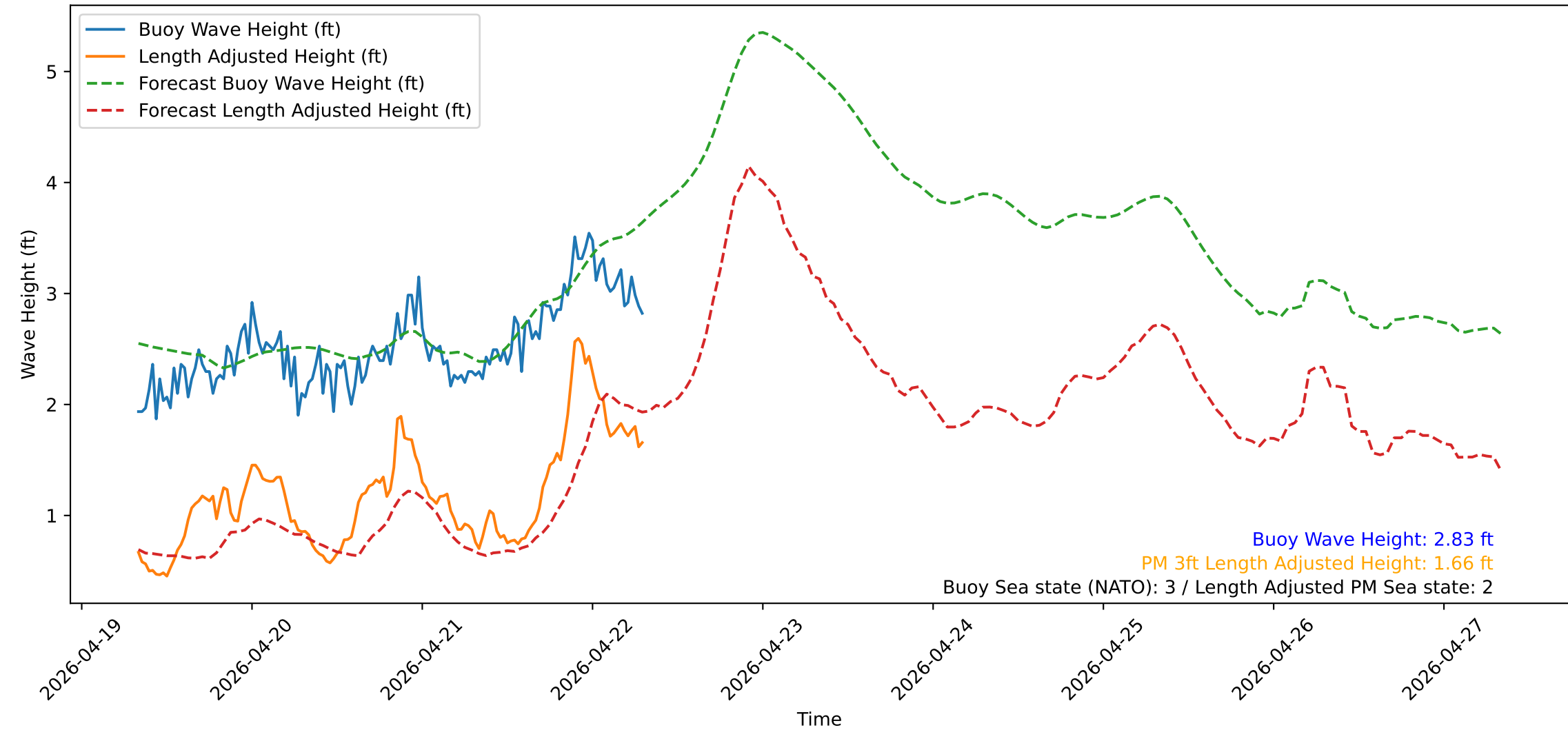
Wave Heights over Time for Green Beach at 2026-04-22 08:01:12
