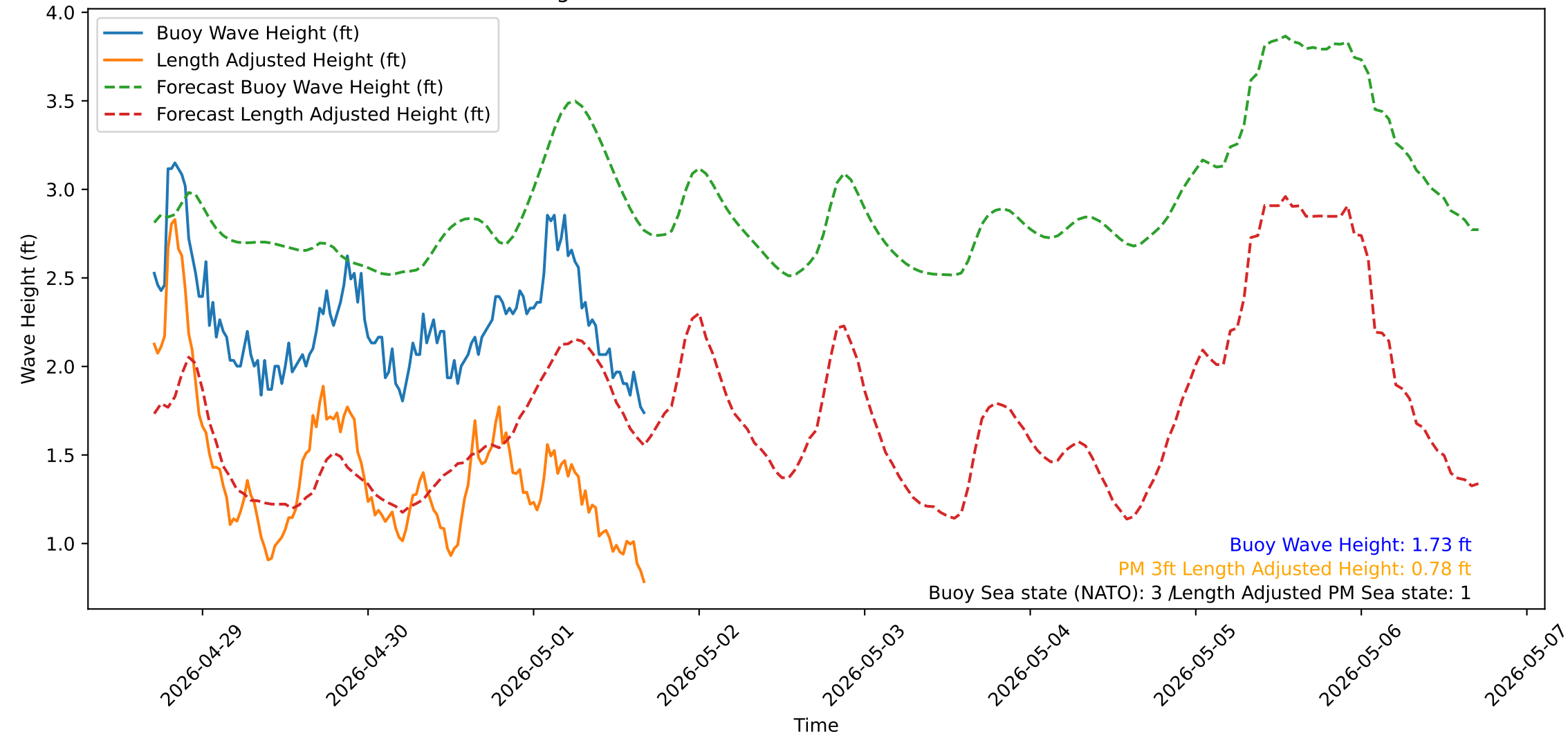
Wave Heights over Time for Green Beach at 2026-05-01 17:01:12
