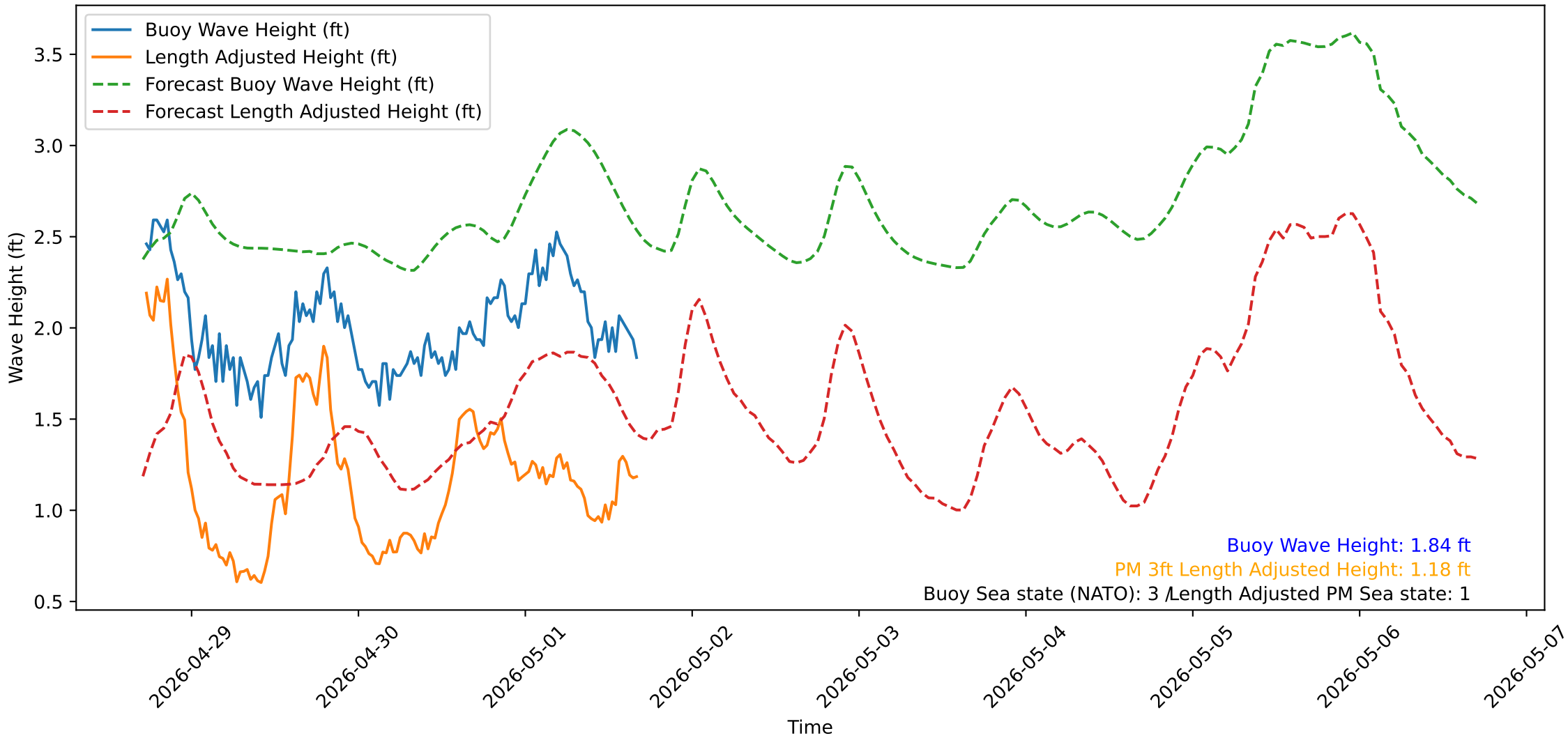
Wave Heights over Time for Red Beach at 2026-05-01 17:00:50
