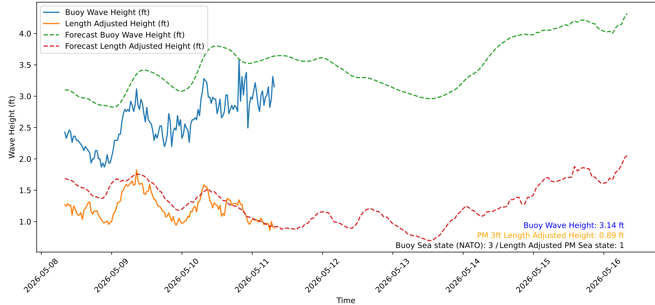
Wave Heights over Time for Oceanside Harbor at 2026-05-11 08:10:32
