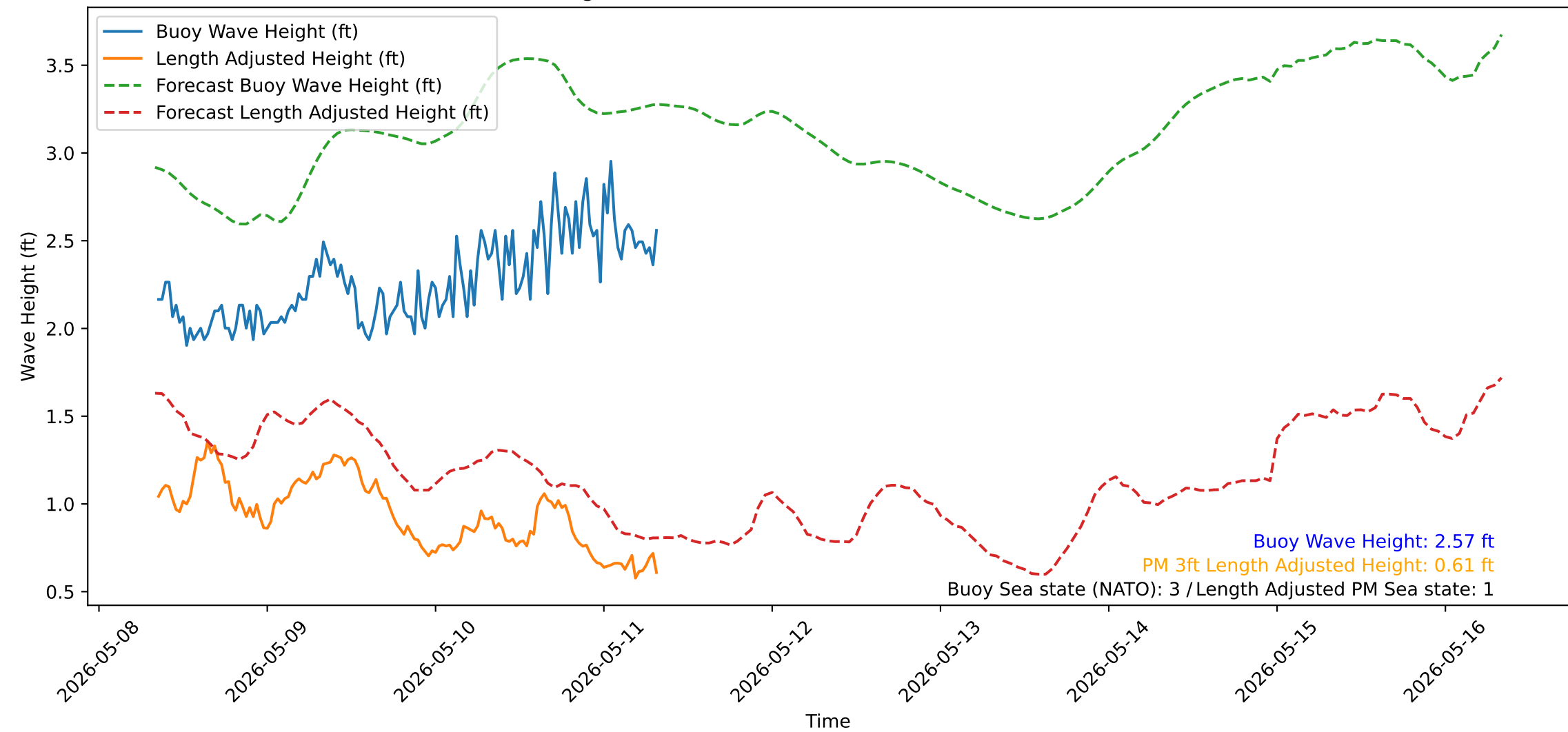
Wave Heights over Time for Red Beach at 2026-05-11 08:10:51
