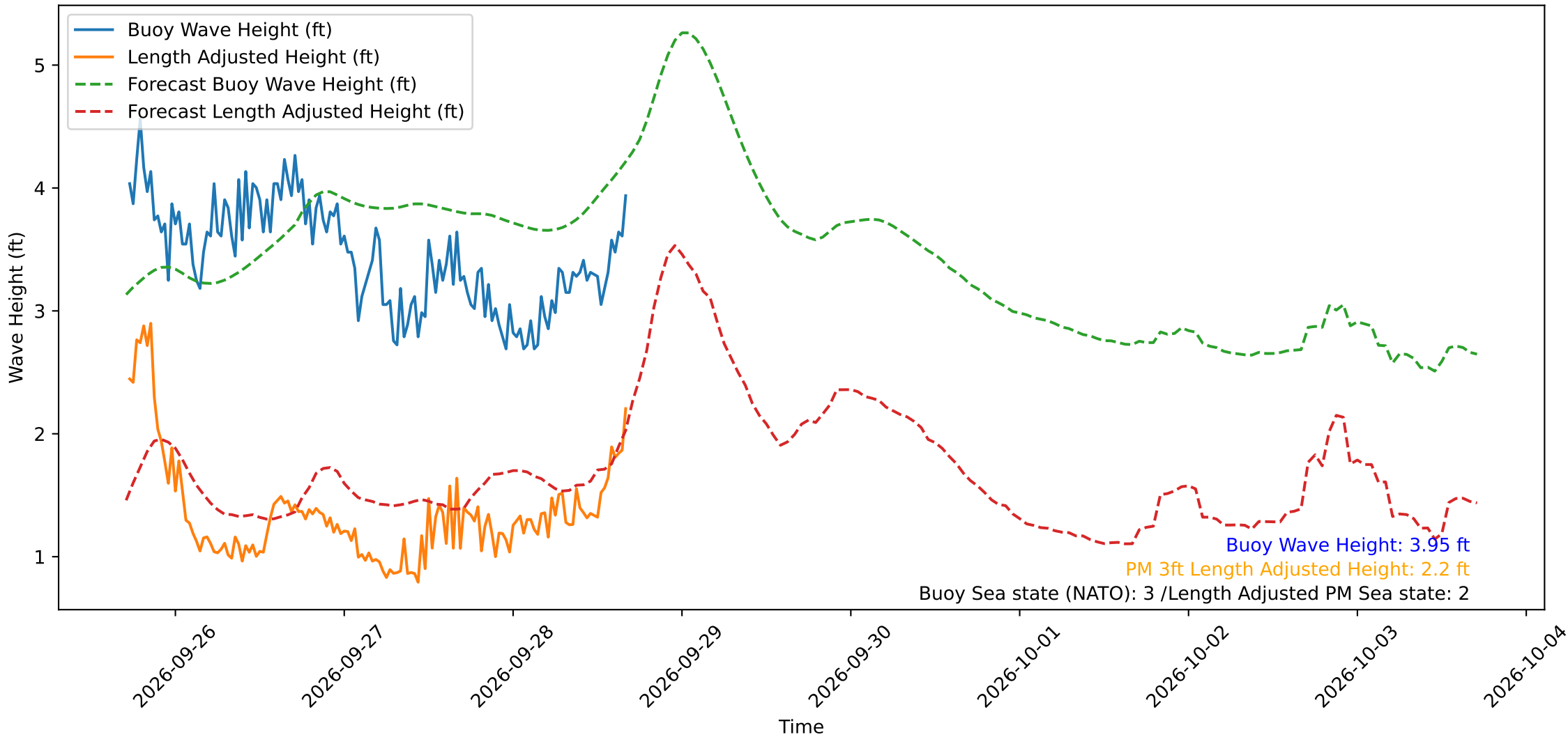
Wave Heights over Time for Green Beach at 2026-09-28 17:01:12
