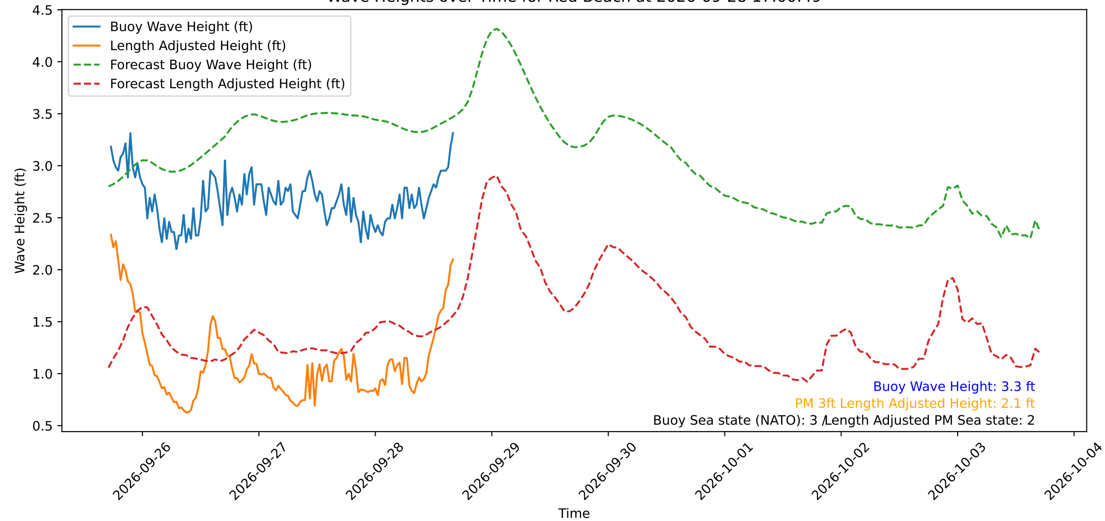
Wave Heights over Time for Red Beach at 2026-09-28 17:00:49
