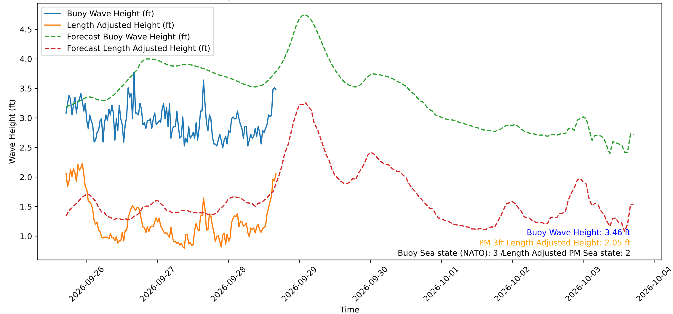
Wave Heights over Time for Oceanside Harbor at 2026-09-28 17:00:30
