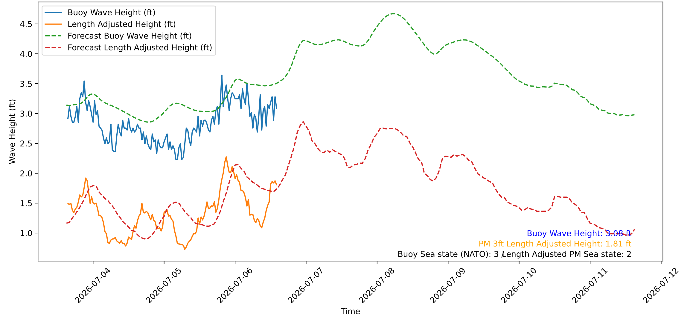
Wave Heights over Time for Red Beach at 2026-07-06 15:00:47
