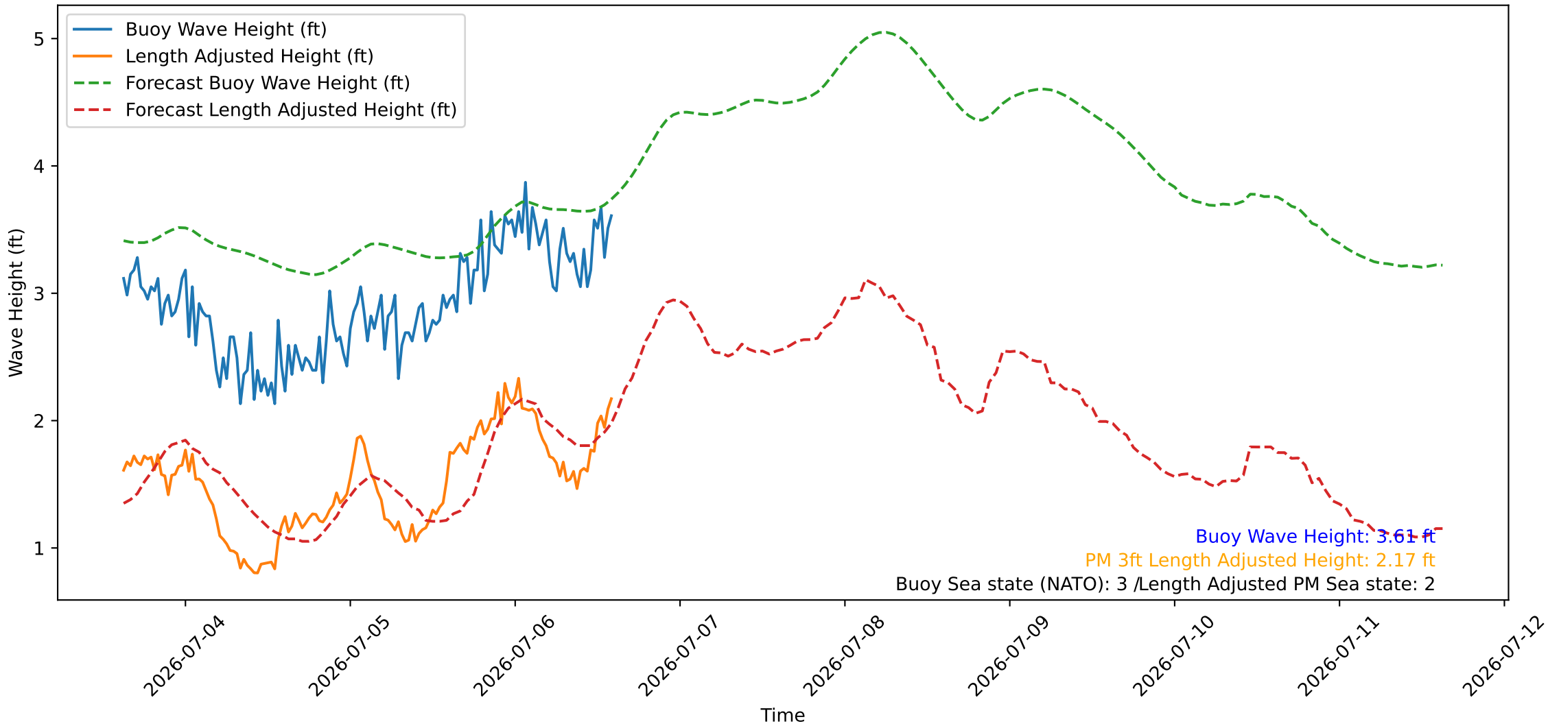
Wave Heights over Time for Oceanside Harbor at 2026-07-06 15:00:27
