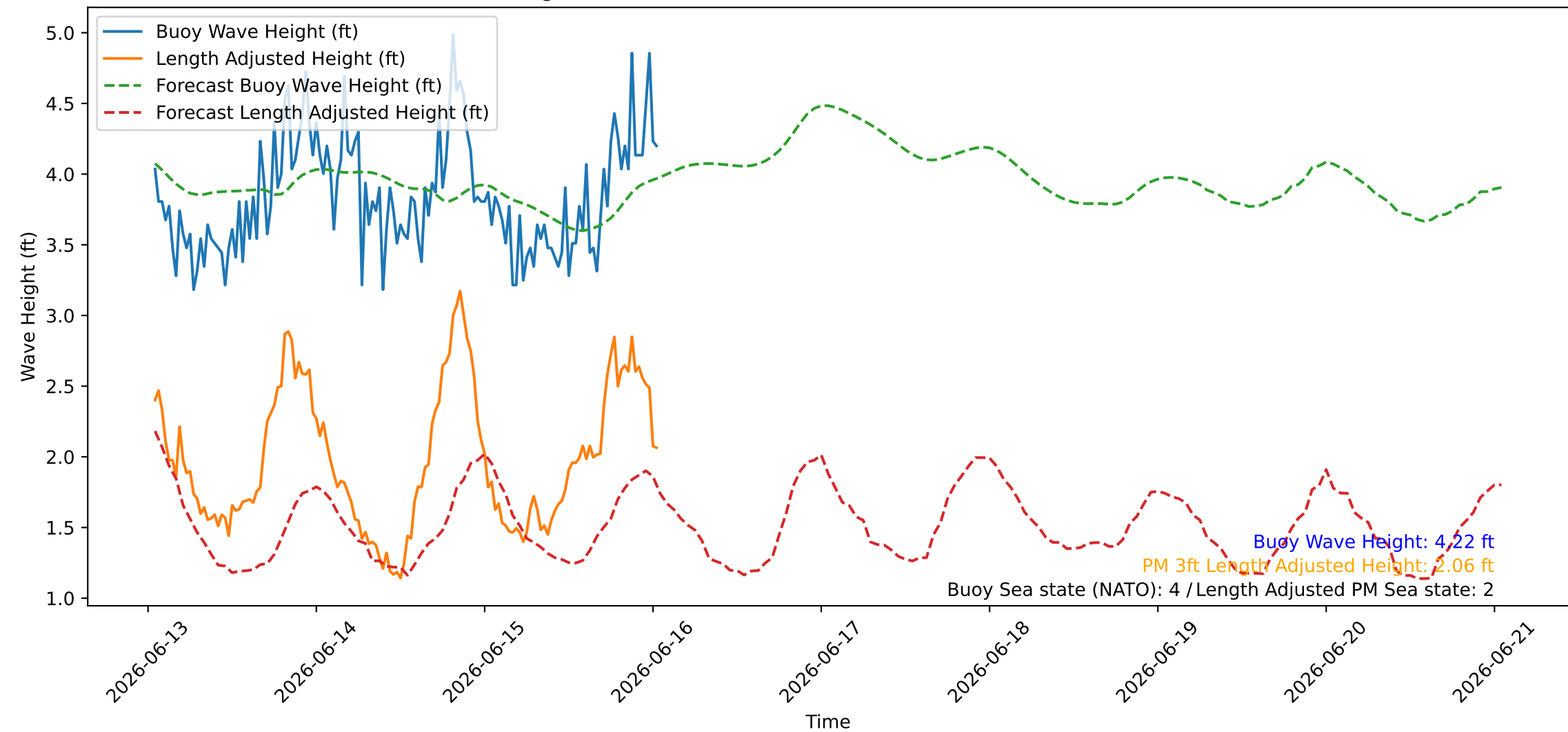
Wave Heights over Time for Oceanside Harbor at 2026-06-16 01:10:26
