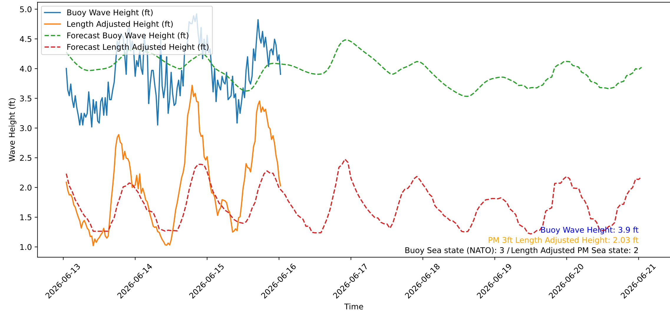
Wave Heights over Time for Green Beach at 2026-06-16 01:11:07
