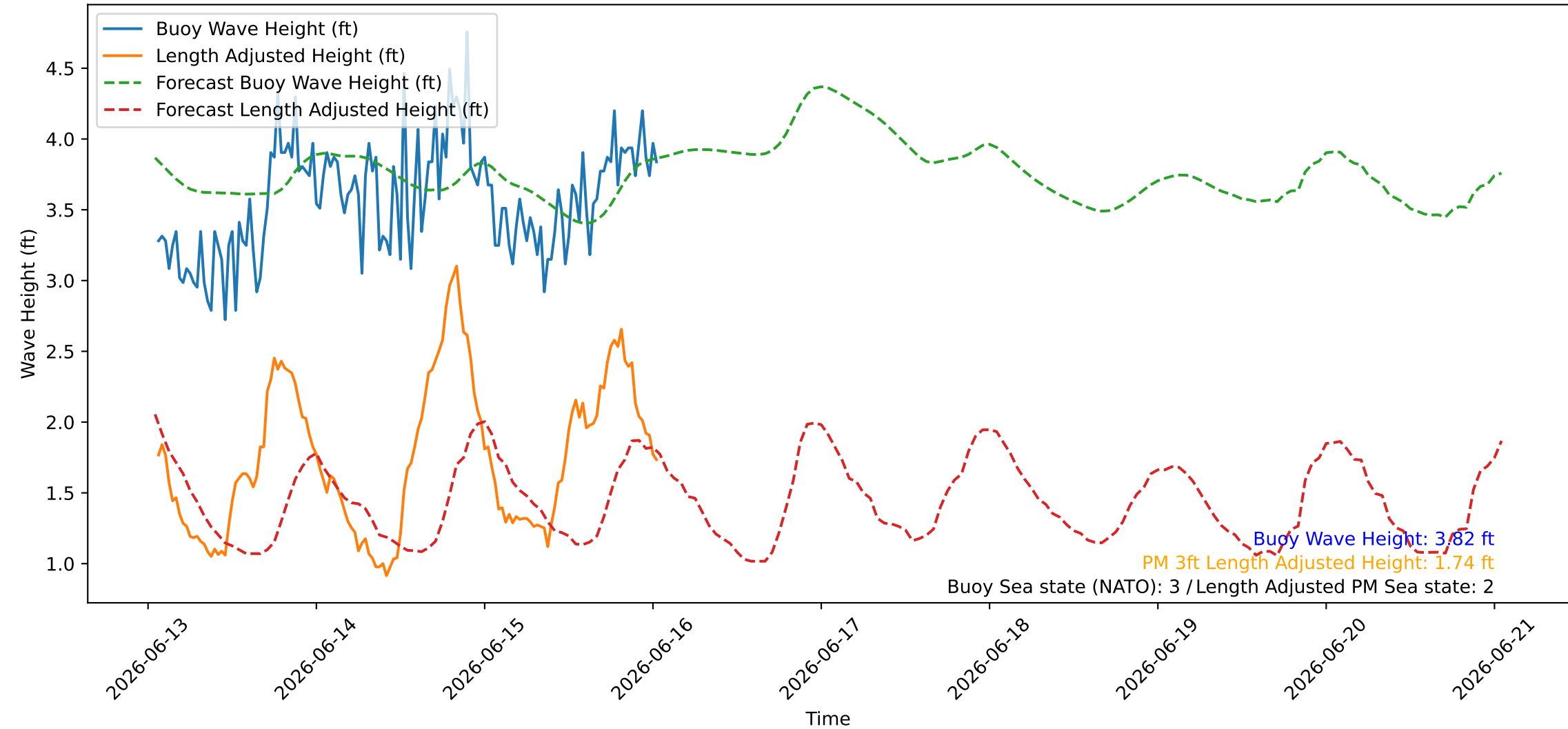
Wave Heights over Time for Red Beach at 2026-06-16 01:10:45
