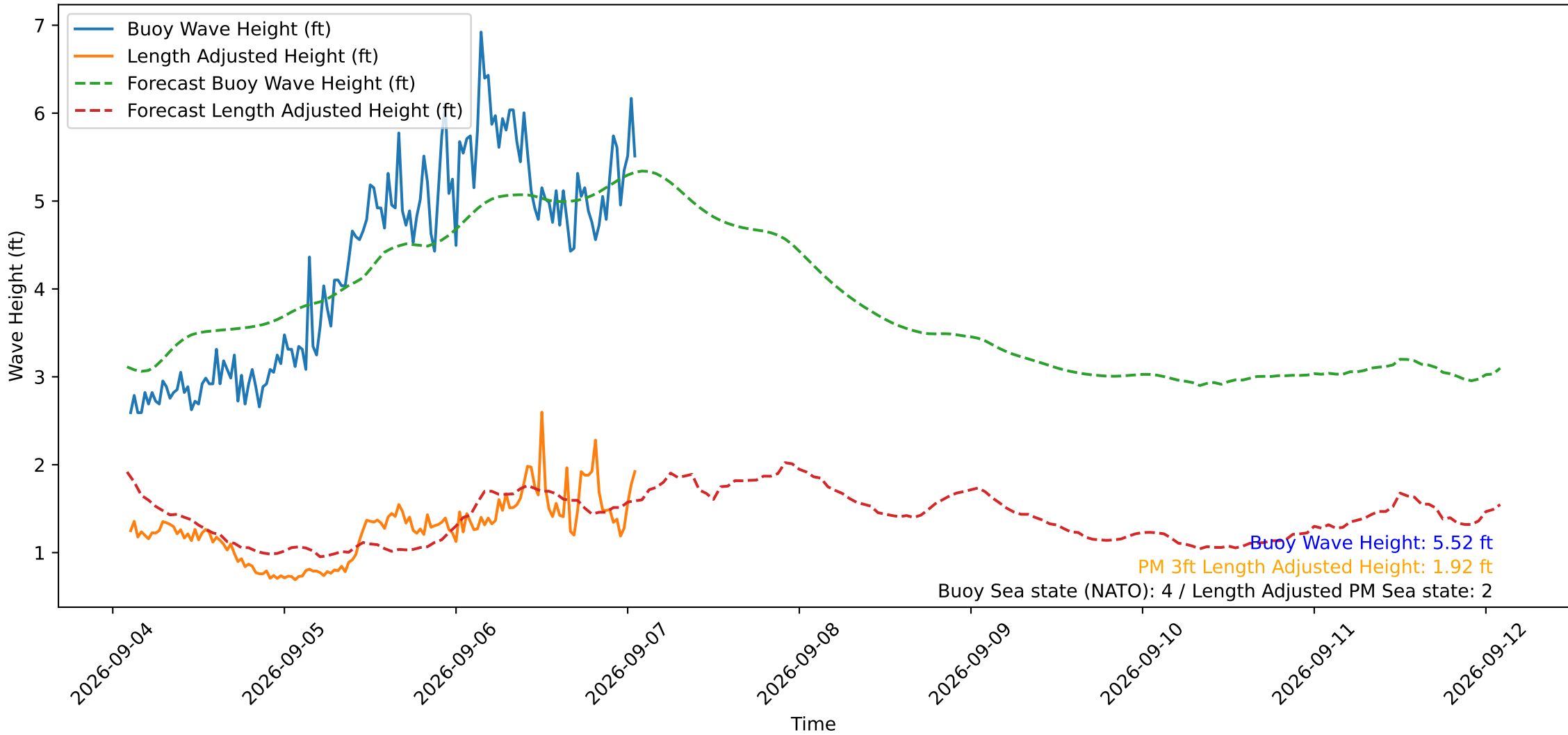
Wave Heights over Time for Red Beach at 2026-09-07 02:00:49
