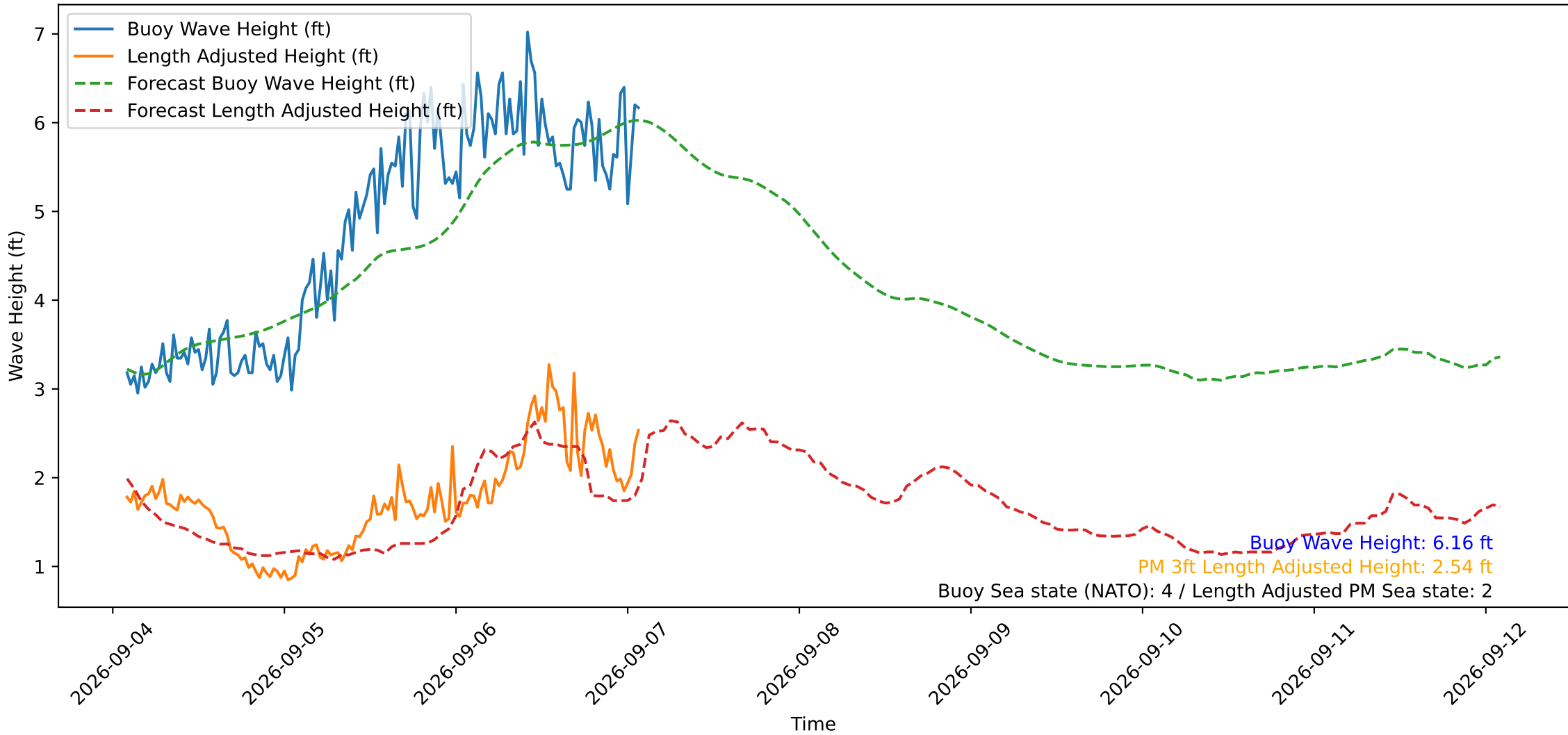
Wave Heights over Time for Oceanside Harbor at 2026-09-07 02:00:30
