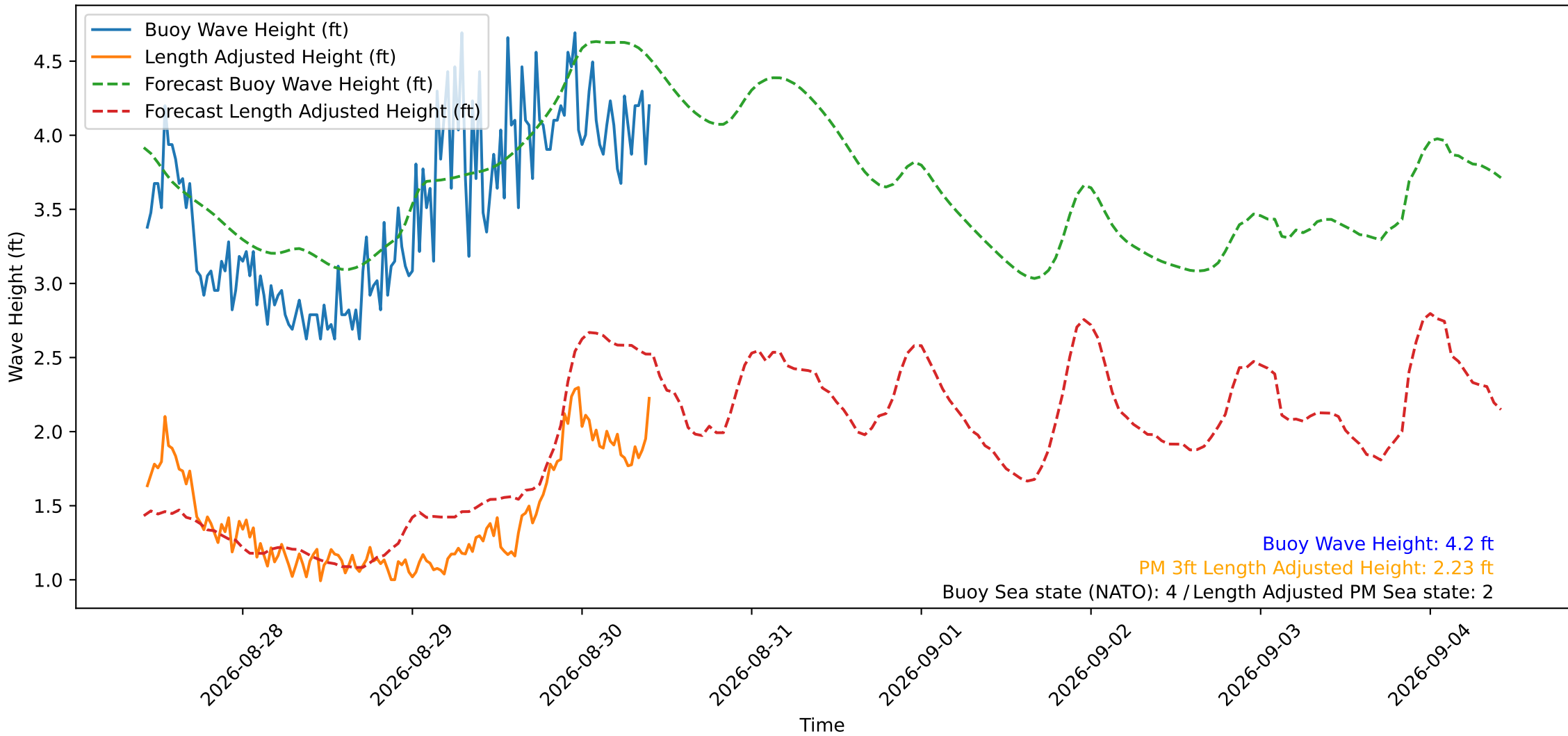
Wave Heights over Time for Red Beach at 2026-08-30 10:10:49
