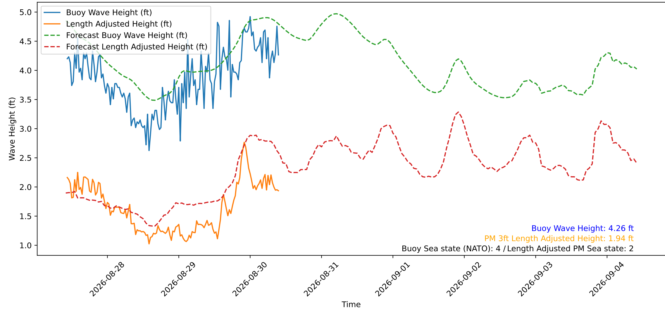
Wave Heights over Time for Green Beach at 2026-08-30 10:11:12
