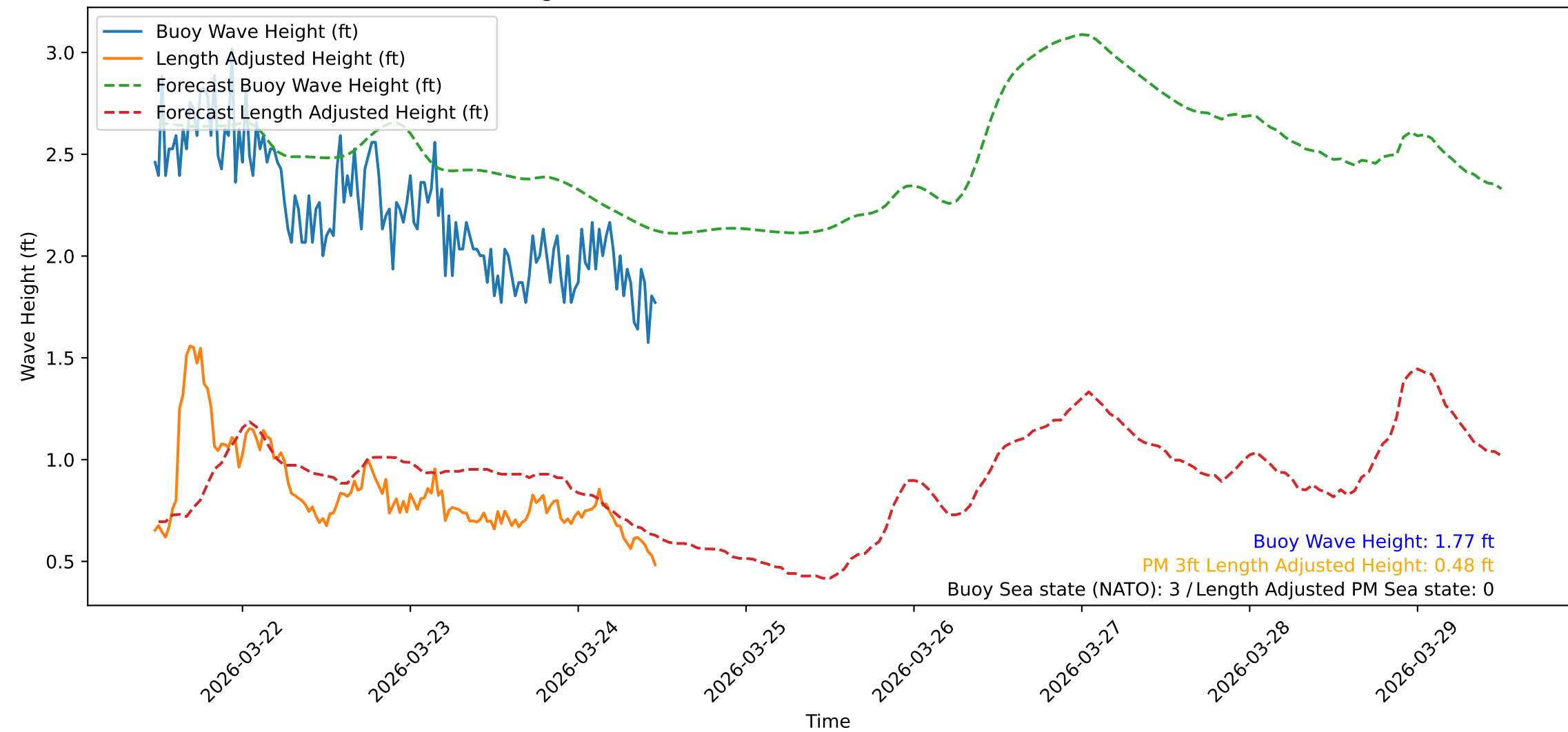
Wave Heights over Time for Oceanside Harbor at 2026-03-24 11:30:31
