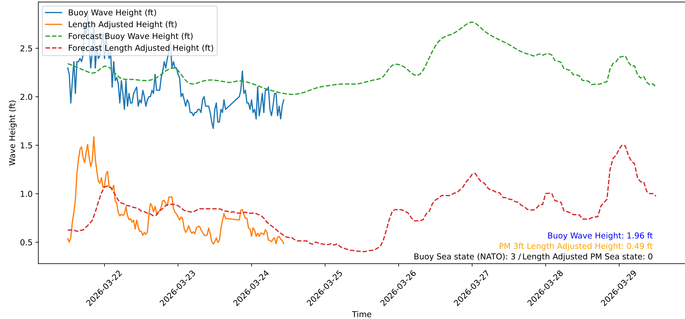
Wave Heights over Time for Red Beach at 2026-03-24 11:30:47
