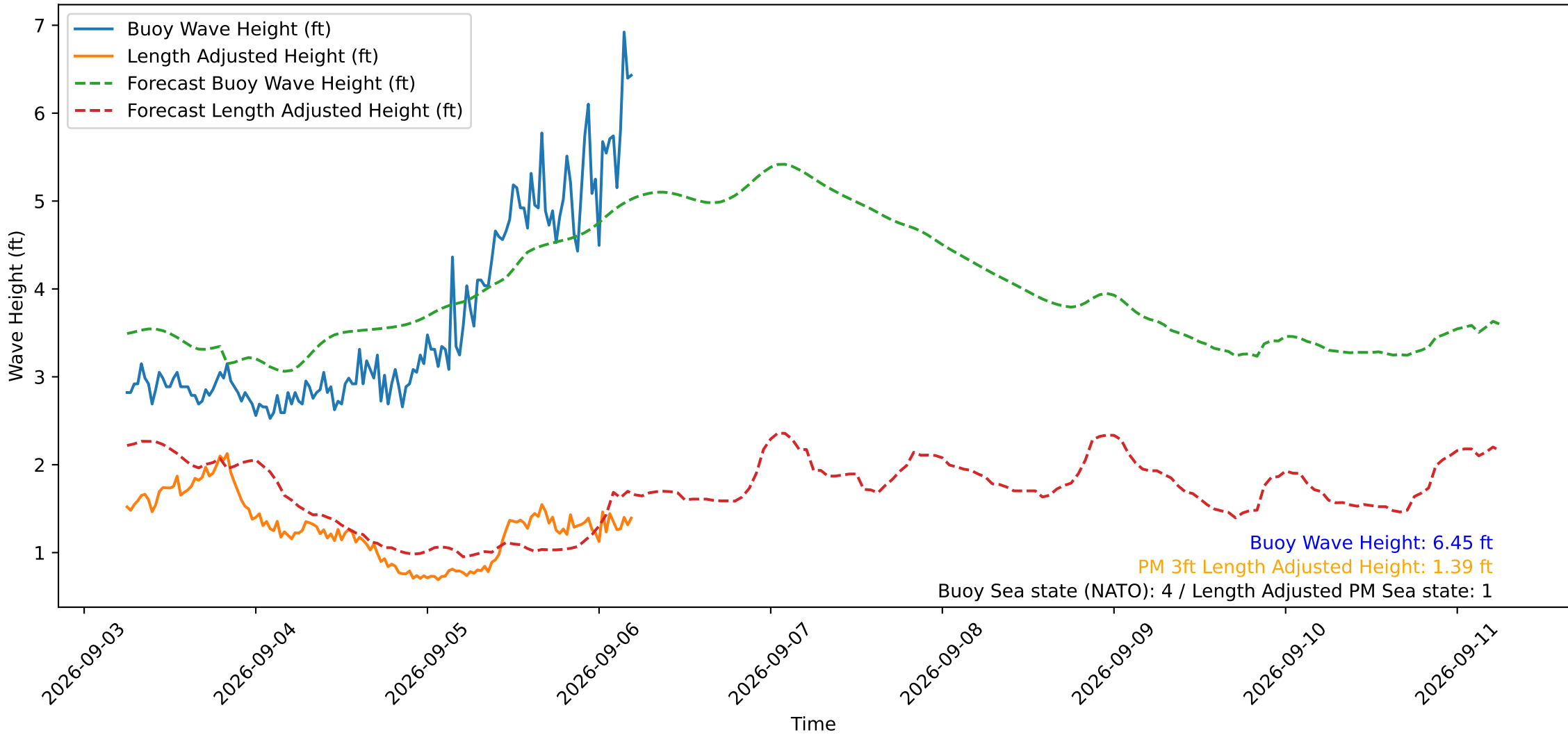
Wave Heights over Time for Red Beach at 2026-09-06 05:30:49
