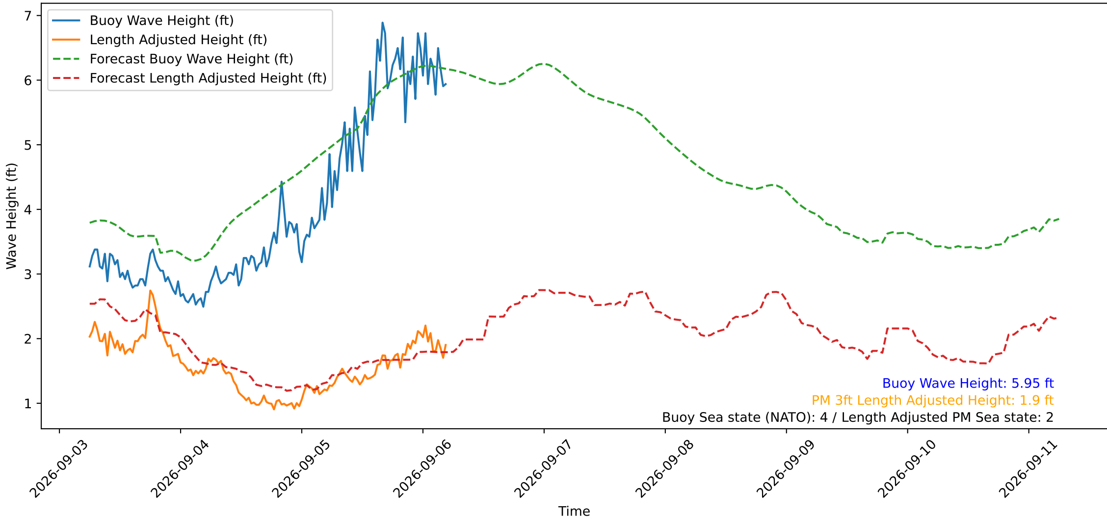
Wave Heights over Time for Green Beach at 2026-09-06 05:31:12
