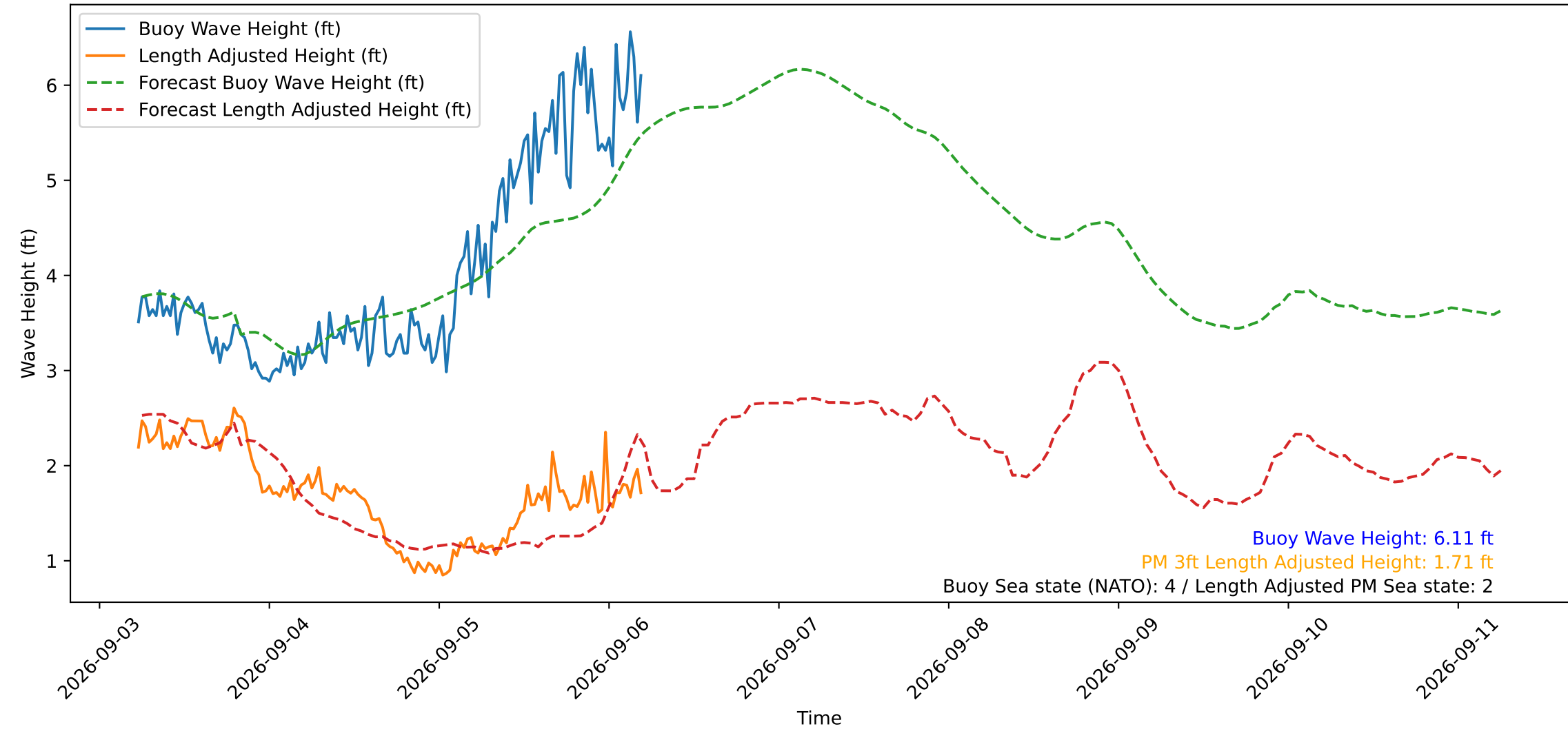
Wave Heights over Time for Oceanside Harbor at 2026-09-06 05:30:30
