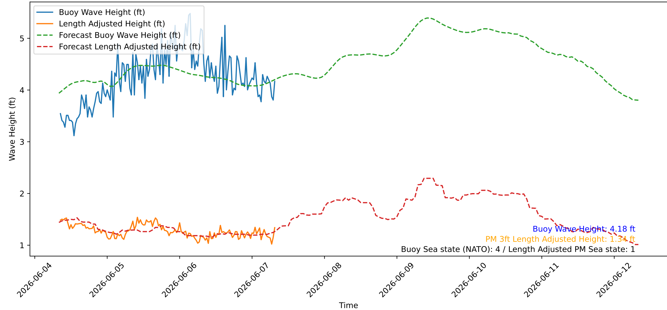
Wave Heights over Time for Oceanside Harbor at 2026-06-07 08:20:26
