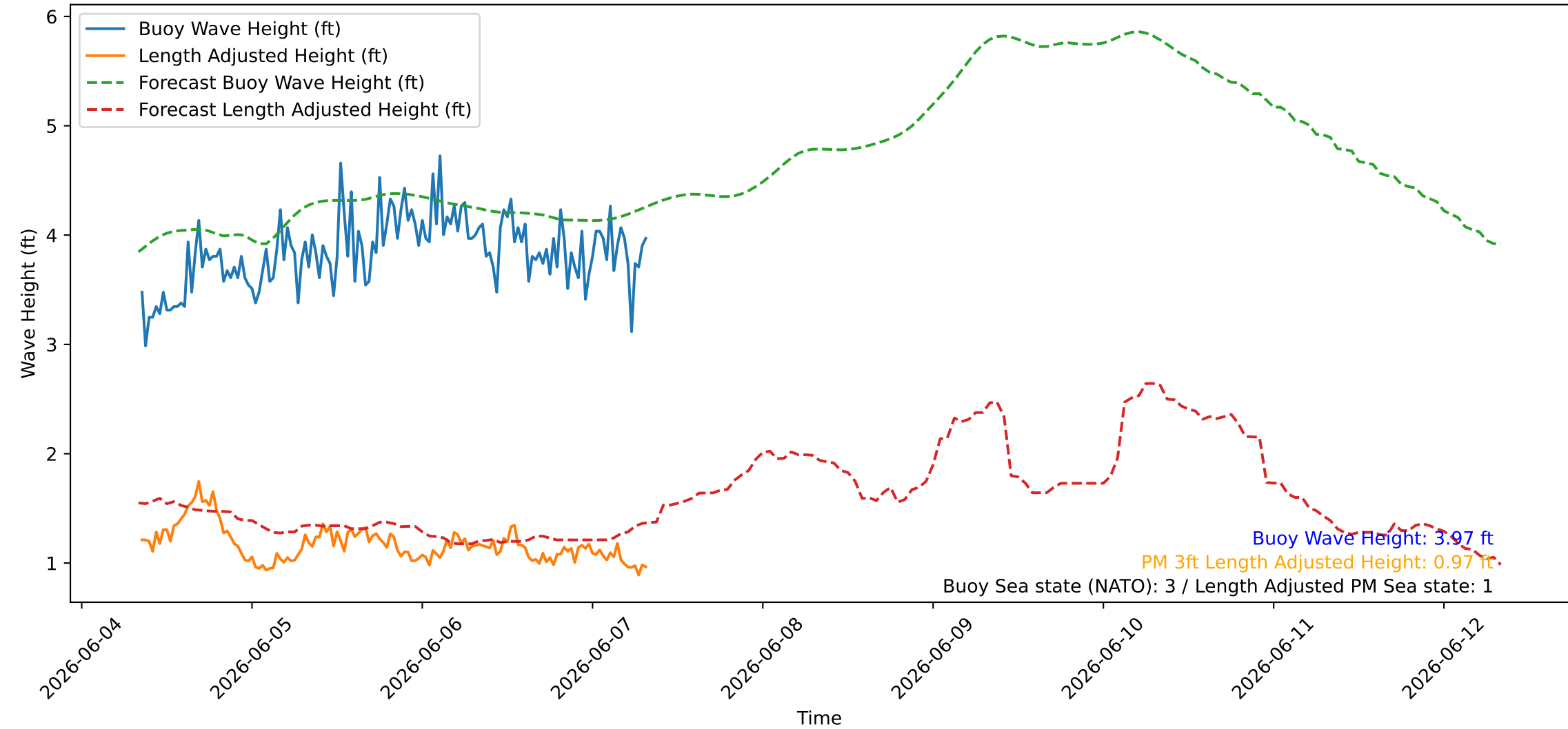
Wave Heights over Time for Green Beach at 2026-06-07 08:21:09
