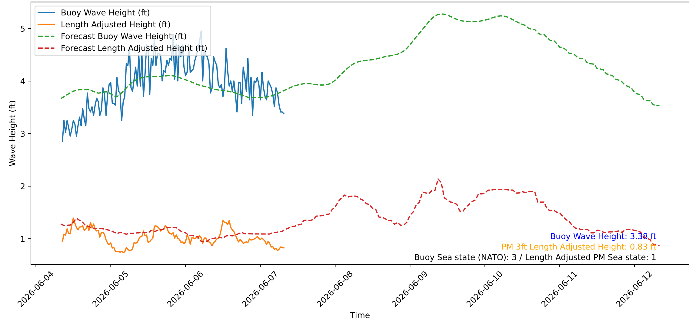
Wave Heights over Time for Red Beach at 2026-06-07 08:20:47
