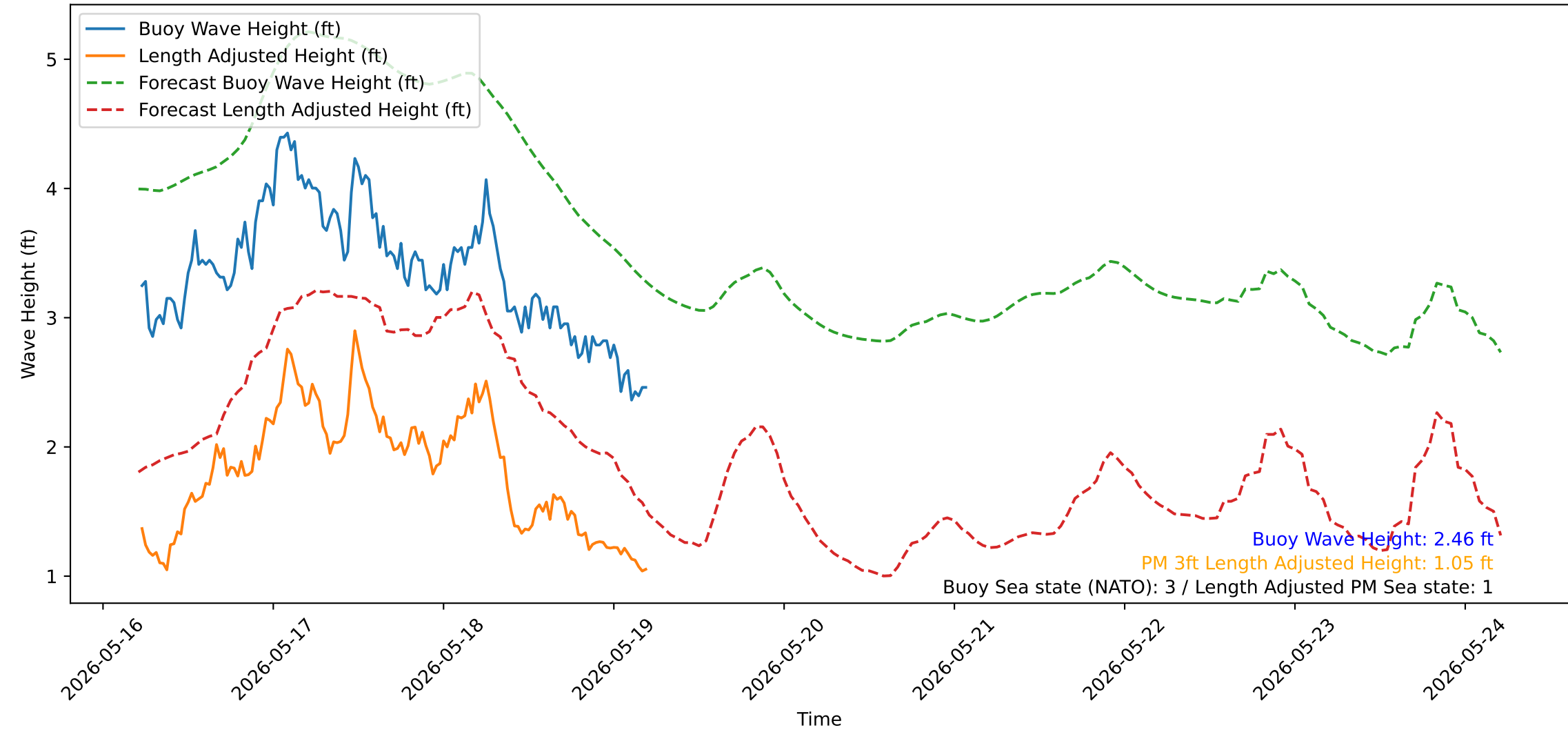
Wave Heights over Time for Green Beach at 2026-05-19 05:21:15
