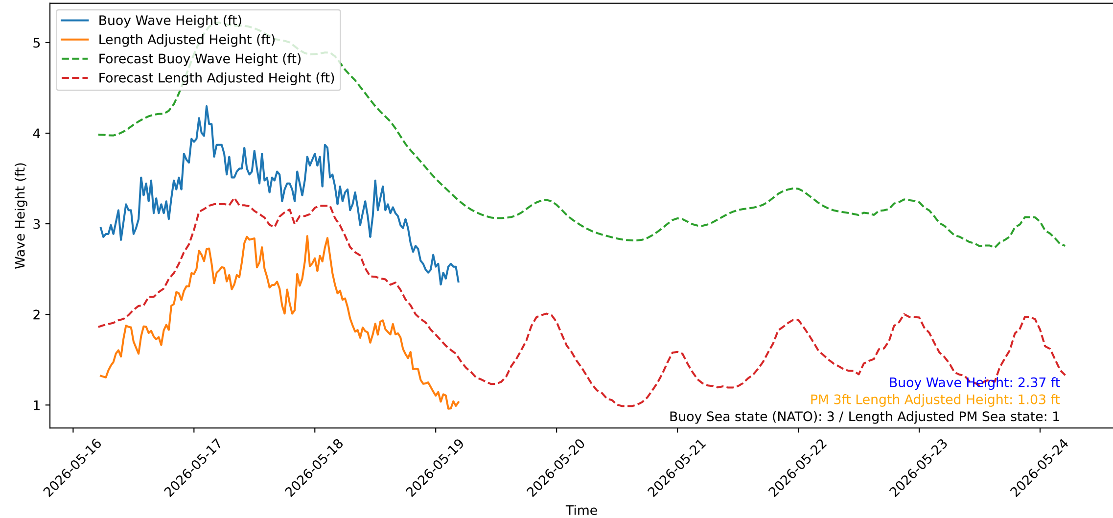
Wave Heights over Time for Oceanside Harbor at 2026-05-19 05:20:31
