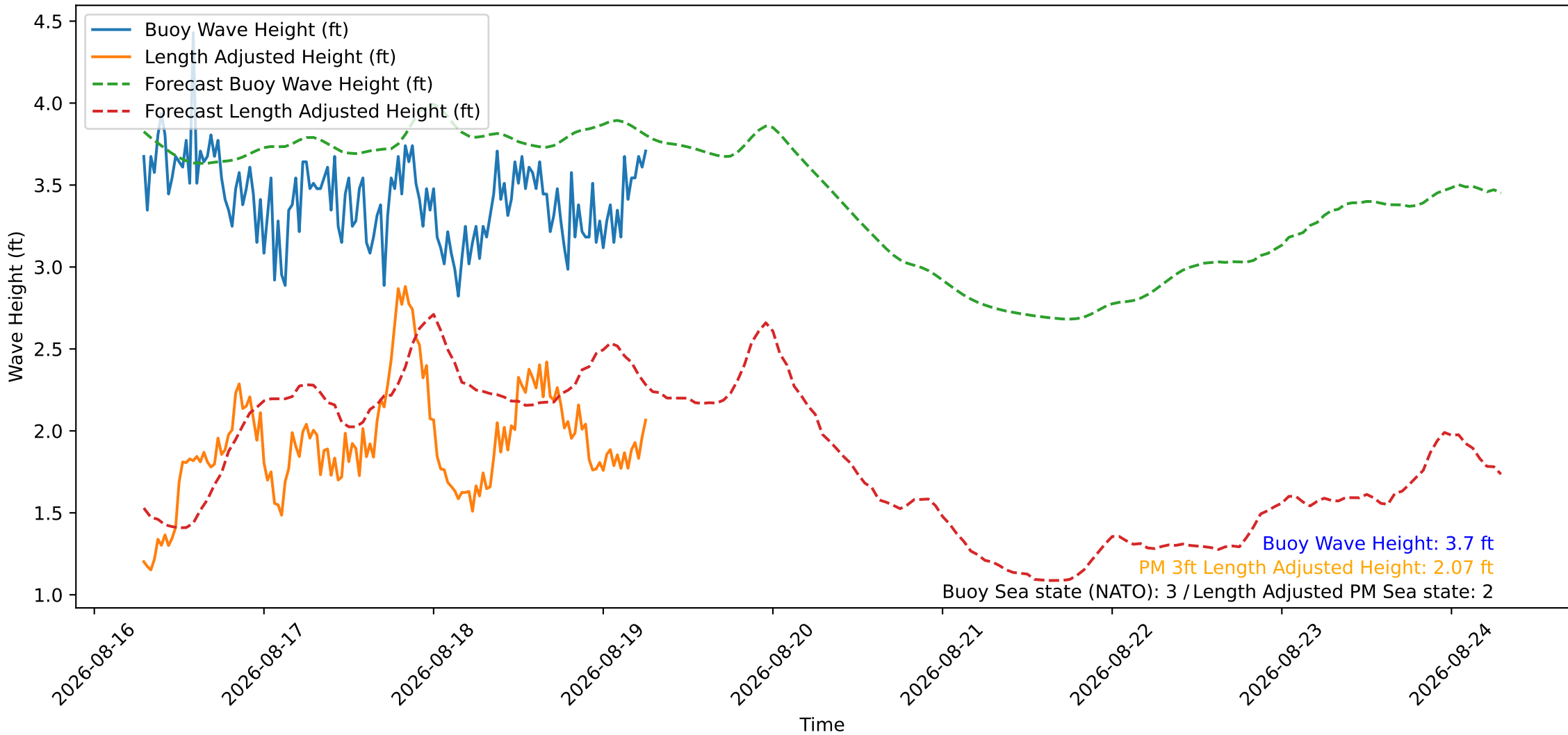
Wave Heights over Time for Oceanside Harbor at 2026-08-19 07:10:27
