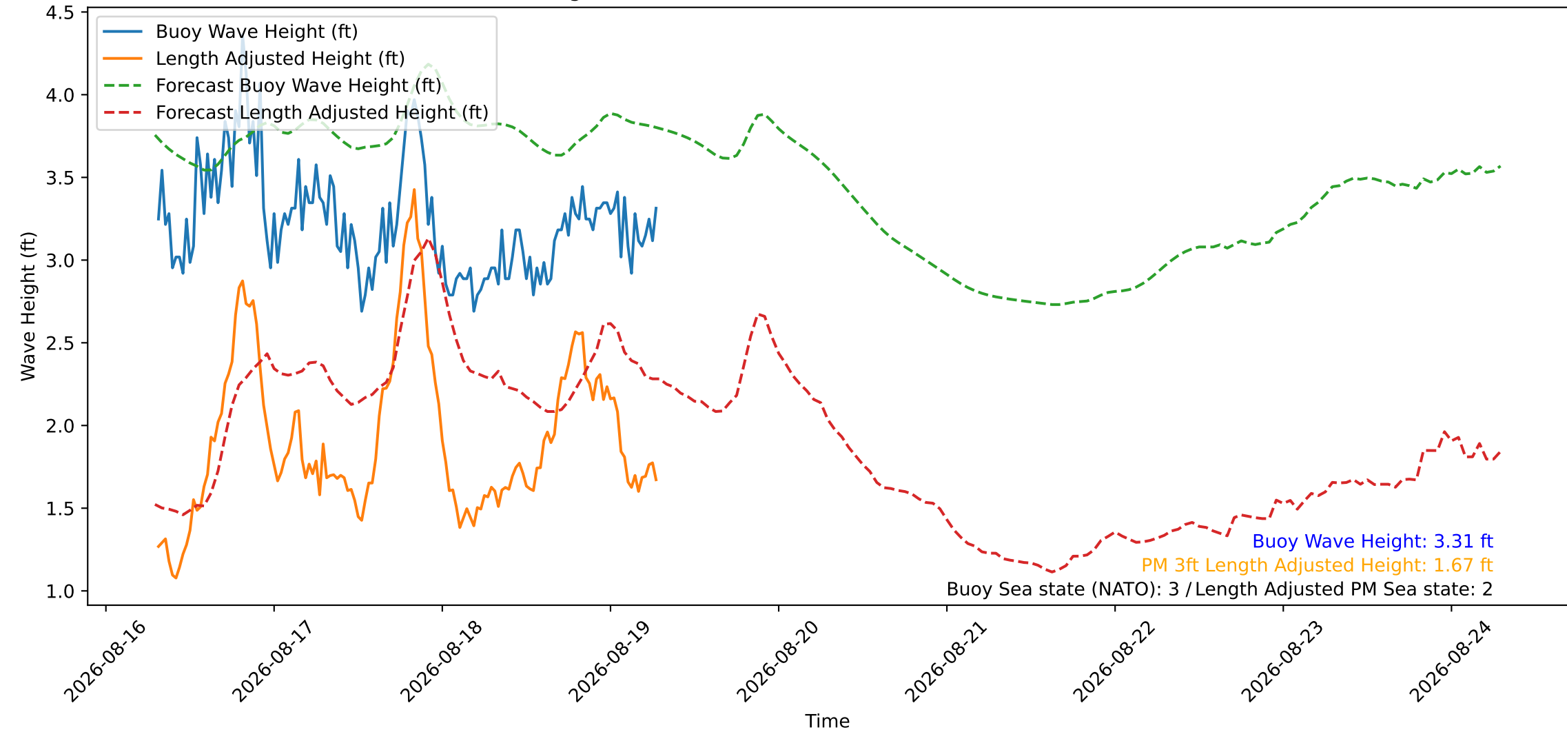
Wave Heights over Time for Green Beach at 2026-08-19 07:11:09
