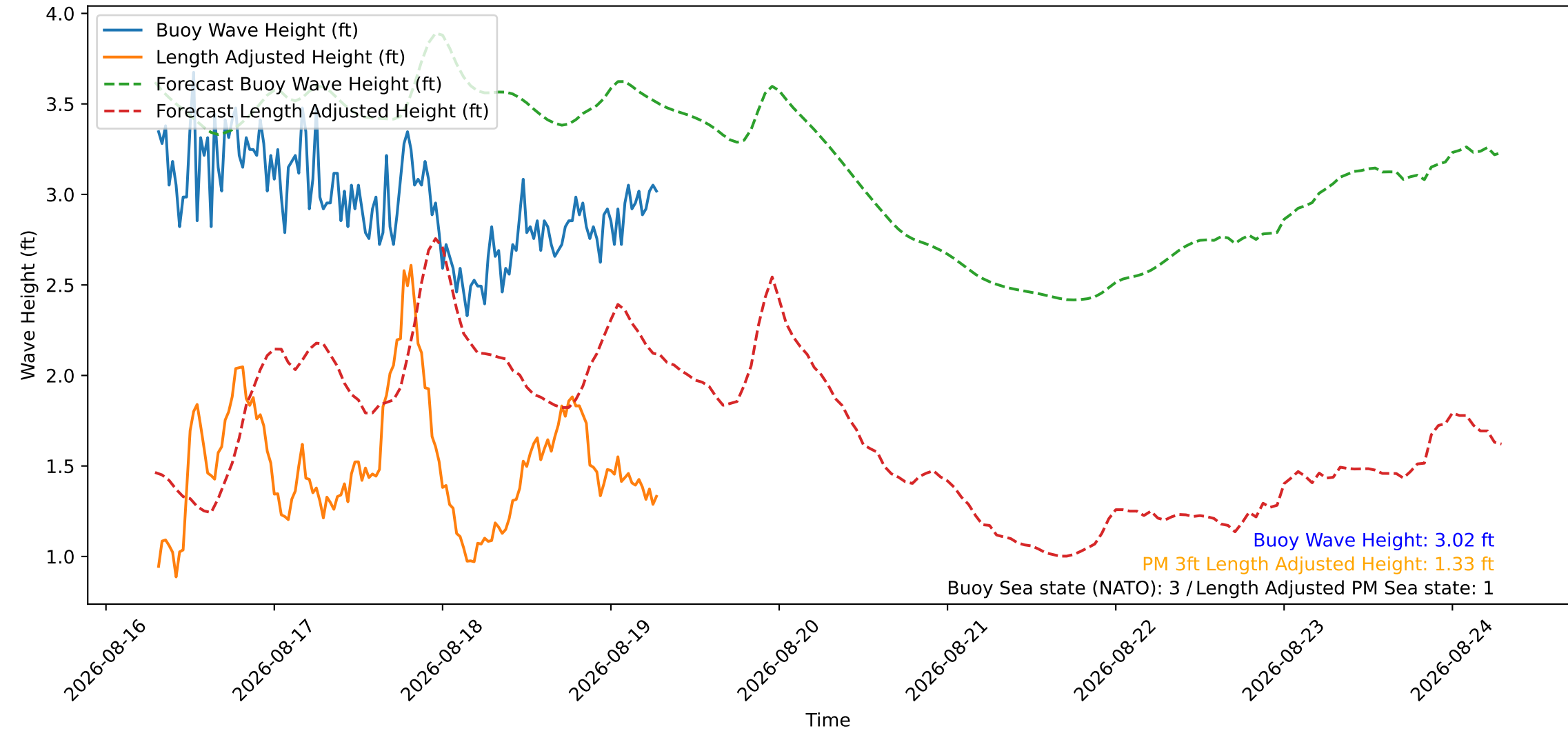
Wave Heights over Time for Red Beach at 2026-08-19 07:10:47
