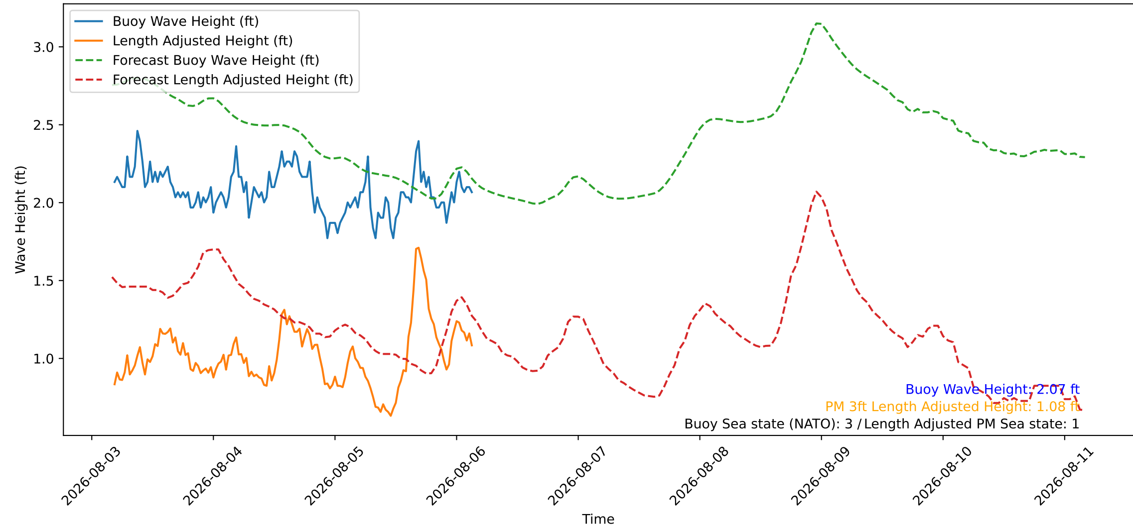
Wave Heights over Time for Red Beach at 2026-08-06 04:00:45
