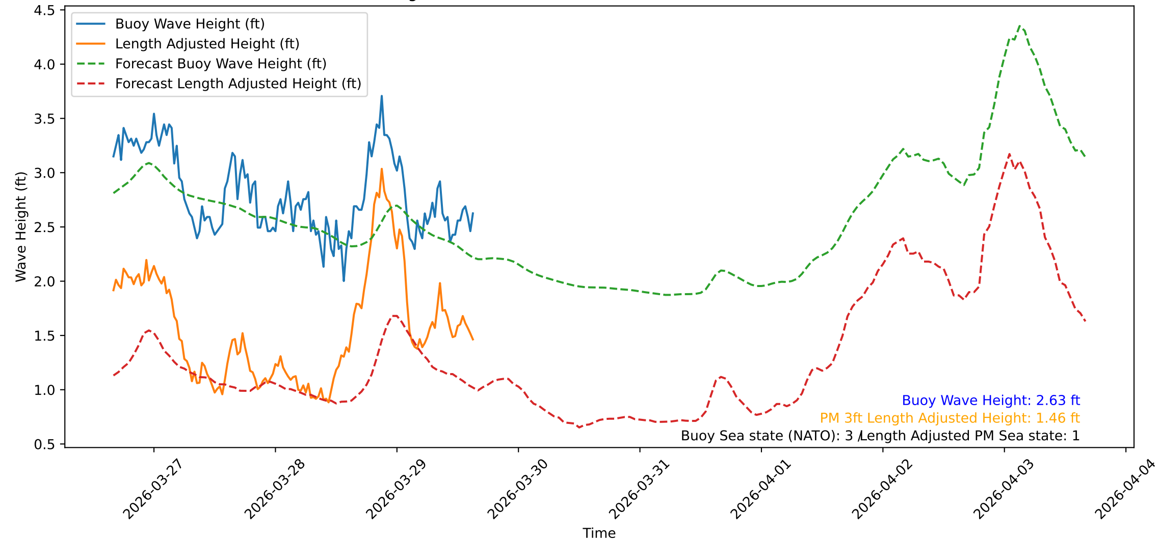
Wave Heights over Time for Green Beach at 2026-03-29 15:51:10
