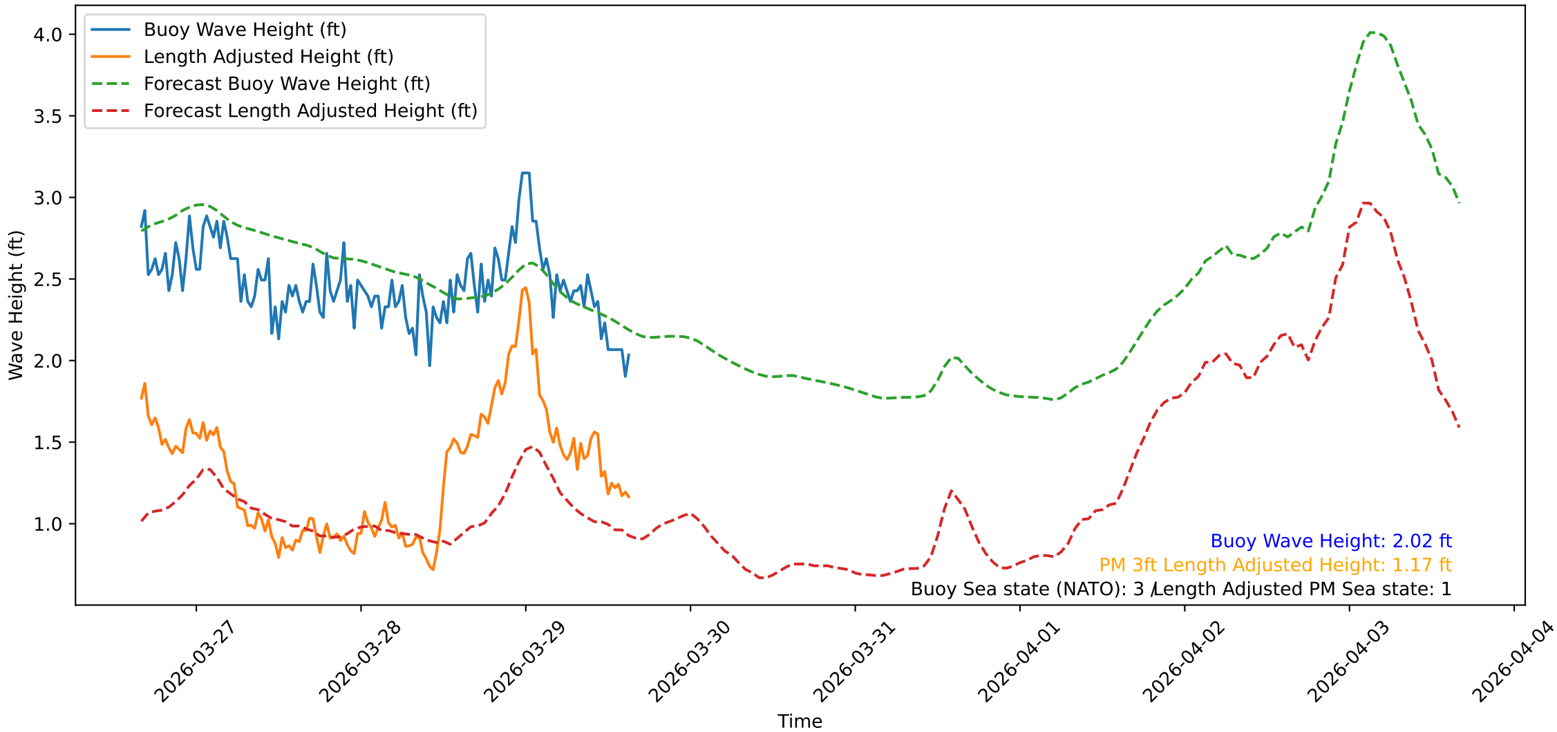
Wave Heights over Time for Oceanside Harbor at 2026-03-29 15:50:31
