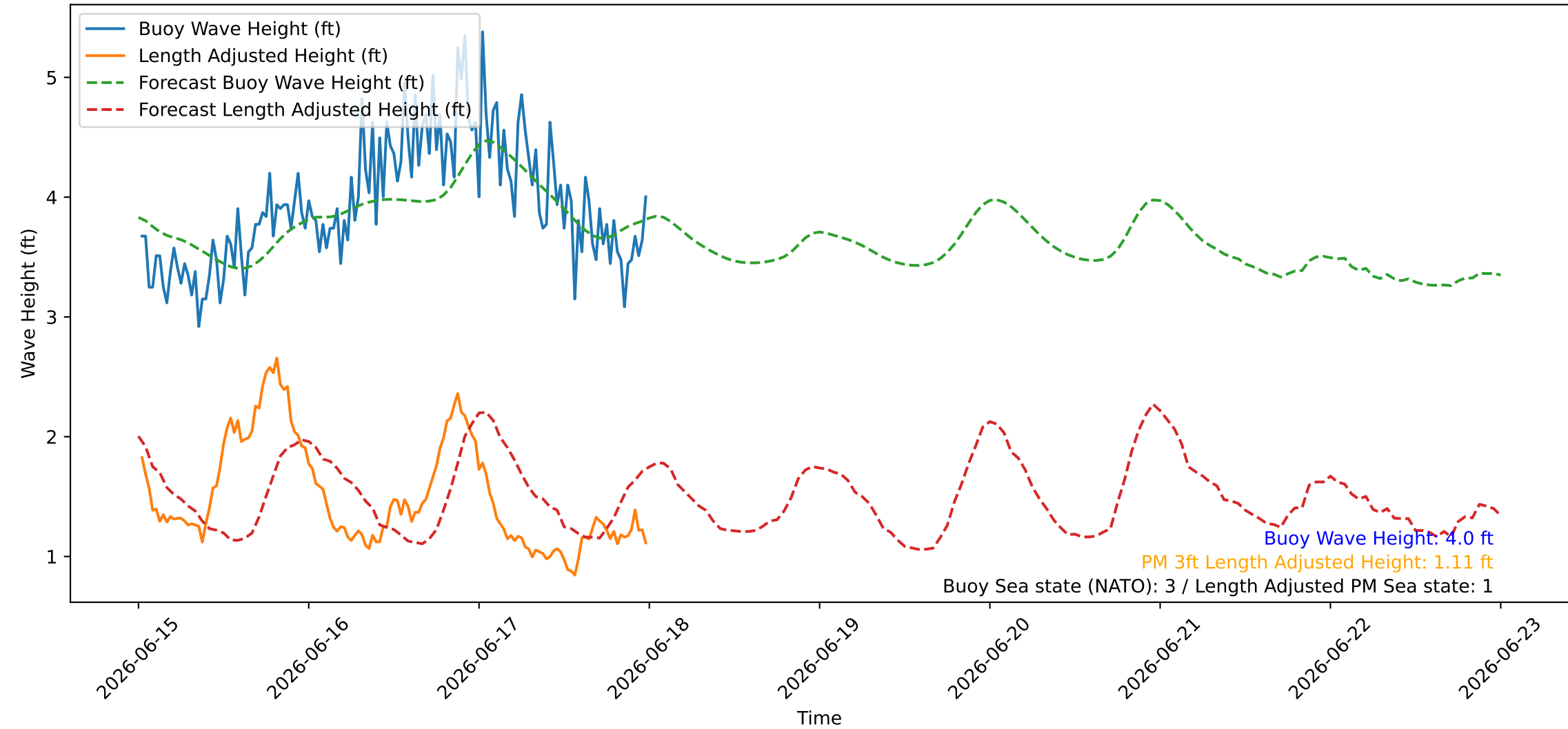
Wave Heights over Time for Red Beach at 2026-06-18 00:10:47
