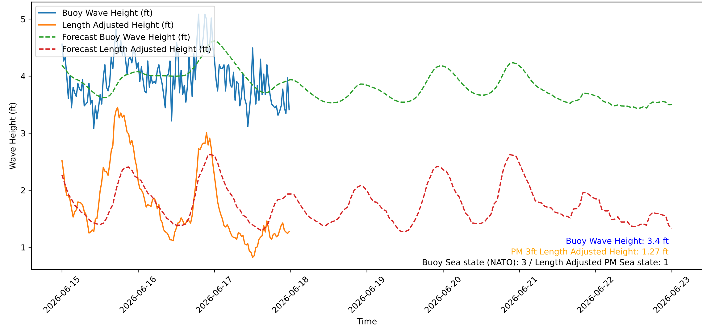
Wave Heights over Time for Green Beach at 2026-06-18 00:11:09
