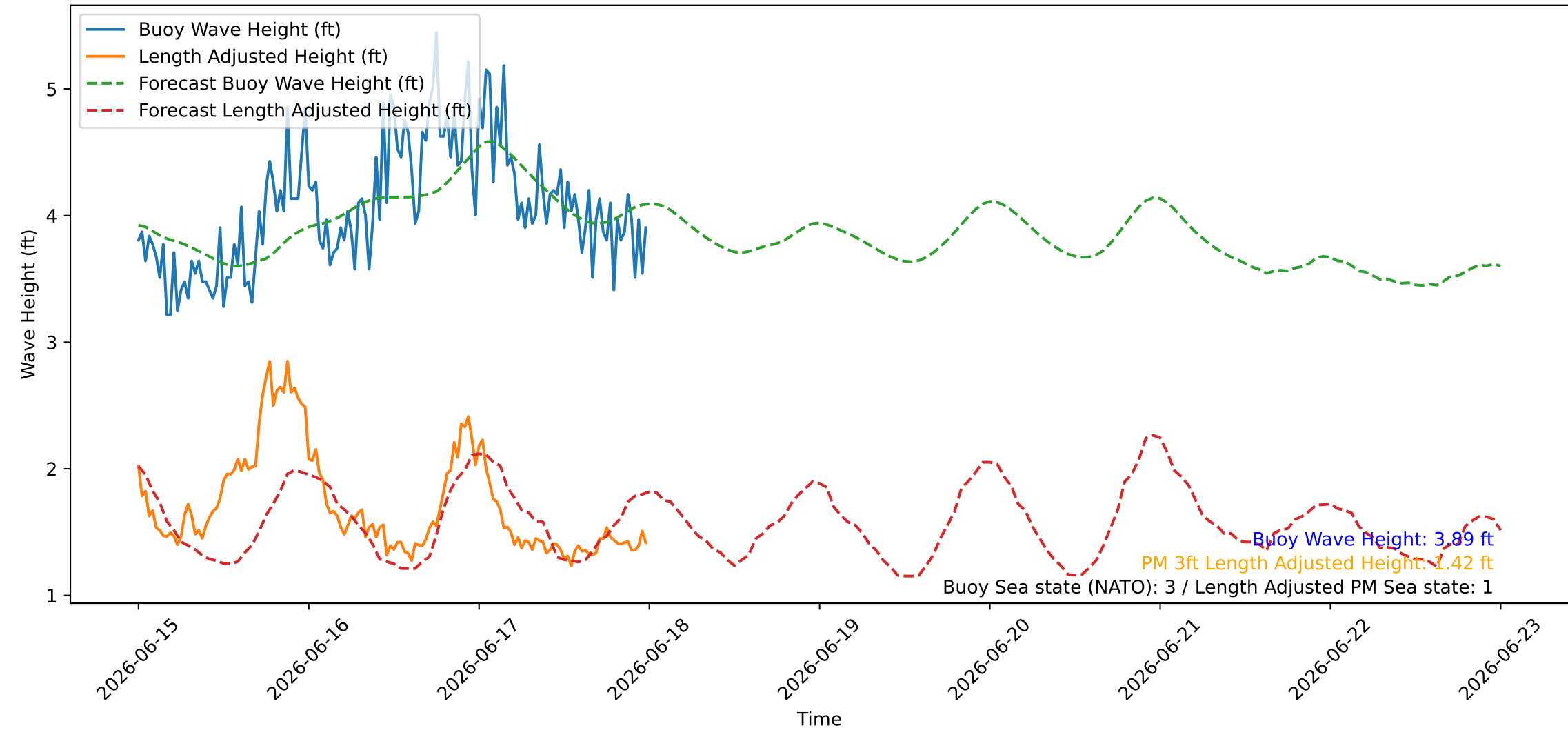
Wave Heights over Time for Oceanside Harbor at 2026-06-18 00:10:27
