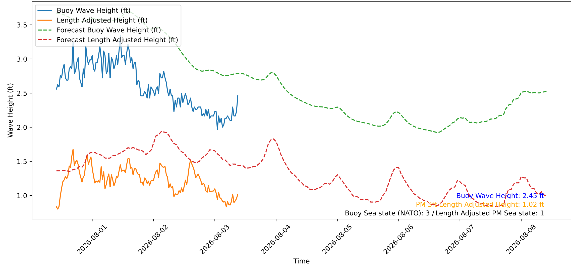
Wave Heights over Time for Red Beach at 2026-08-03 09:40:46
