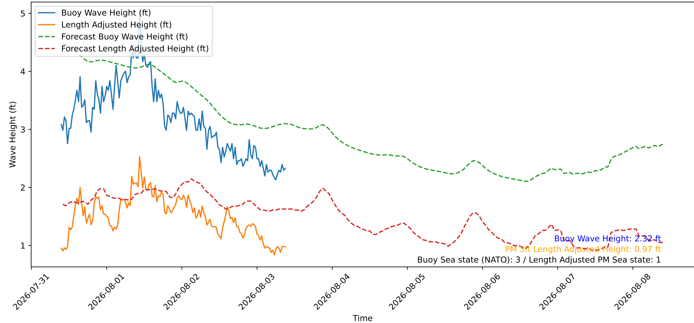
Wave Heights over Time for Green Beach at 2026-08-03 09:41:08
