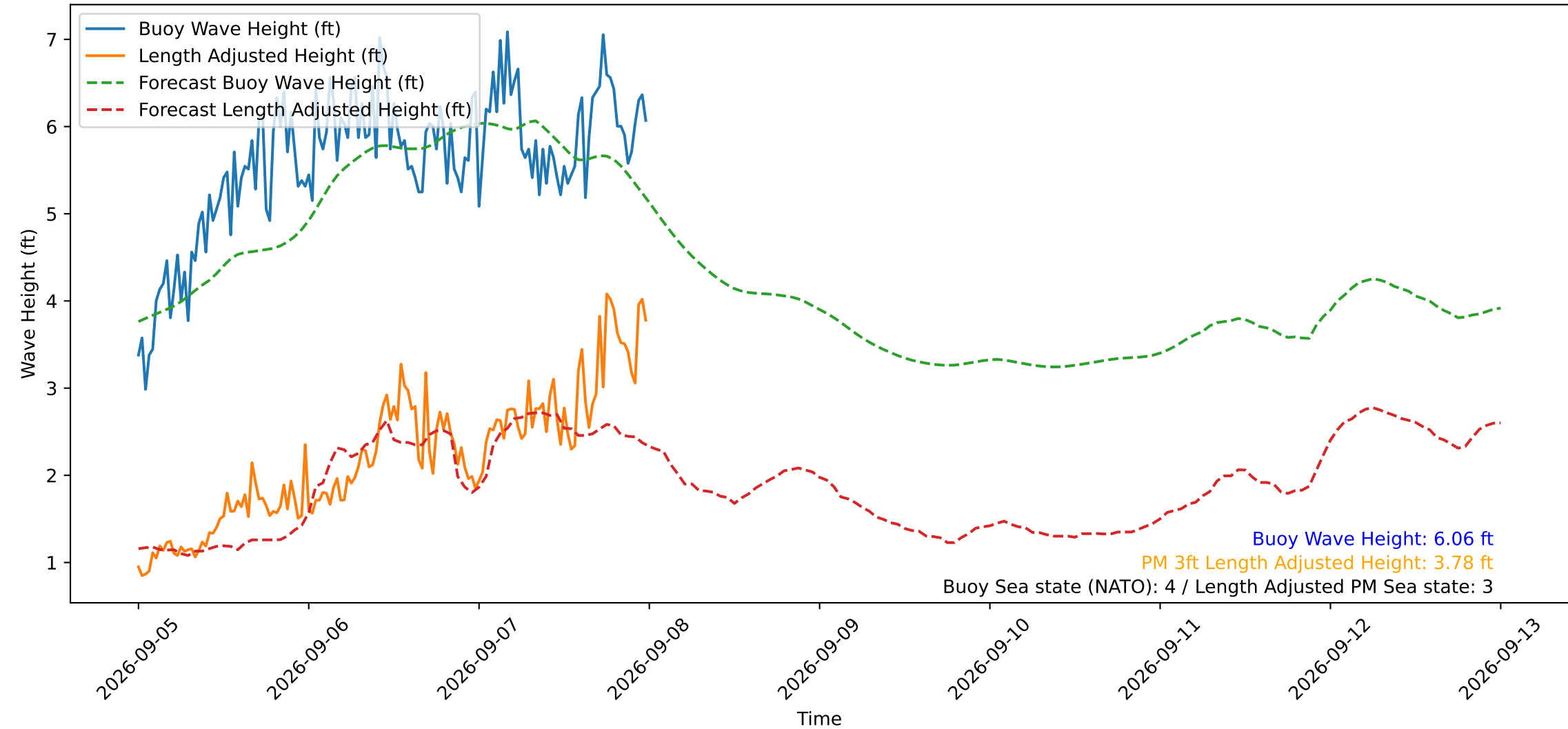
Wave Heights over Time for Oceanside Harbor at 2026-09-08 00:10:30
