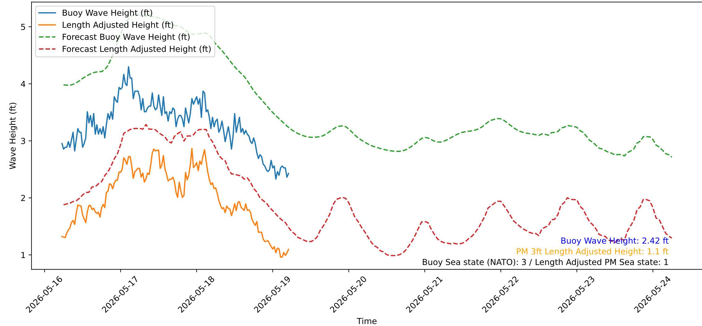
Wave Heights over Time for Oceanside Harbor at 2026-05-19 05:30:31
