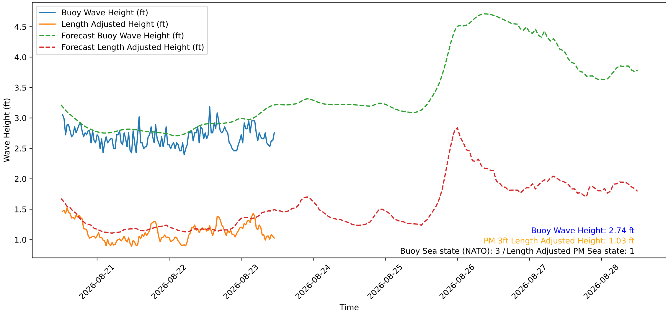
Wave Heights over Time for Green Beach at 2026-08-23 12:01:12
