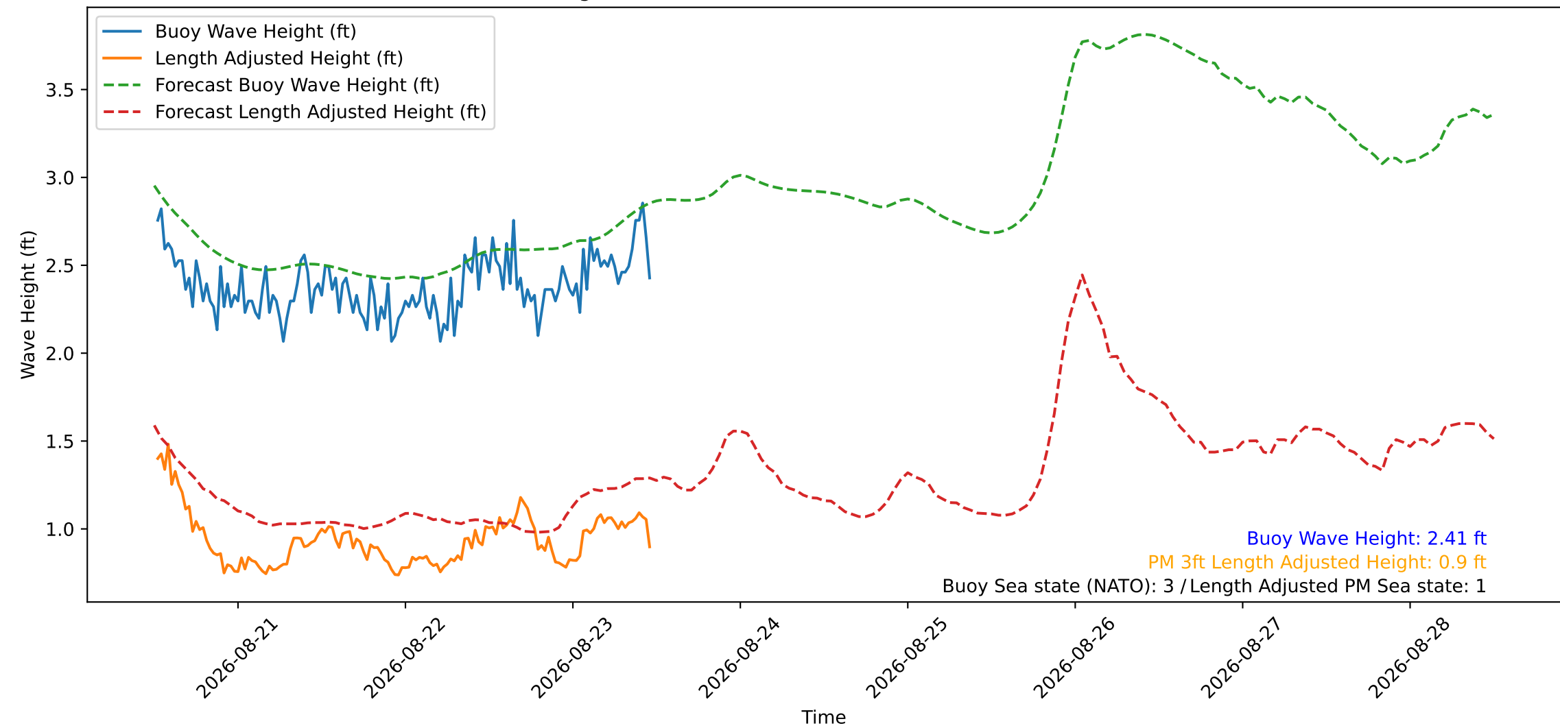
Wave Heights over Time for Red Beach at 2026-08-23 12:00:50
