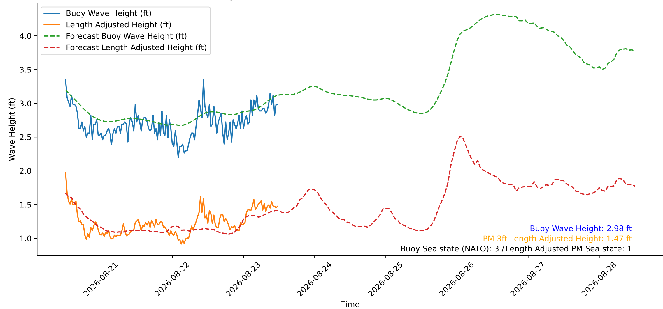
Wave Heights over Time for Oceanside Harbor at 2026-08-23 12:00:30
