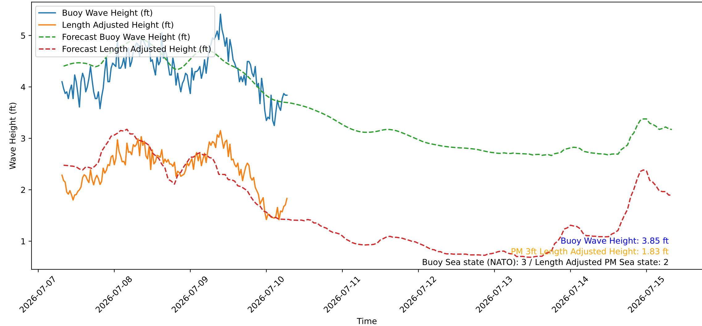
Wave Heights over Time for Oceanside Harbor at 2026-07-10 07:30:26
