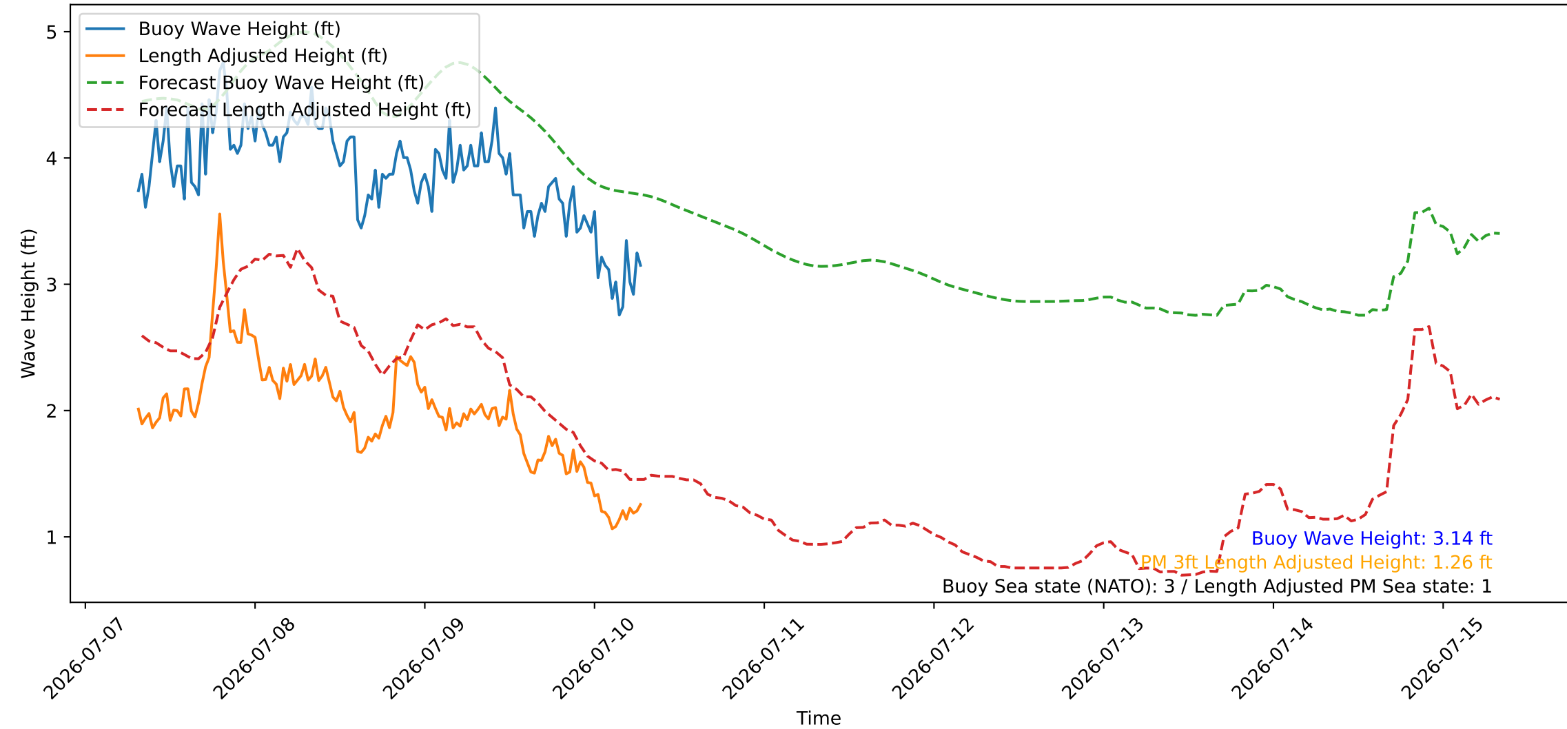
Wave Heights over Time for Green Beach at 2026-07-10 07:31:08
